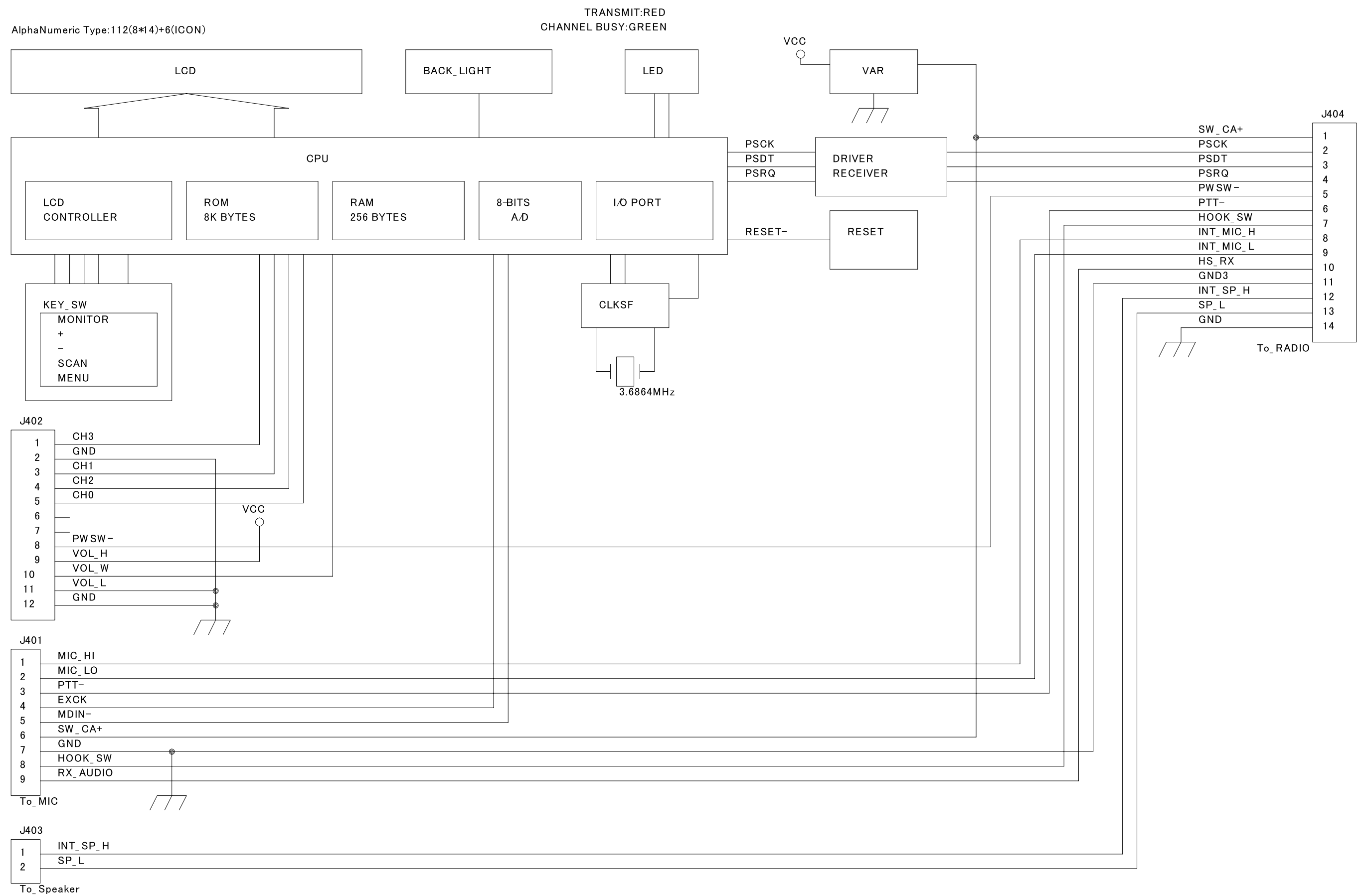
LCD Board Unit Block Diagram MA00-TC-0085 1/1
