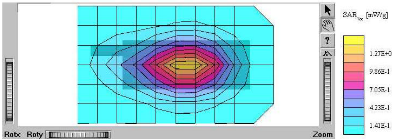
Distribution of maximum SAR in 800 AMPS band using BKB 193 123.
