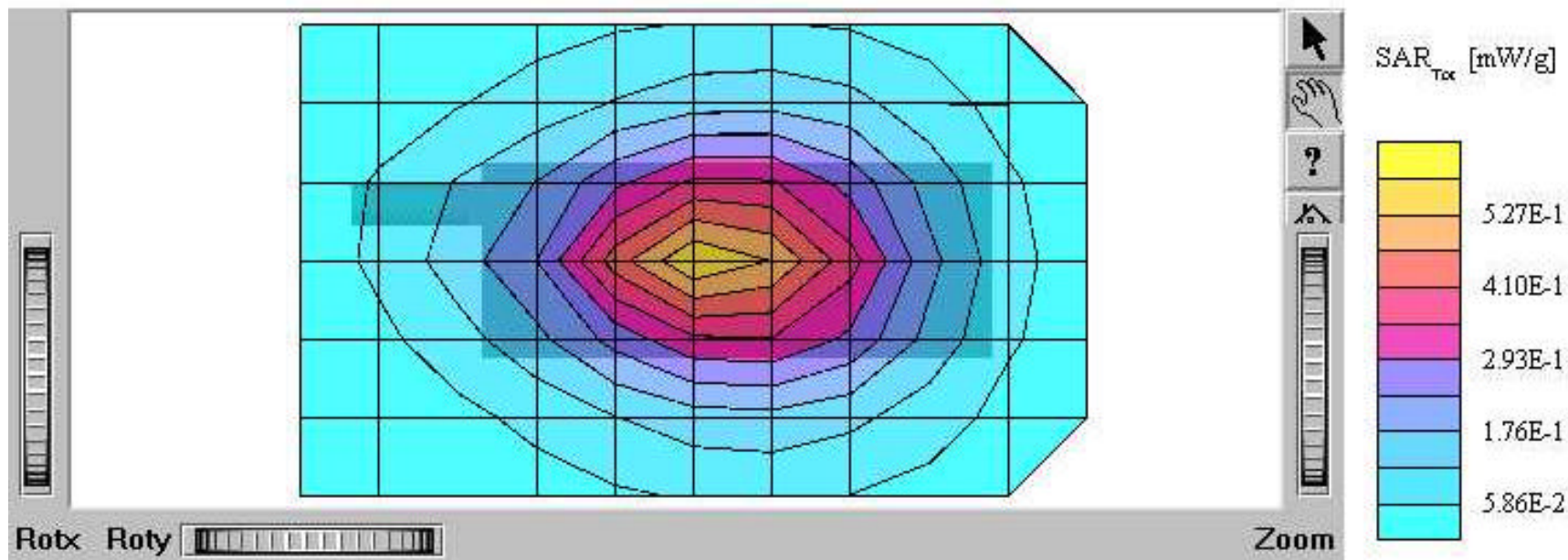
Distribution of maximum SAR in 800 AMPS band using KRY 104 1292 + SXK 107 6820.
