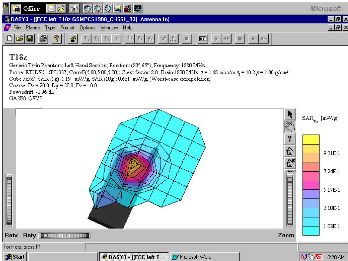
Distribution of worst-case SAR in PCS 1900 mode.
