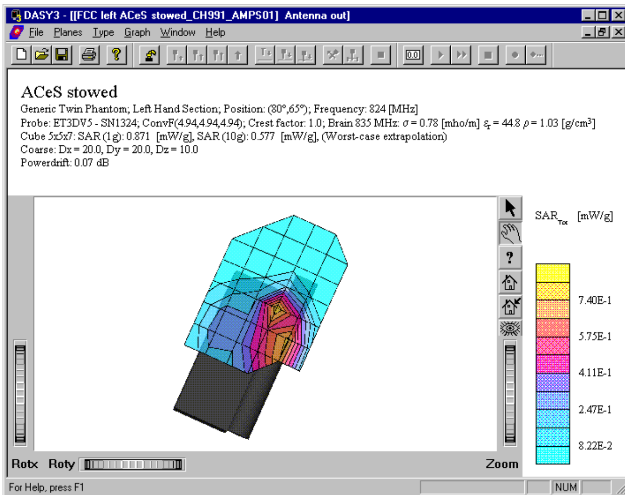
Distribution of worst-case SAR in AMPS mode.
