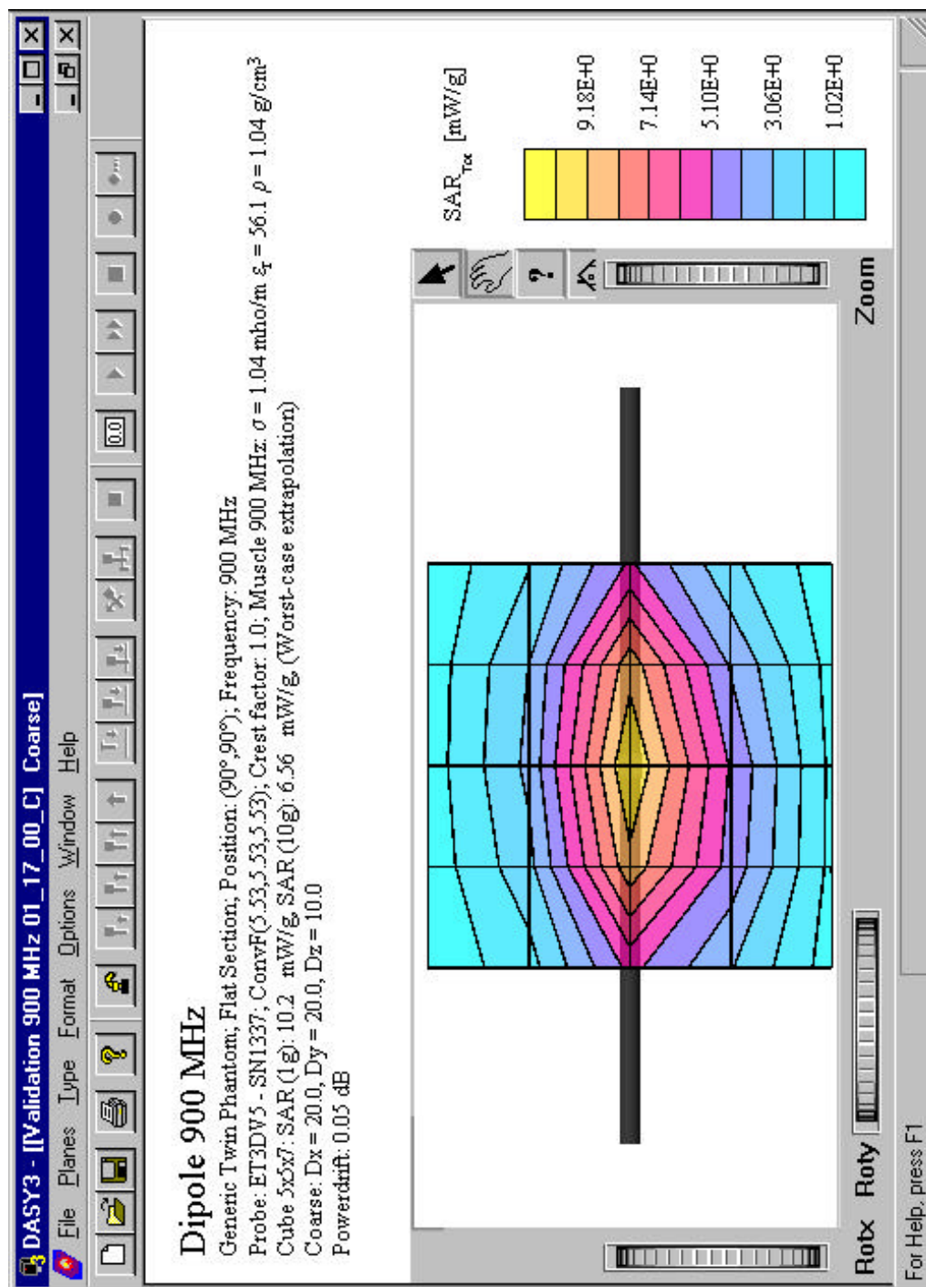
900 MHz SAR distribution of validation dipole antenna from system accuracy verification test.
