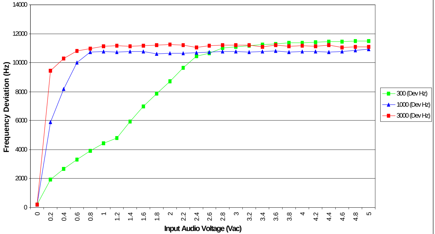
Modulation Limiting versus Input Signal
