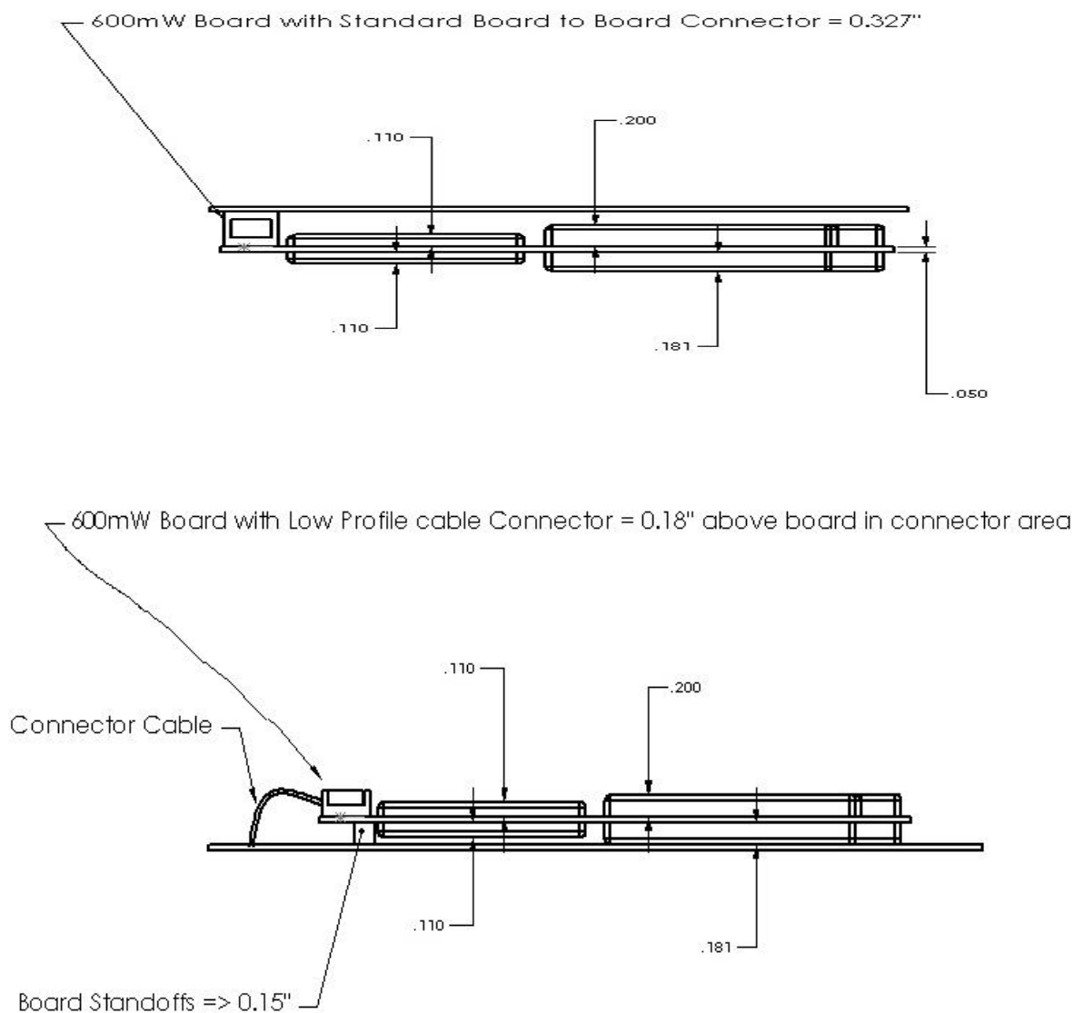
Figure 1.4-1 Module Mounting Configuration
