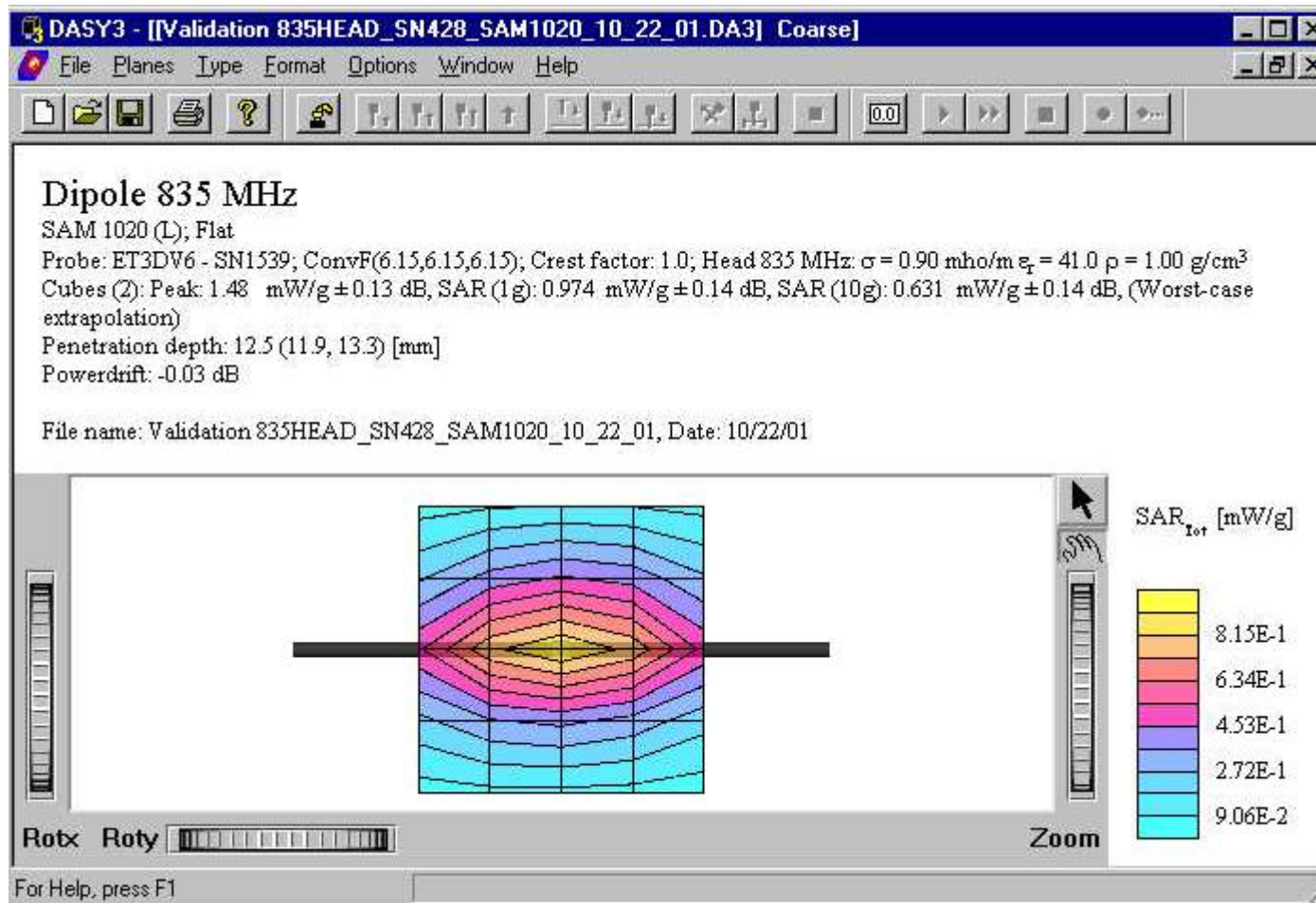
835 MHz SAR distribution of validation dipole antenna from system accuracy verification test on October 22, 2001. Using head tissue. Antenna input power = 98.7mW.
