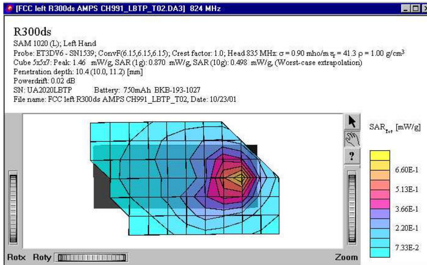
Distribution of maximum SAR in 800 AMPS band. Measured against the head in the "Tilt" position.
