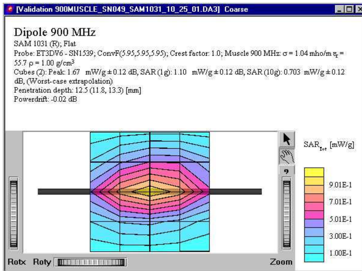
900 MHz SAR distribution of validation dipole antenna from system accuracy verification test on October 25, 2001. Using muscle tissue. Antenna input power = 99.4 mW.
