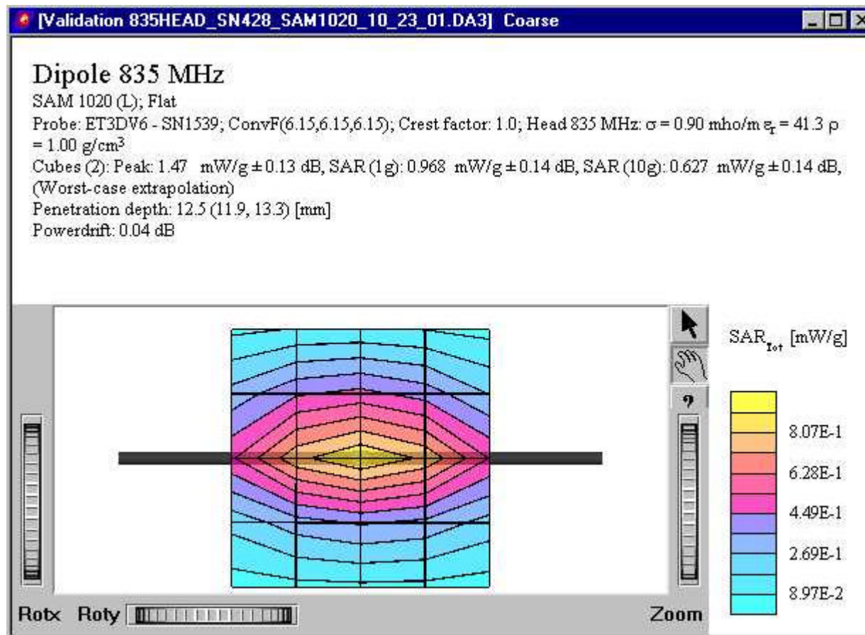
835 MHz SAR distribution of validation dipole antenna from system accuracy verification test on October 23, 2001. Using head tissue. Antenna input power = 99.2 mW.
