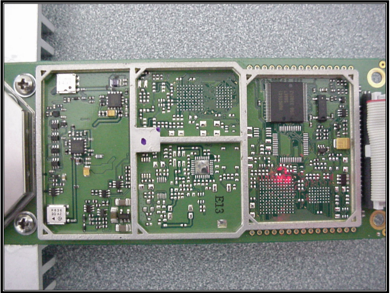
PHOTOGRAPH 5: FRONT VIEW OF MODULE (1)
