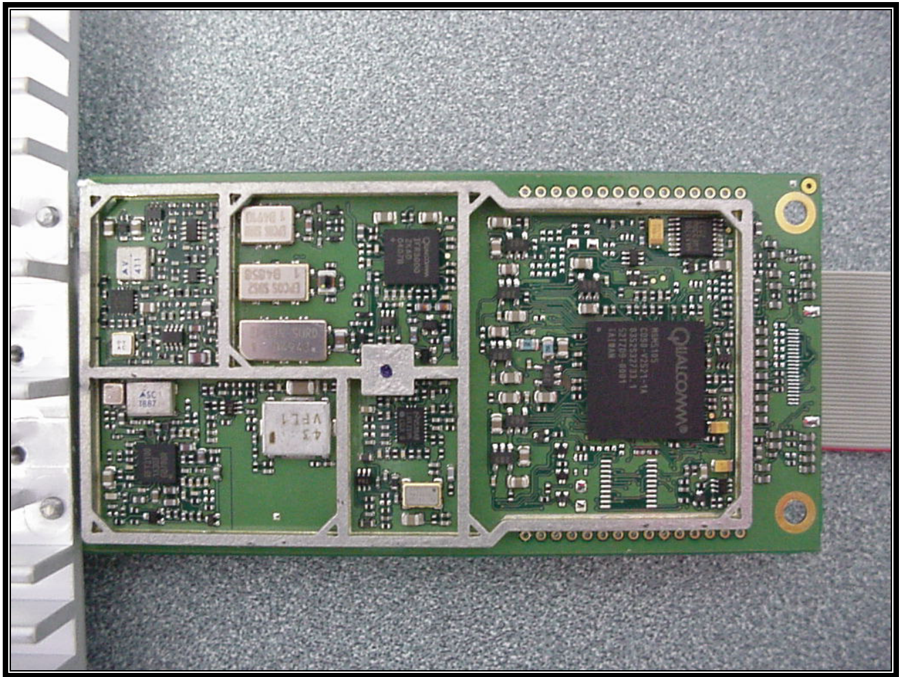
PHOTOGRAPH 7: BACK VIEW OF MODULE
