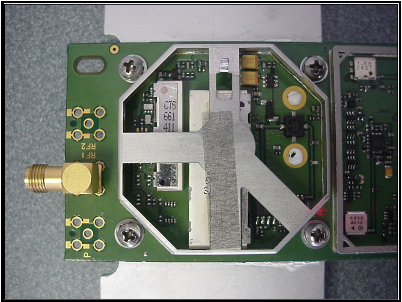
PHOTOGRAPH 6: FRONT VIEW OF MODULE (2)
