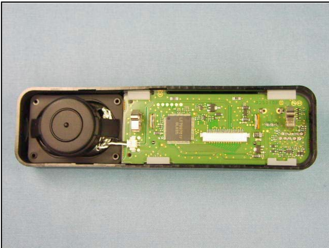
Inside of FRONT panel with Unit and SP (EVX-5400)
