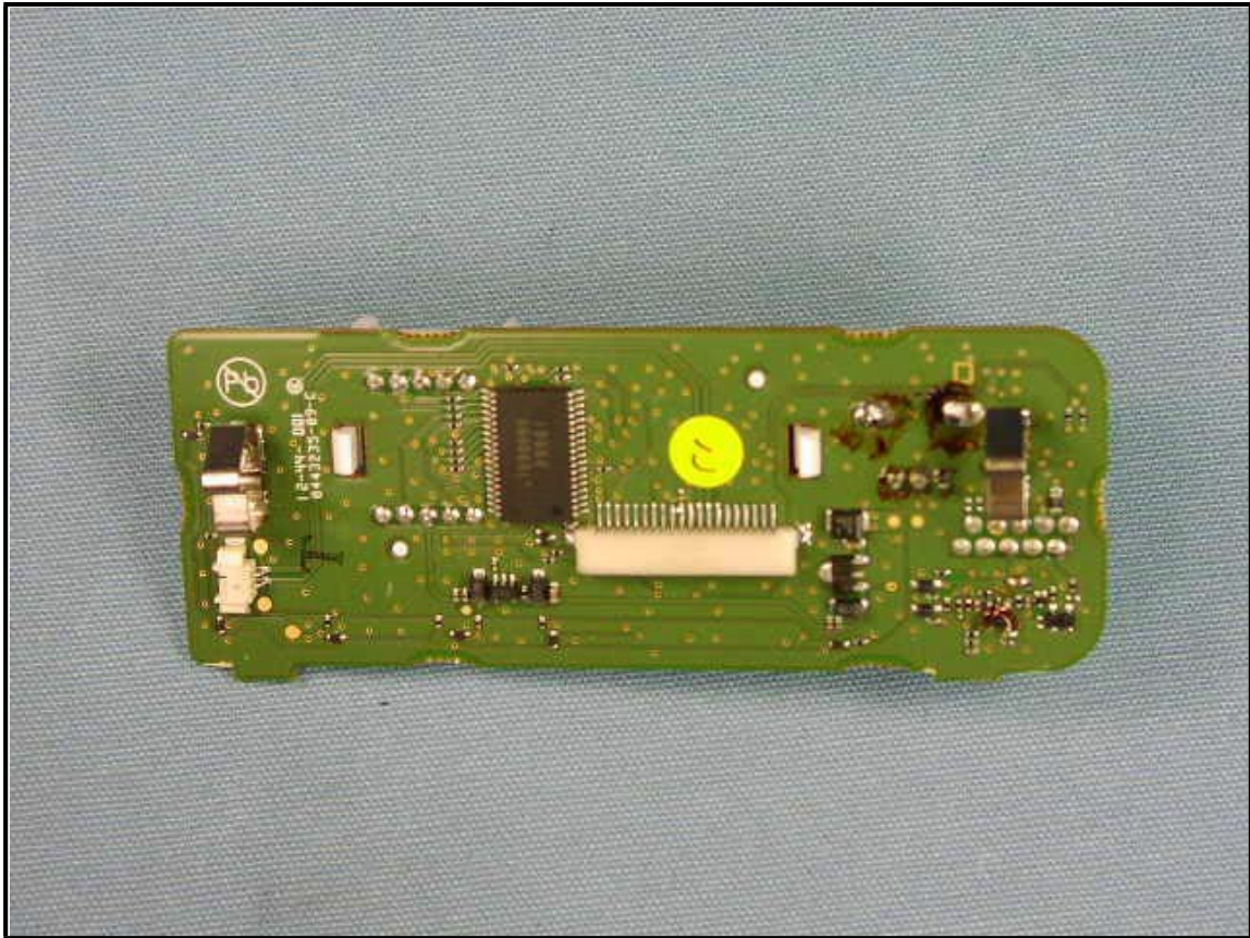
Side-B of FRONT-Unit (EVX-5300)
