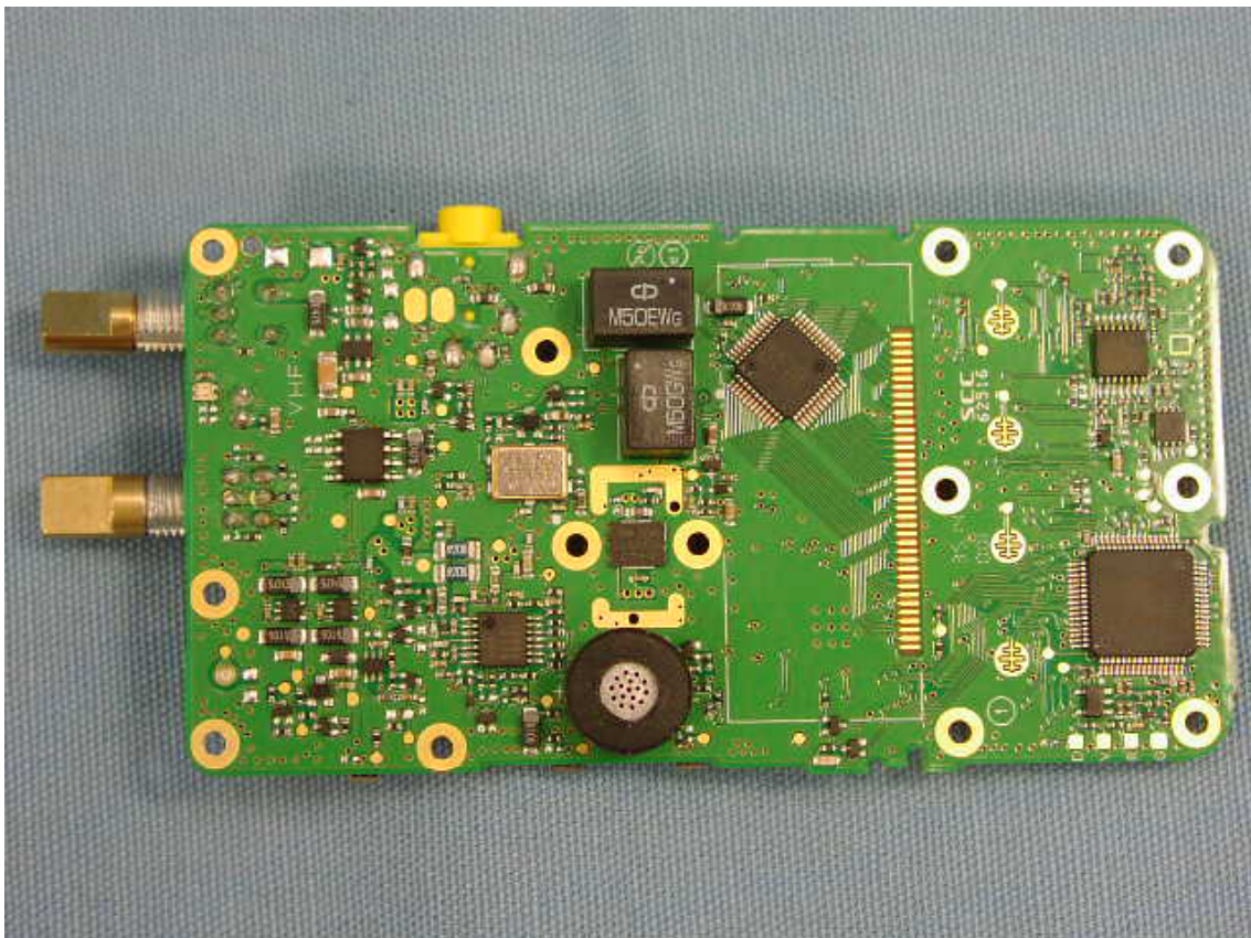
Side-A of MAIN-UNIT without LCD and Shield
