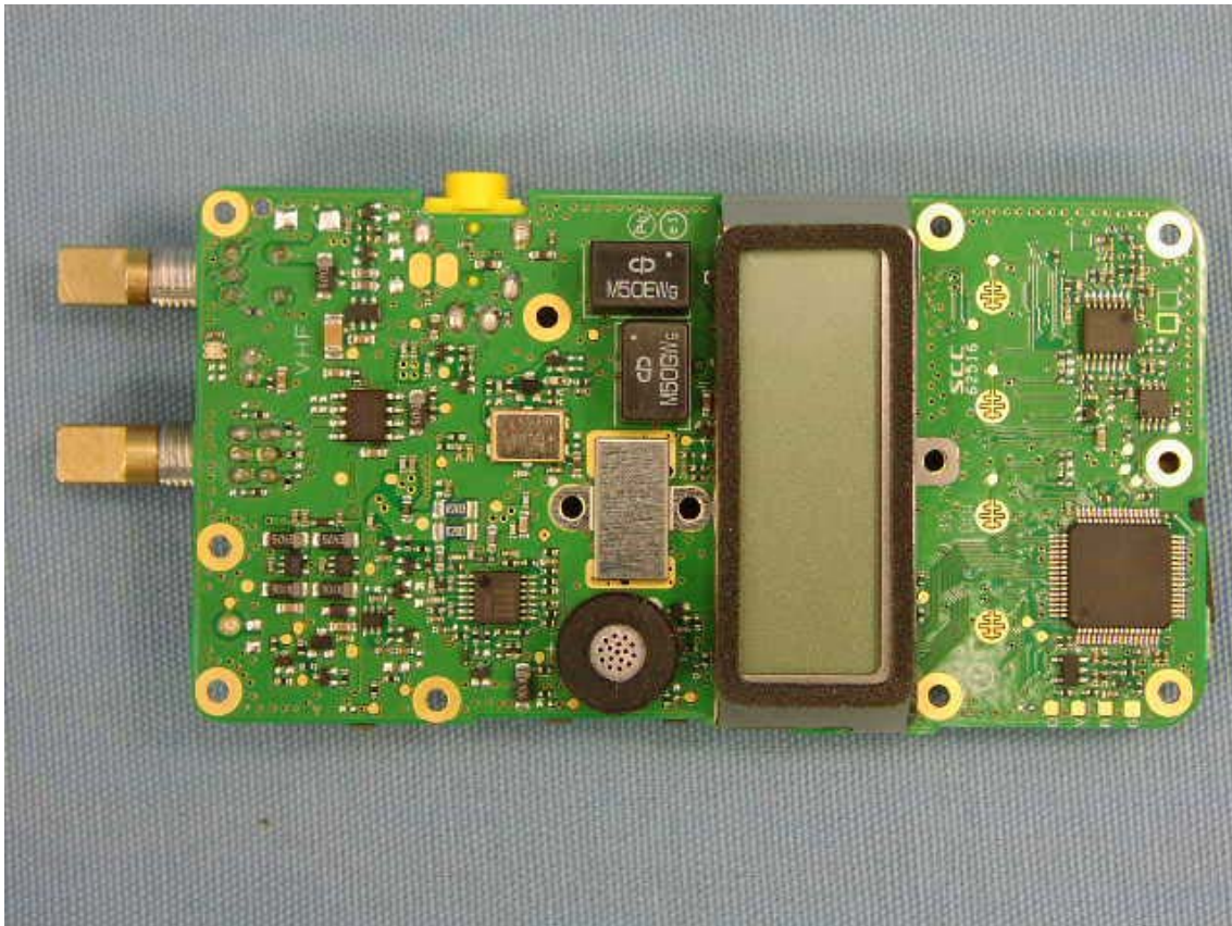
Side-A of MAIN-UNIT with LCD and Shield
