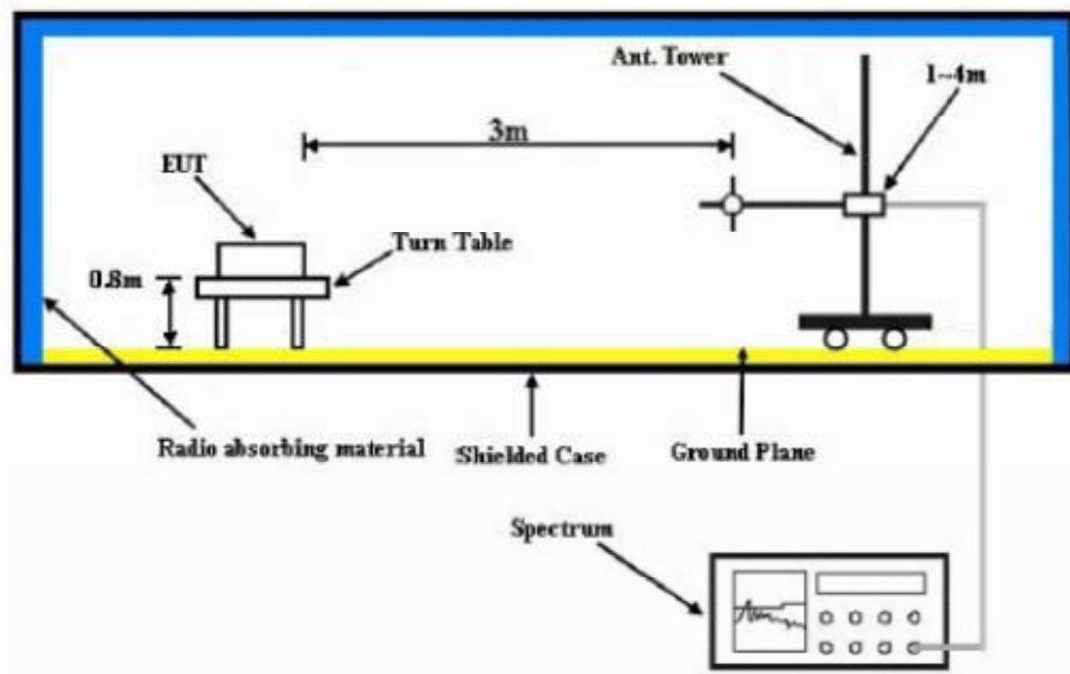
Radiated test setup drawing
