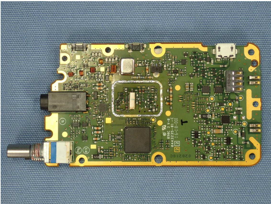
Side-B of MAIN-UNIT without Shield
