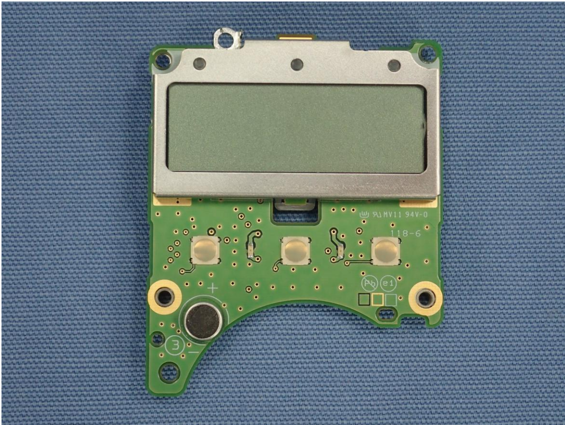
Side-A of Display-UNIT
