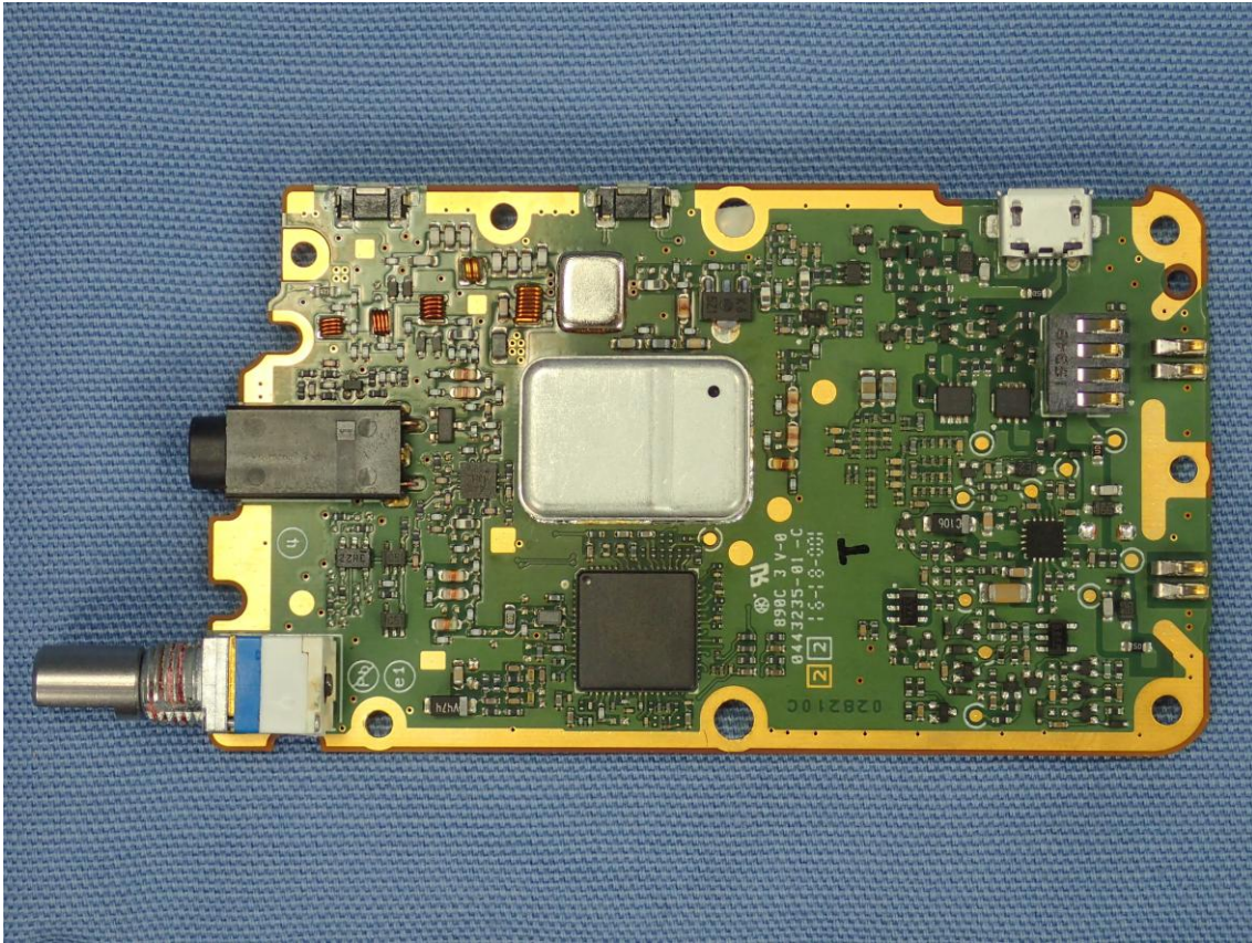
Side-B of MAIN-UNIT with Shield
