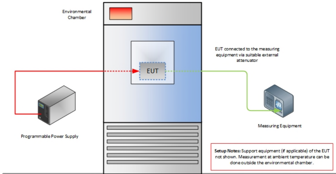
Transmission Spectrum Mask Test Configuration
