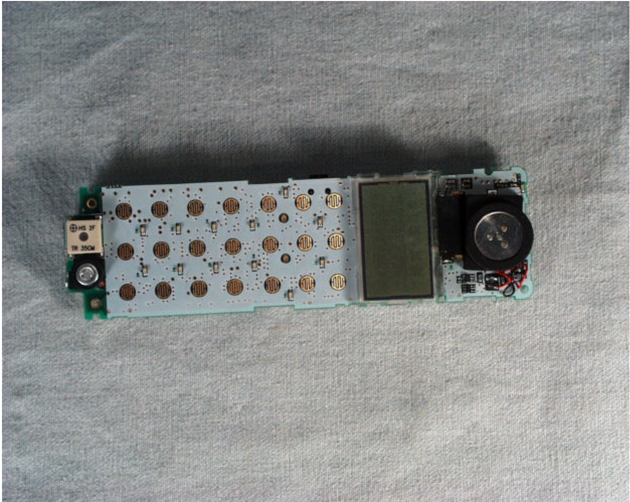
Side B (Keypad and LCD display)
