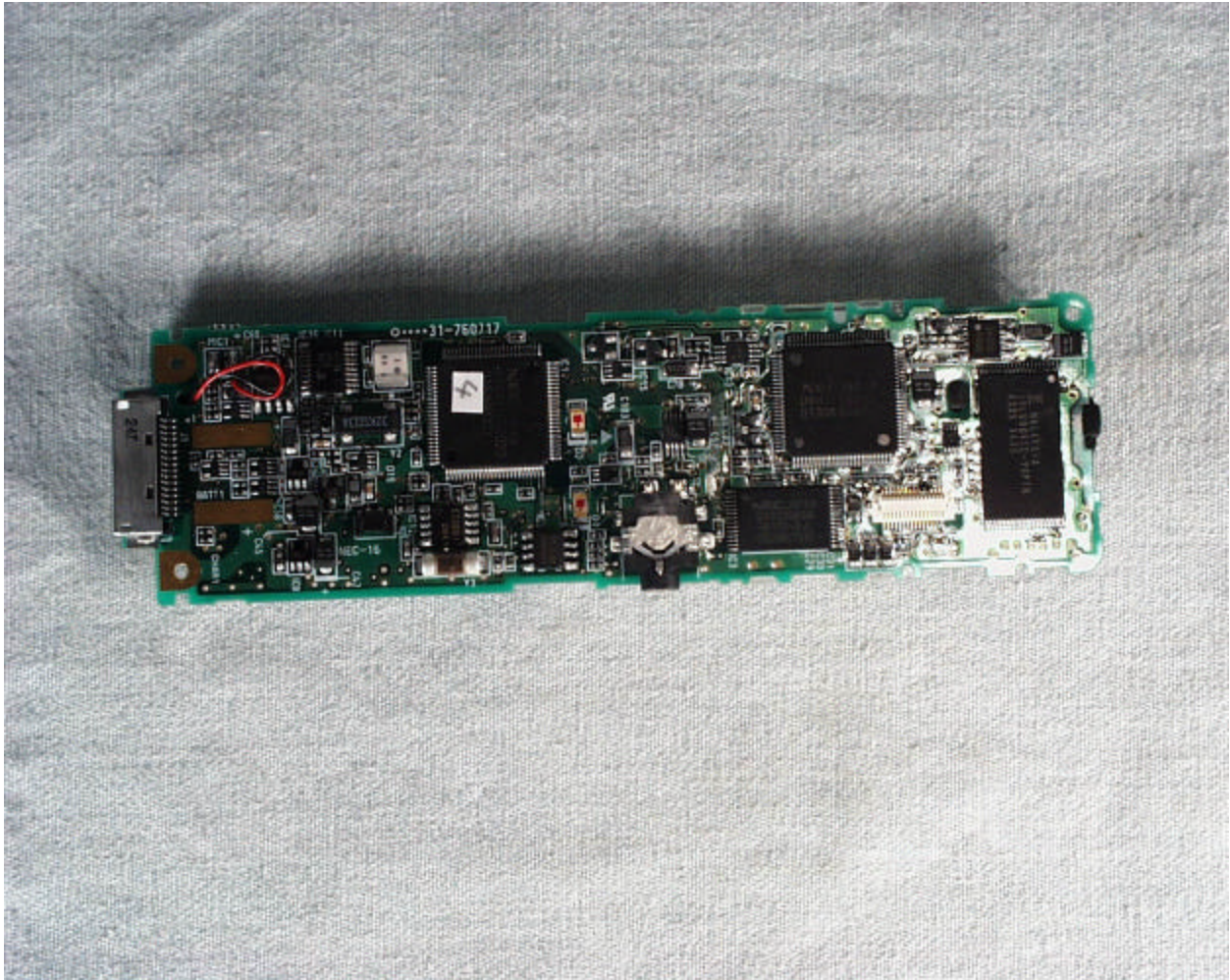
Side A of the Digital board
