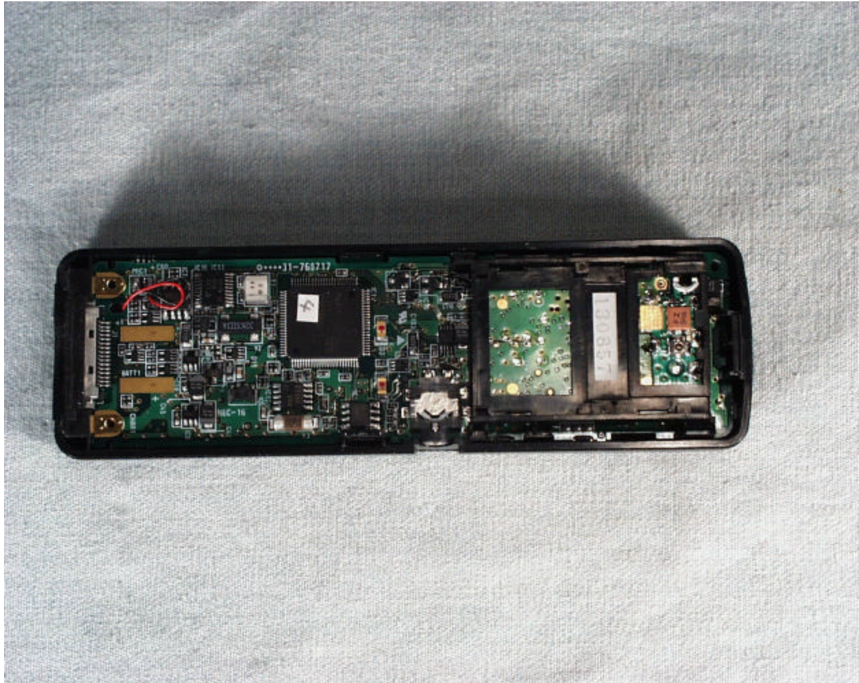
Inside View of the SN531 PSTH-A
