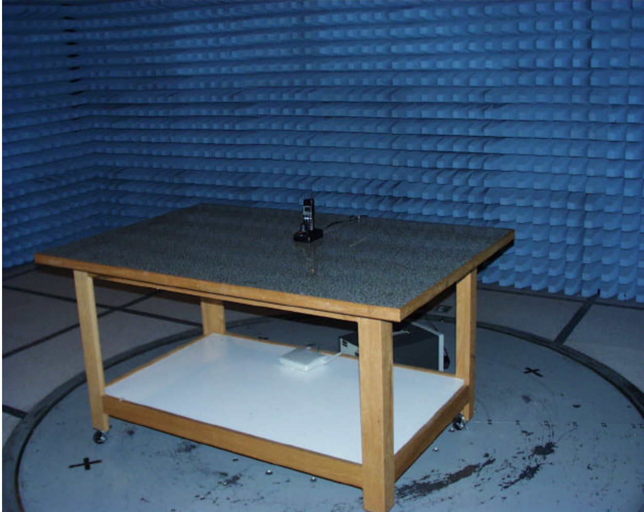
Front View of Worst Case Radiated and Line Conducted Emissions Test Set-up
