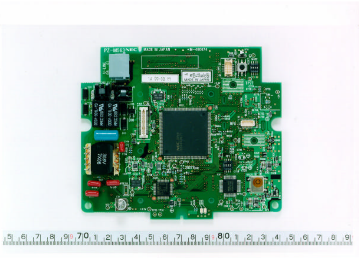
Component side of the interface board
