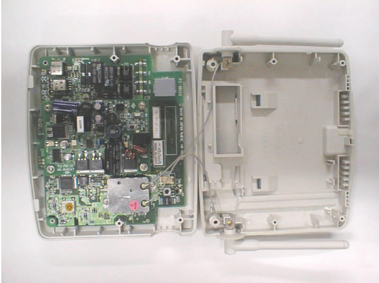
Inside View of the SN999CSEQ
