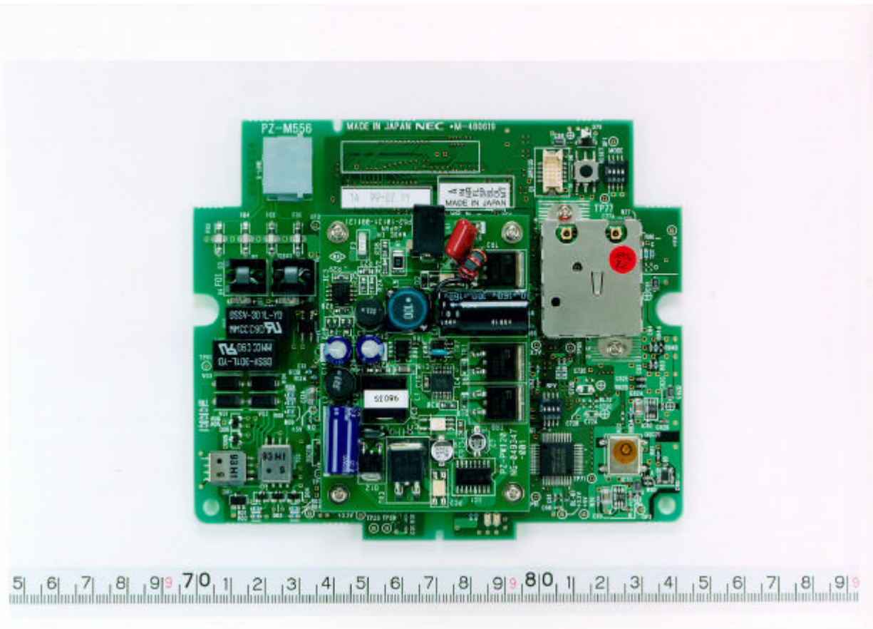
SN999CSEQ with all board installed
