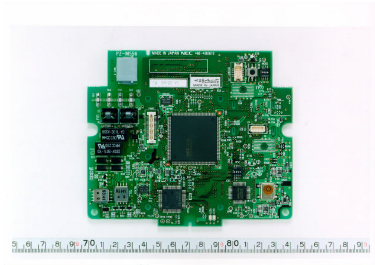
Component side of the interface board
