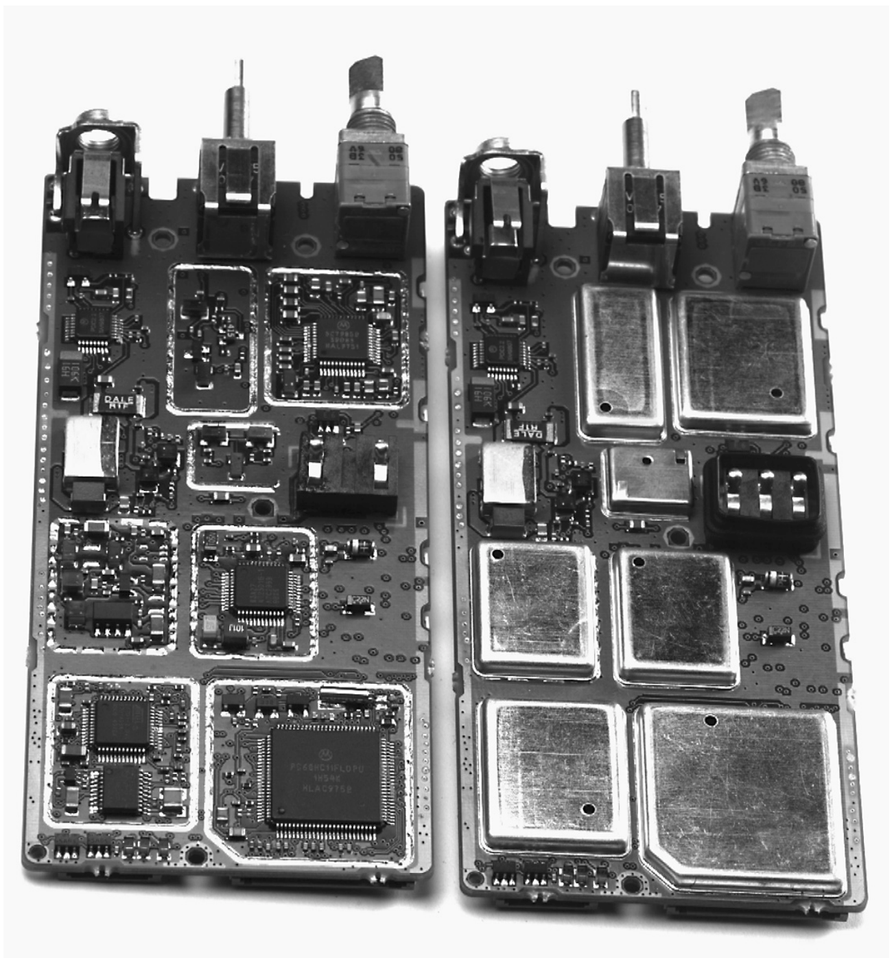
Back side of transceiver board with shields removed
