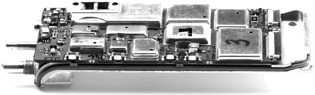
Transceiver Board mounted on chassis
