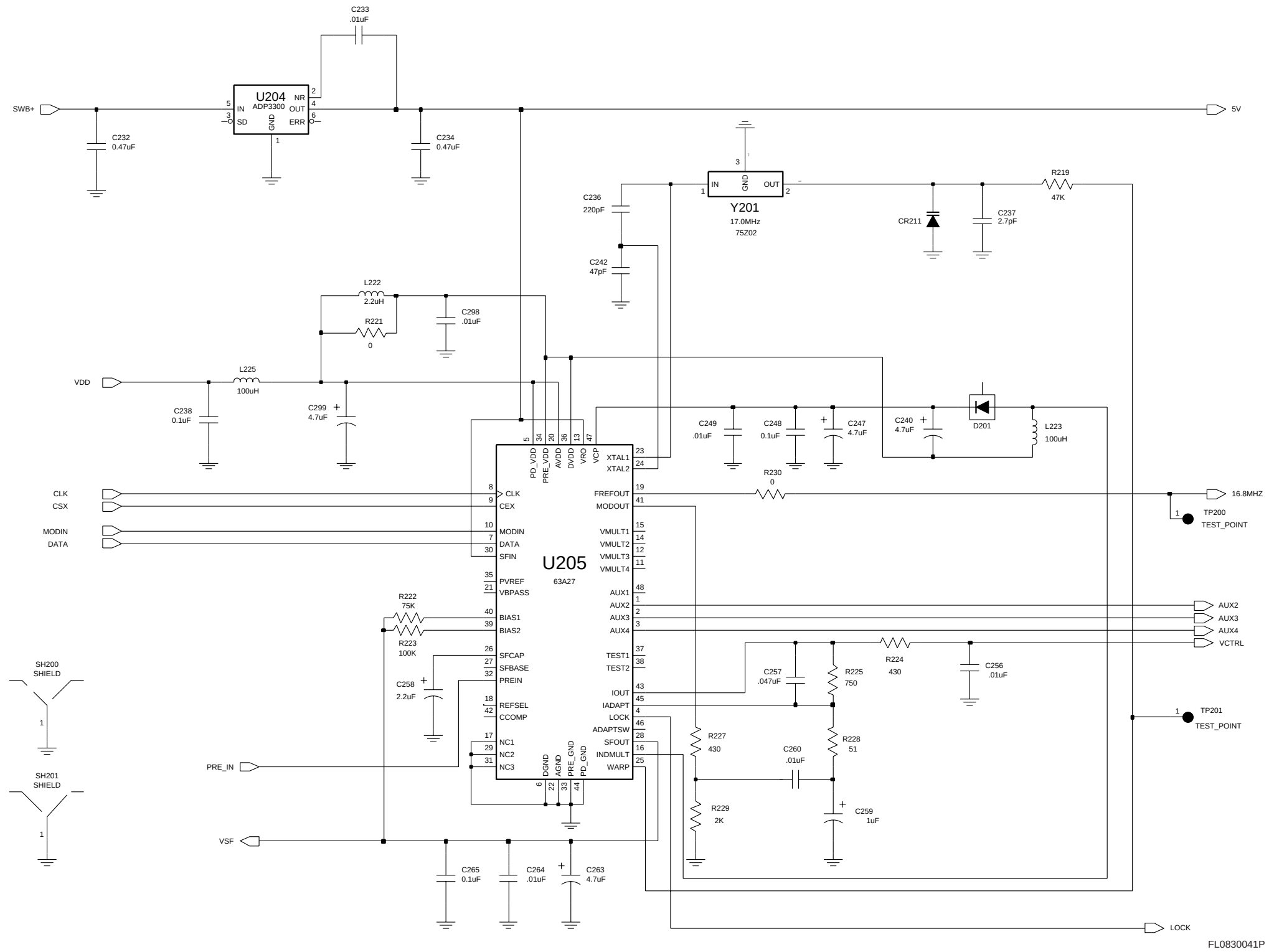
Low Band RF Board FGU Synthesizer Schematic
