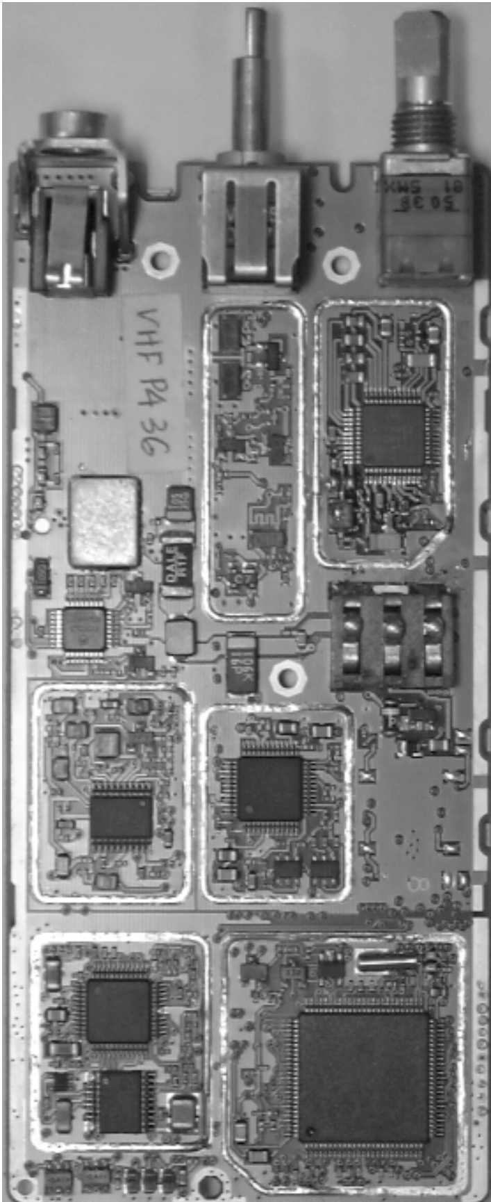
Back of Transceiver Board without Shields 10--10
