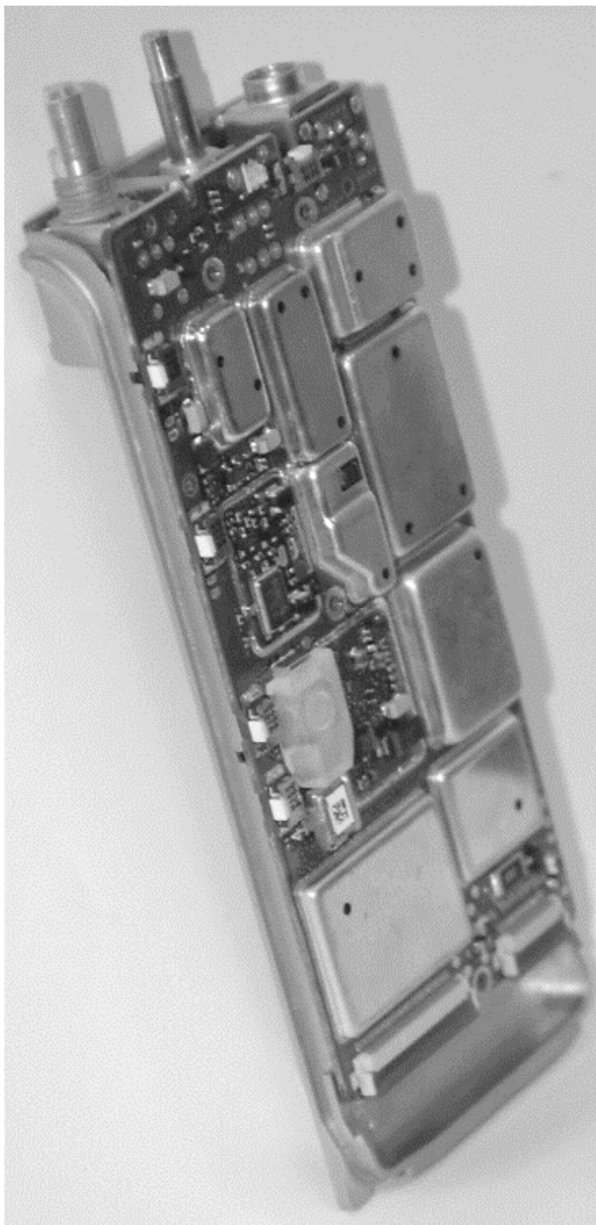
Transceiver Board and Chassis 10--6
