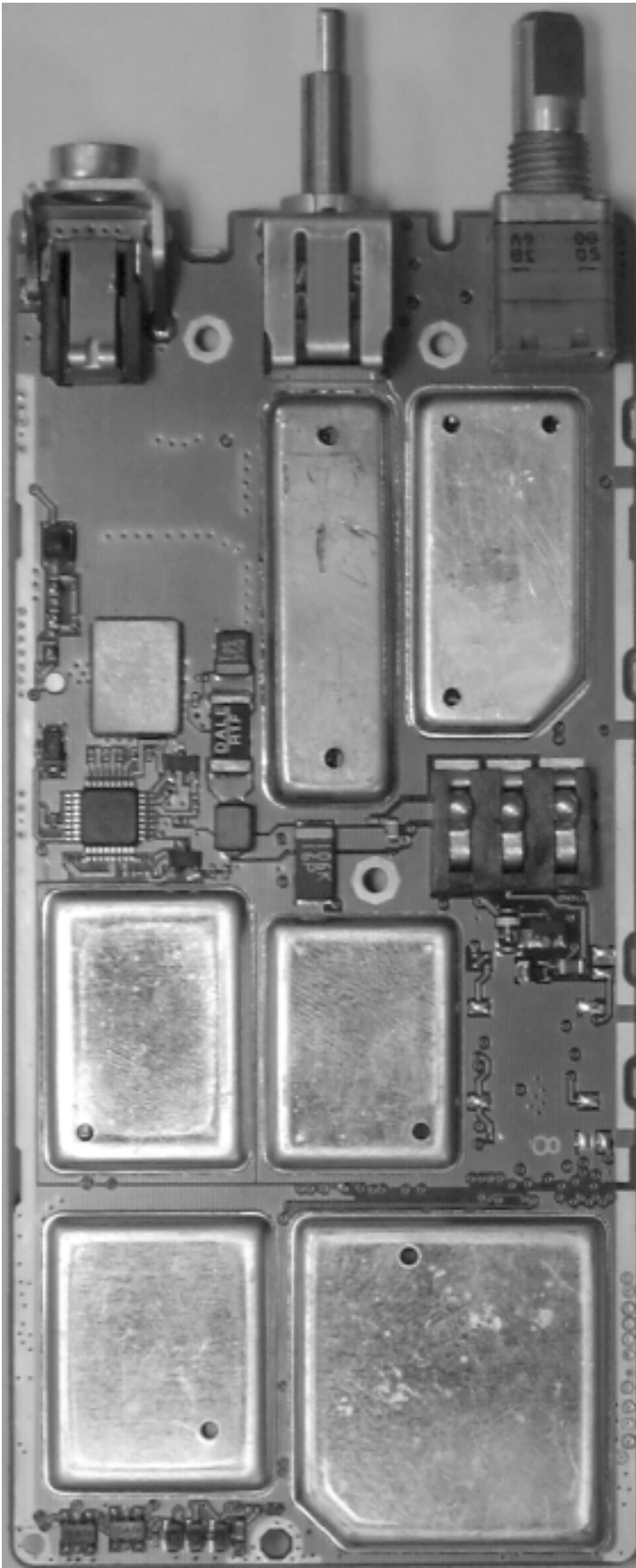
Back of Transceiver Board with Shields 10--9
