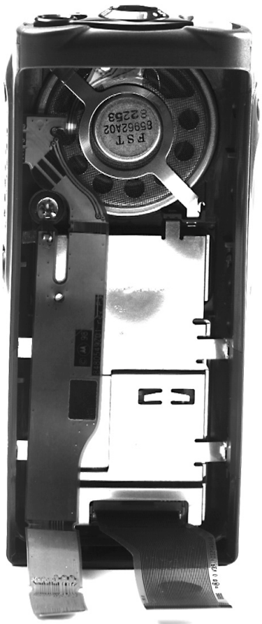
Back view of the front housing showing keypad board installed
