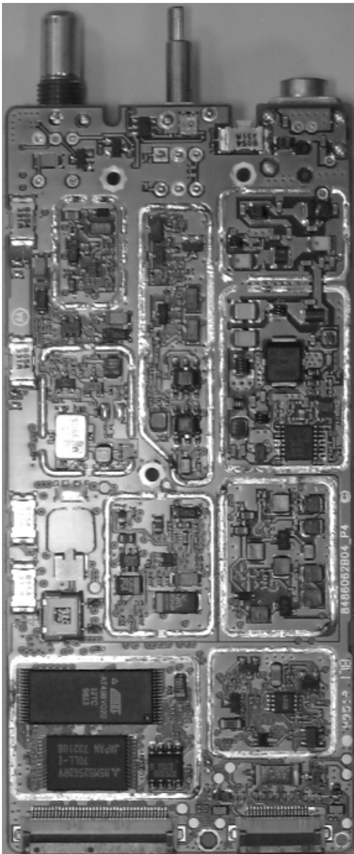
Top of Transceiver Board without Shields 10--8
