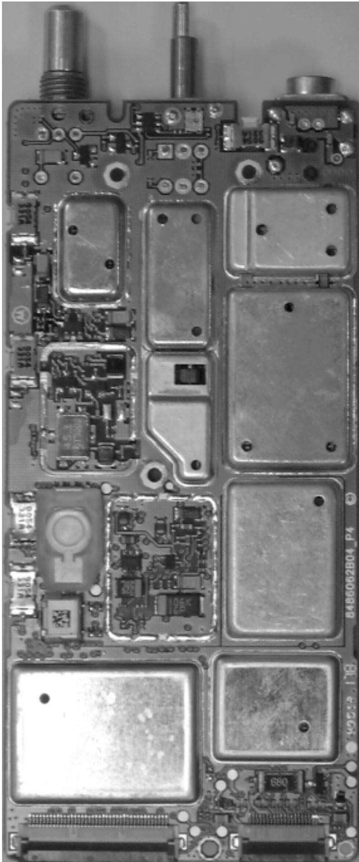
Top of Transceiver Board with Shields 10-7
