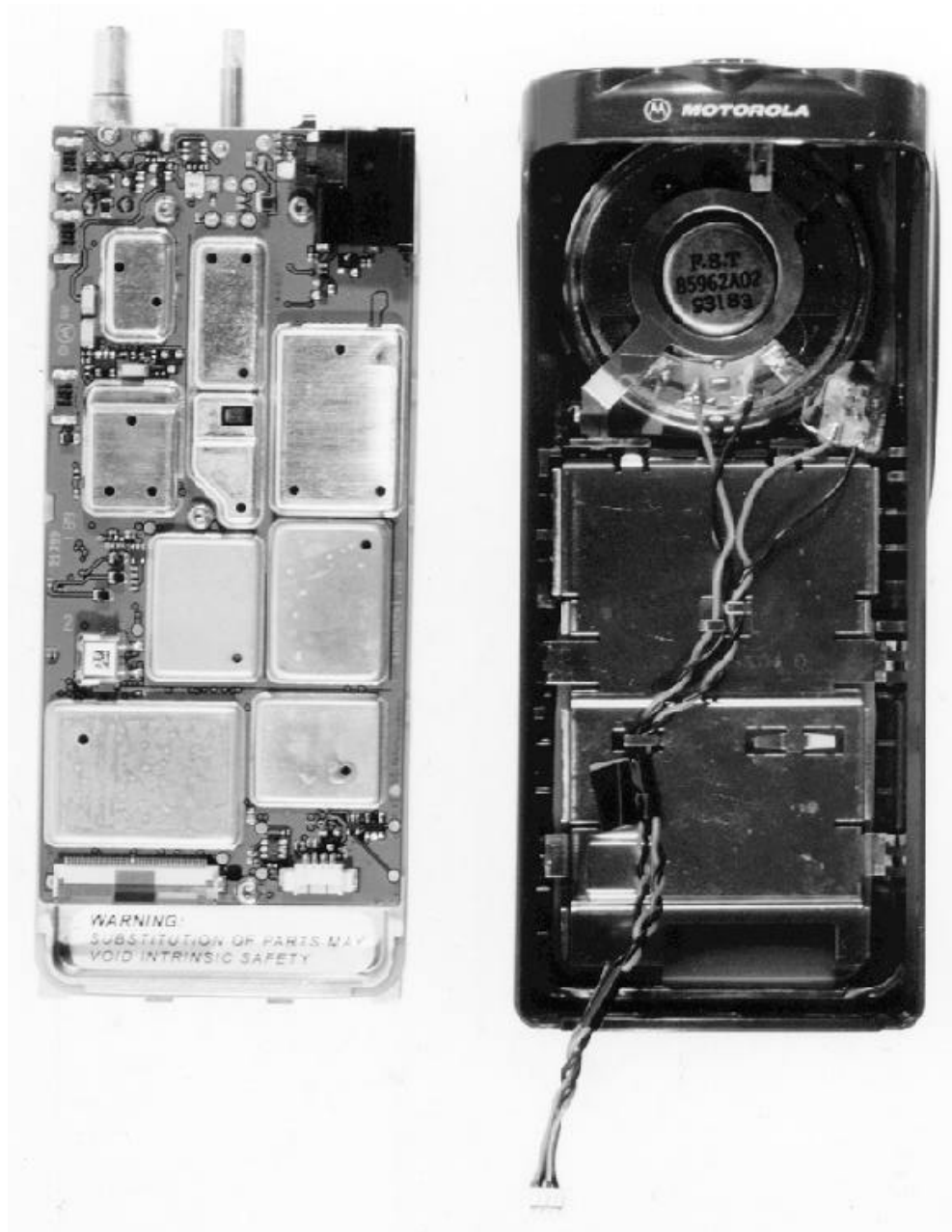
View with Front Housing Open up (**Plain Model)
