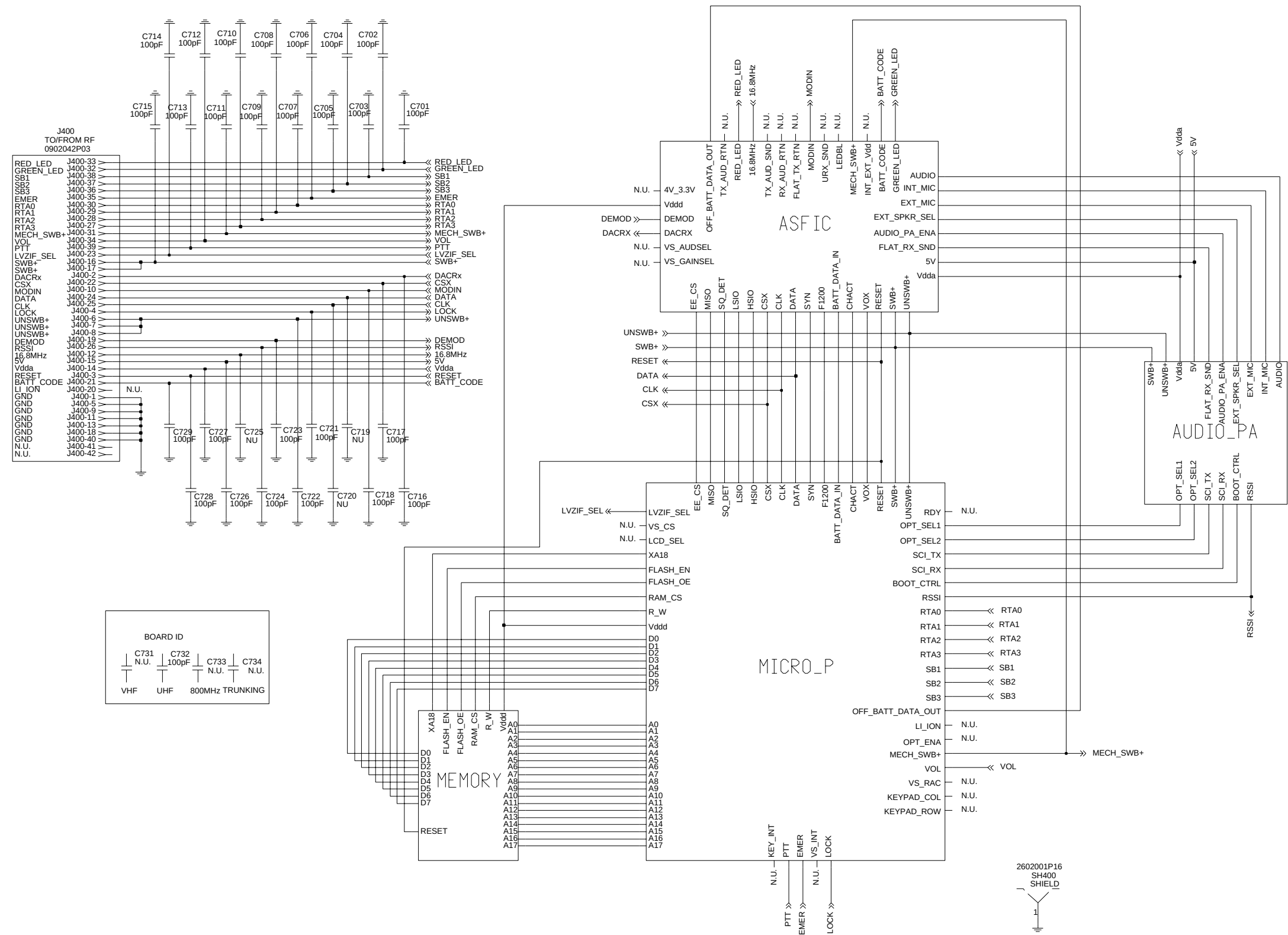
Figure 4-12: Complete Controller Schematic Diagram
