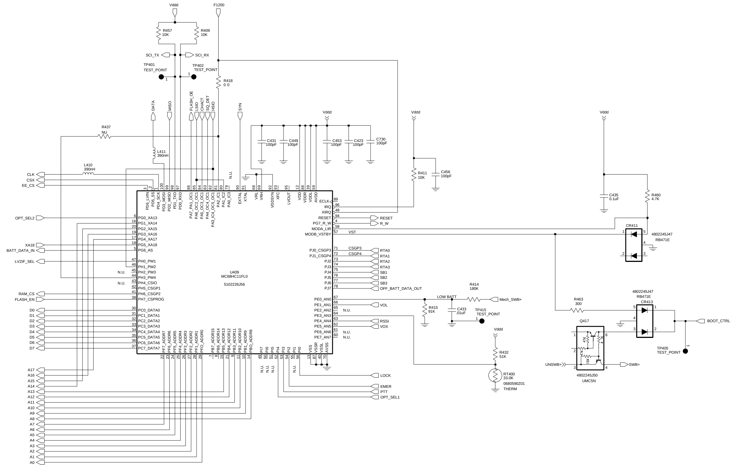
Figure 4-14: Controller Micro Processor Schematic Diagram
