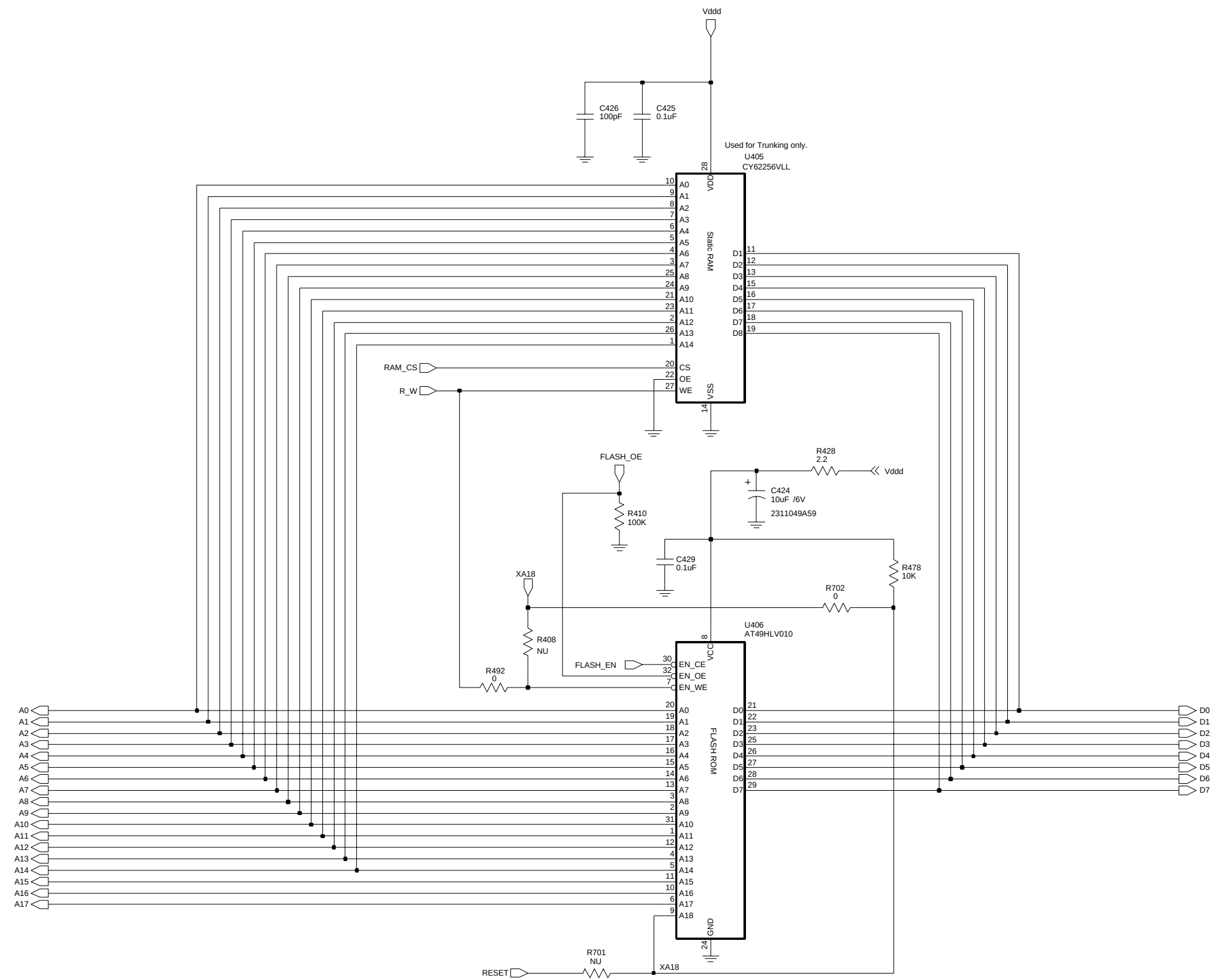
Figure 4-15: Controller Memory Schematic Diagram
