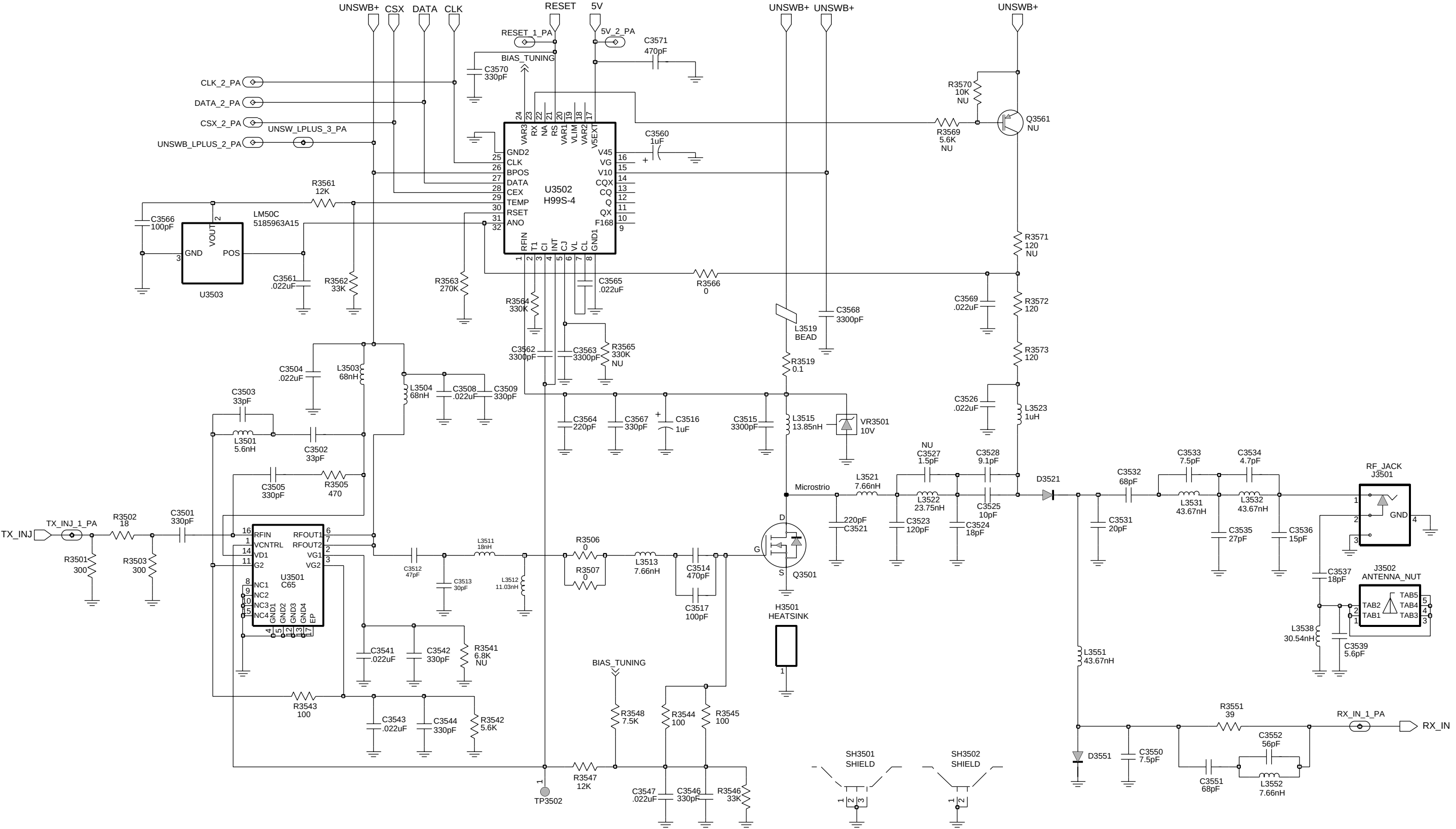
Figure 4-24: VHF Transmitter Schematic Diagram
