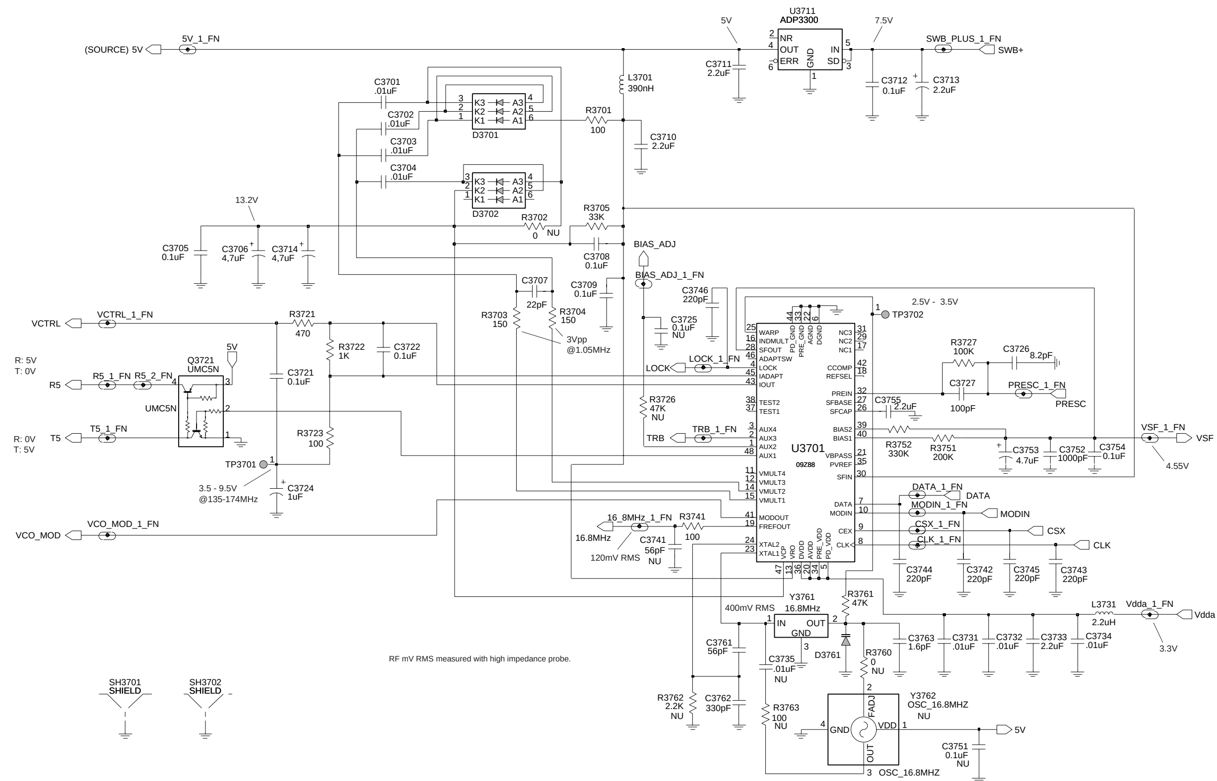
Figure 4-22: VHF Synthesizer Schematic Diagram
