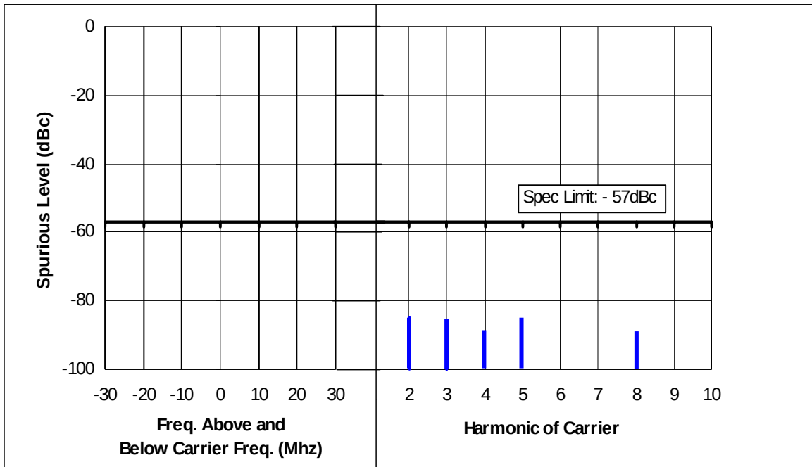
Figure 6F-3: Hi-Power, 173.9875 MHz, 12.5 kHz Channel Spacing
