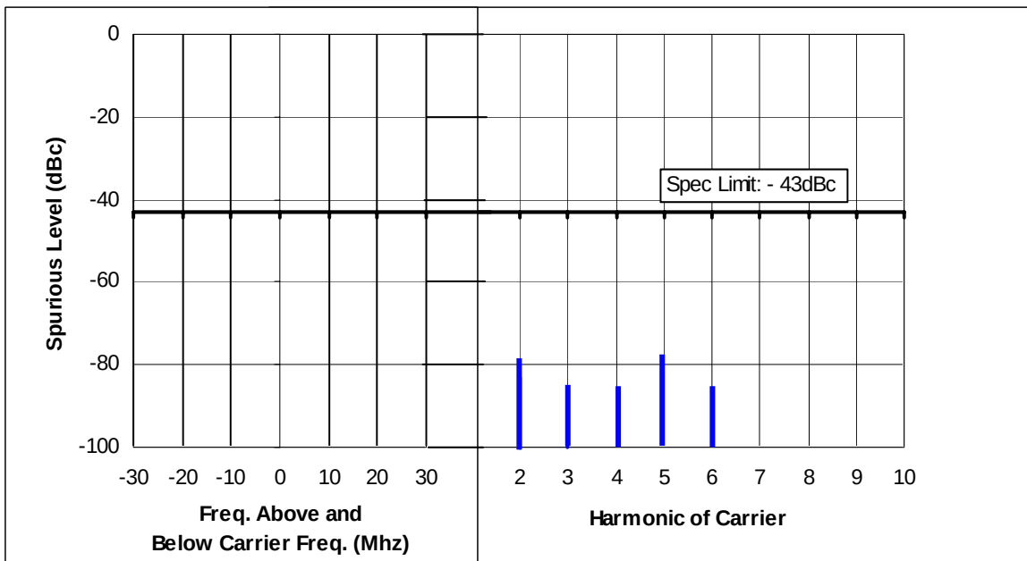
Figure 6F-10: Lo-Power, 136.0125 MHz, 25 kHz Channel Spacing
