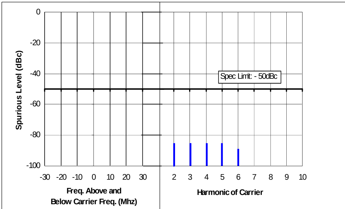
Figure 6F-8: Lo-Power, 153.0125 MHz, 12.5 kHz Channel Spacing
