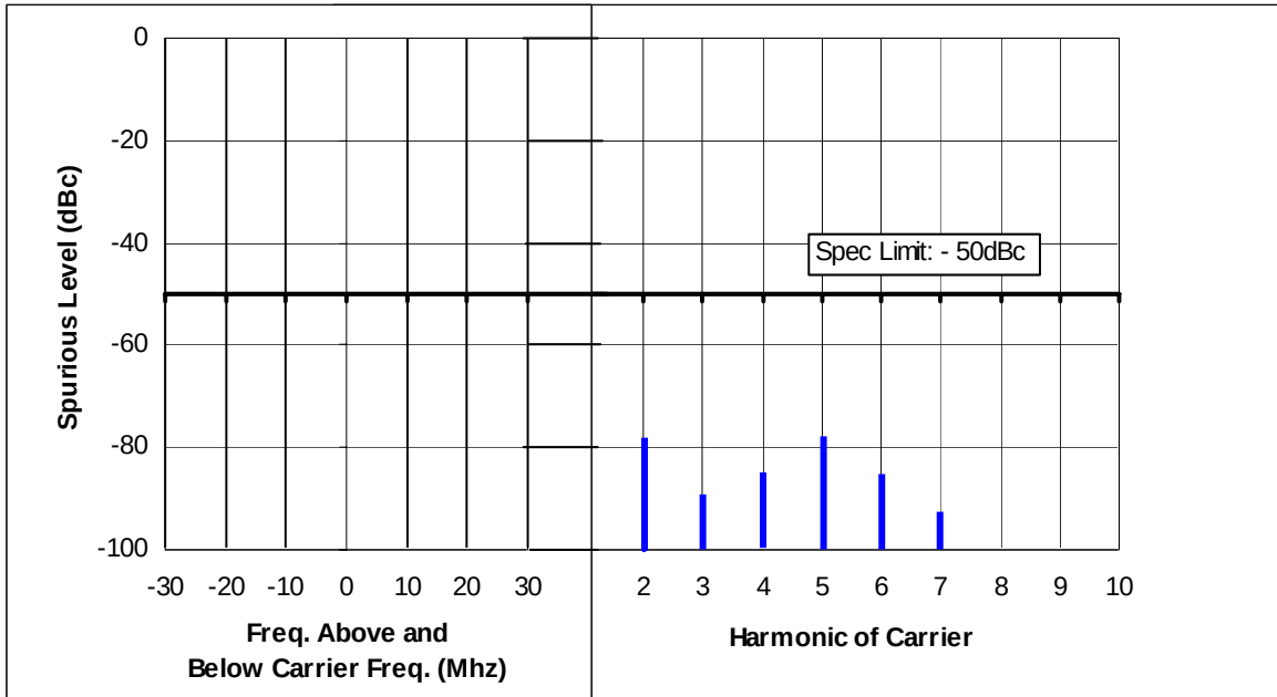
Figure 6F-7: Lo-Power, 136.0125 MHz, 12.5 kHz Channel Spacing
