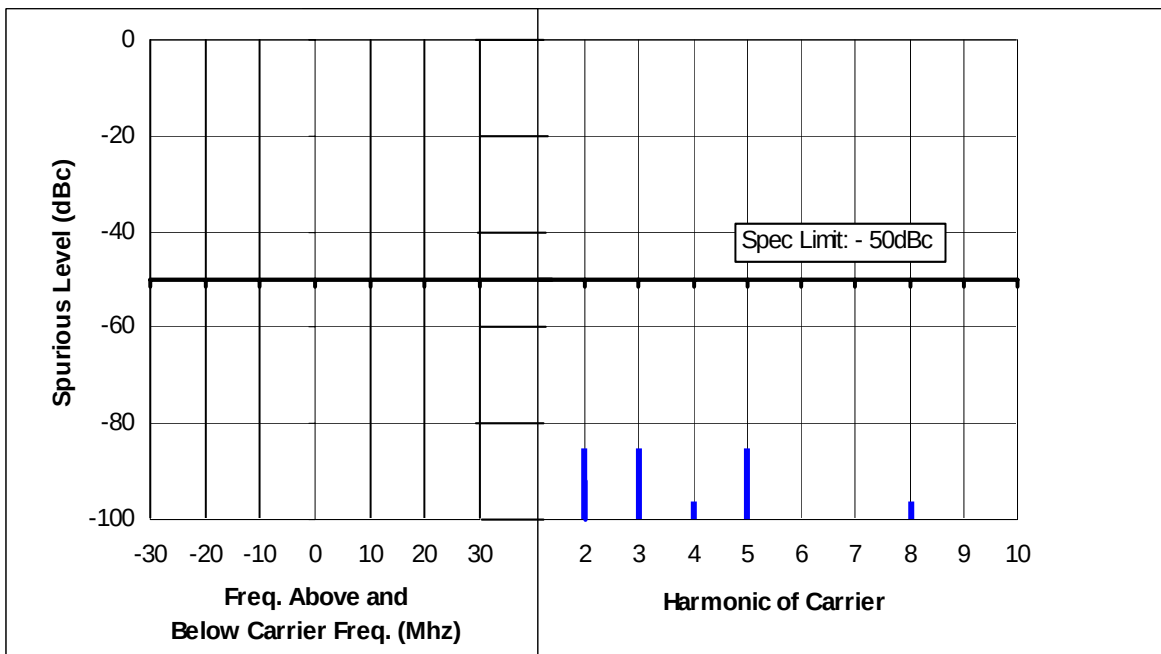
Figure 6F-6: Hi-Power, 173.9875 MHz, 25 kHz Channel Spacing
