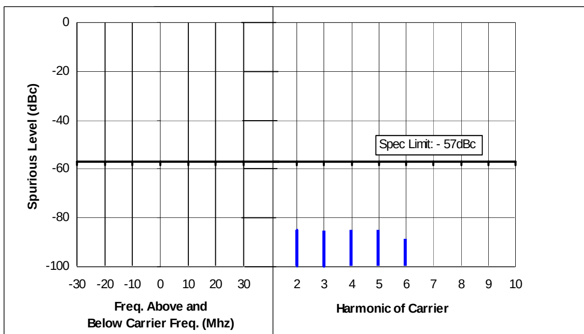
Figure 6F-2: Hi-Power, 153.0125 MHz, 12.5 kHz Channel Spacing
