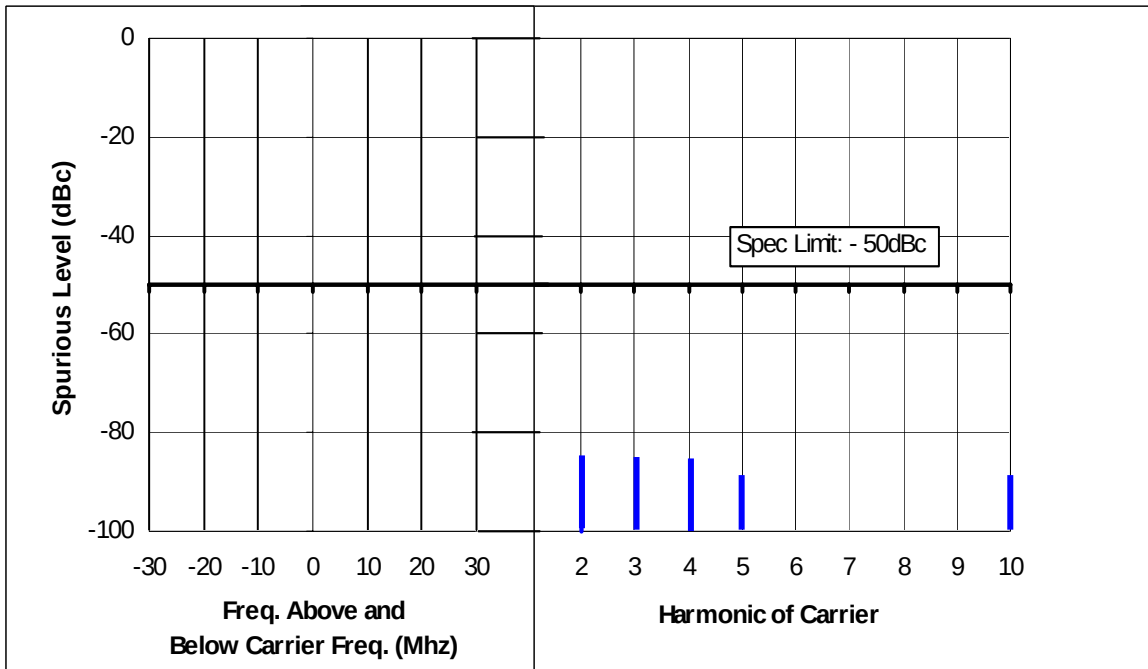
Figure 6F-9: Lo-Power, 173.9875 MHz, 12.5 kHz Channel Spacing
