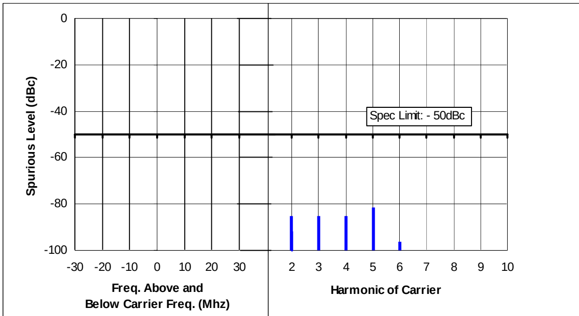
Figure 6F-5: Hi-Power, 153.0125 MHz, 25 kHz Channel Spacing
