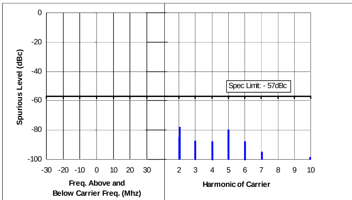
Figure 6F-1: Hi-Power, 136.0125 MHz, 12.5 kHz Channel Spacing
