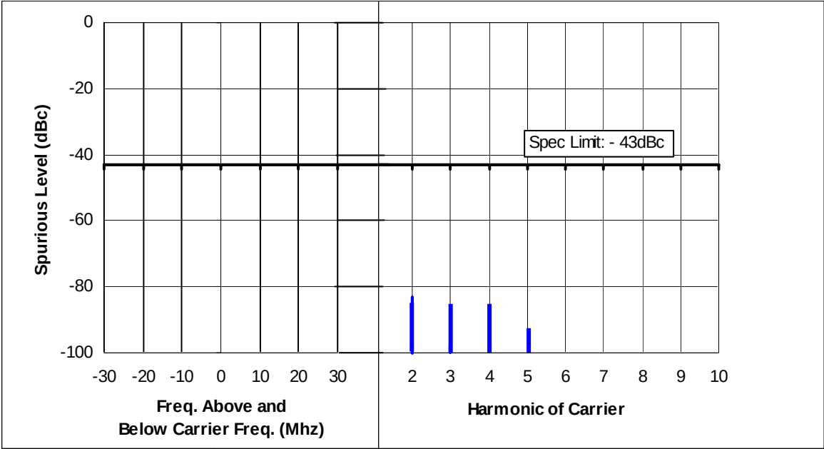
Figure 6F-12: Lo-Power, 173.9875 MHz, 25 kHz Channel Spacing
