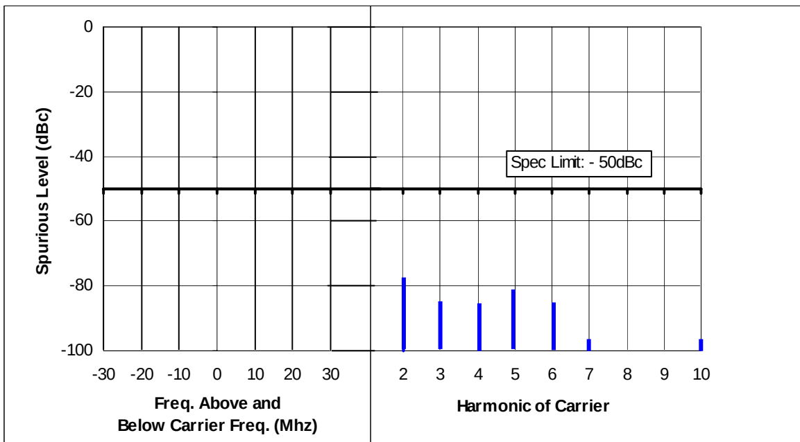
Figure 6F-4: Hi-Power, 136.0125 MHz, 25 kHz Channel Spacing
