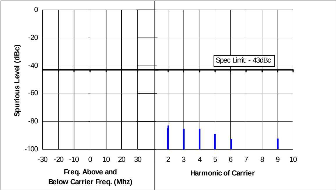
Figure 6F-11: Lo-Power, 153.0125 MHz, 25 kHz Channel Spacing
