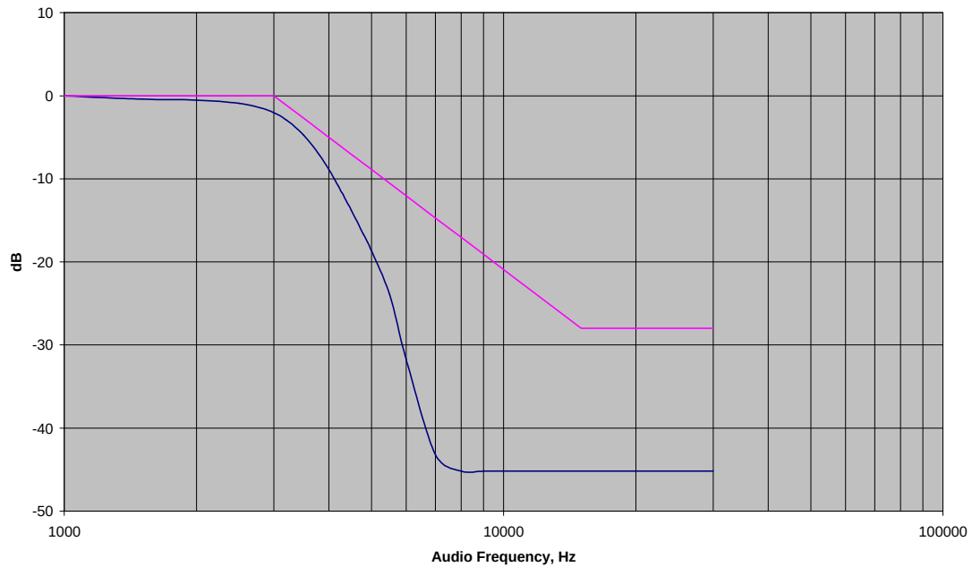
Audio Low Pass Filter Response (25kHz Channel Spacing) FCC ID: AZ489FT3801
