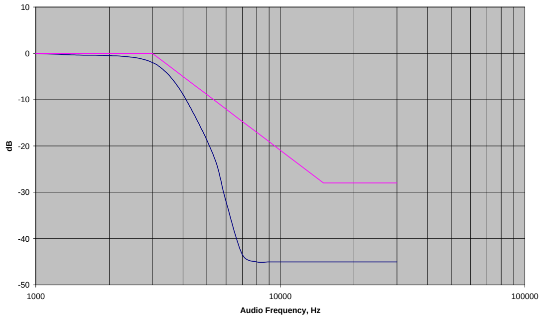
Audio Low Pass Filter Response (12.5kHz Channel Spacing) FCC ID: AZ489FT3801
