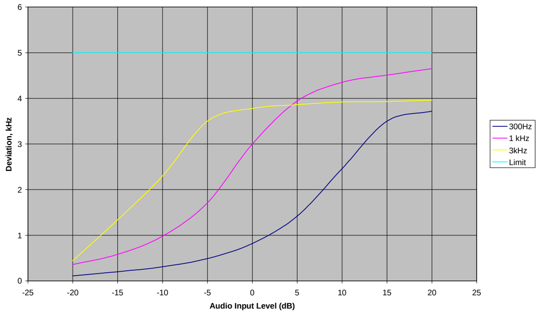
Modulation Limiting (25kHz Channel Spacing) FCC ID: AZ489FT3801
