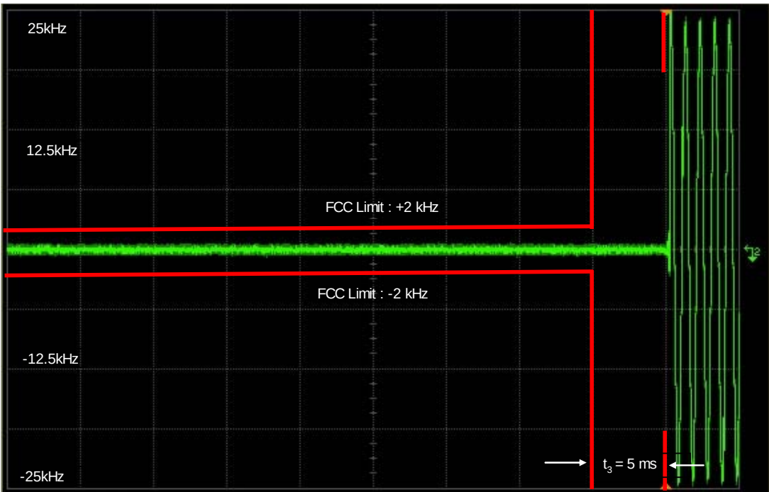
Figure 6I-8: Lo Power, 25 kHz De-Key Decay Time
