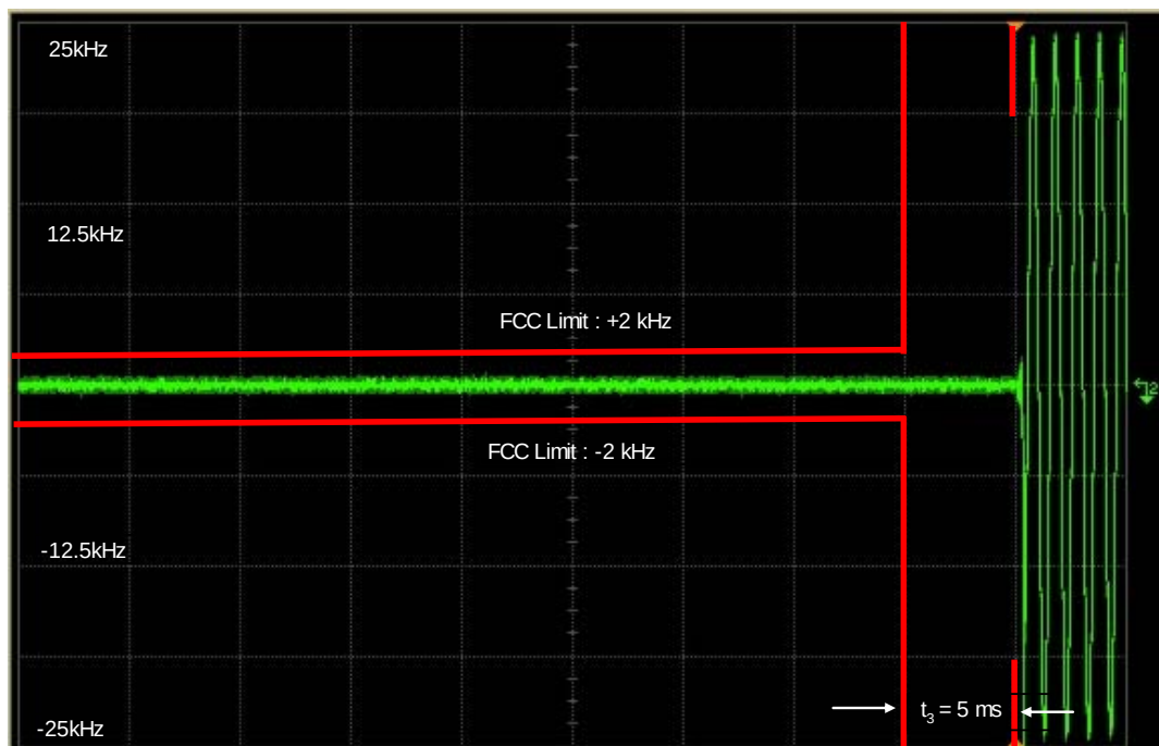
Figure 6I-4: Hi Power, 25 kHz De-Key Decay Time
