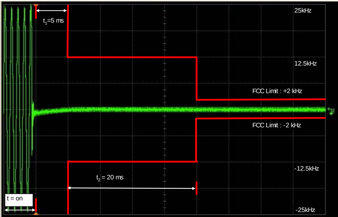
Figure 6I-1: Hi Power, 12.5 kHz Key-Up Attack Time
