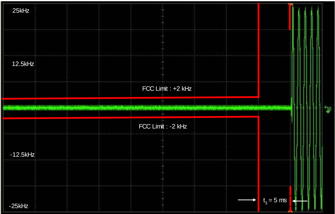
Figure 6I-6: Lo Power, 12.5 kHz De-Key Decay Time
