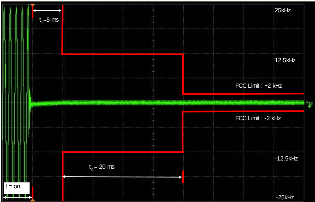
Figure 6I-5: Lo Power, 12.5 kHz Key-Up Attack Time
