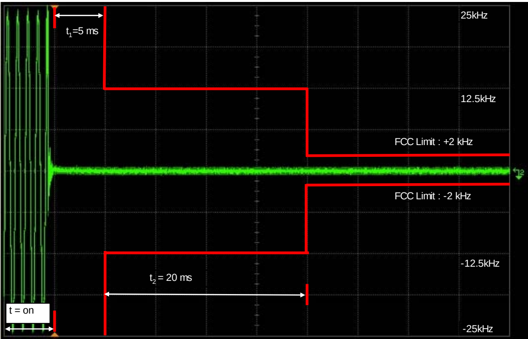
Figure 6I-7: Lo Power, 25 kHz Key-Up Attack Time
