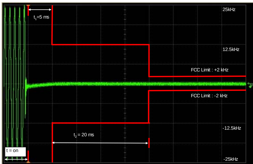
Figure 6I-3: Hi Power, 25 kHz Key-Up Attack Time
