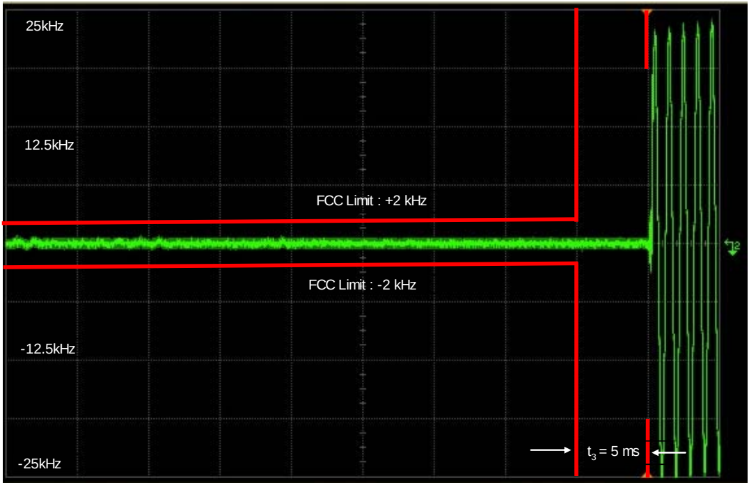
Figure 6I-2: Hi Power, 12.5 kHz De-Key Decay Time
