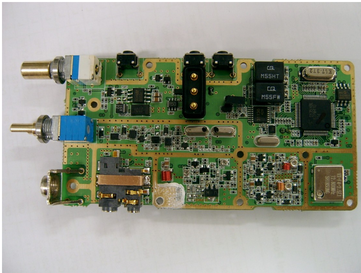
Figure 9-2: Bottom Side of PCB.
