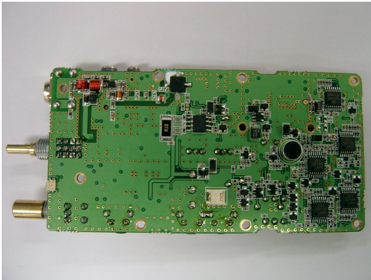
Figure 9-1: Top Side of PCB.
