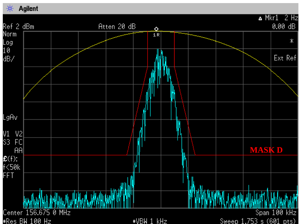
Figure 6E-8: 12.5 kHz Channel Spacing, 156.675 MHz, APCO25 Digital Voice (8K10F1E), 8K10F1E
