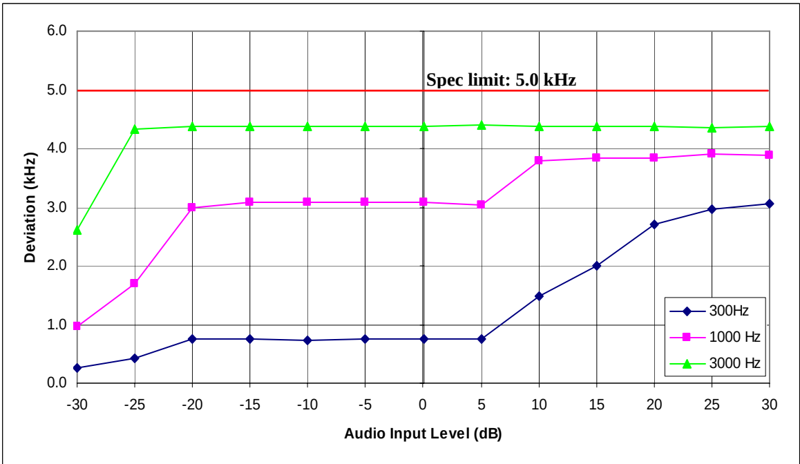
Figure 6D-4: 25 kHz Channel Spacing, 156.675 MHz, Carrier Squelch (CSQ) Mode
