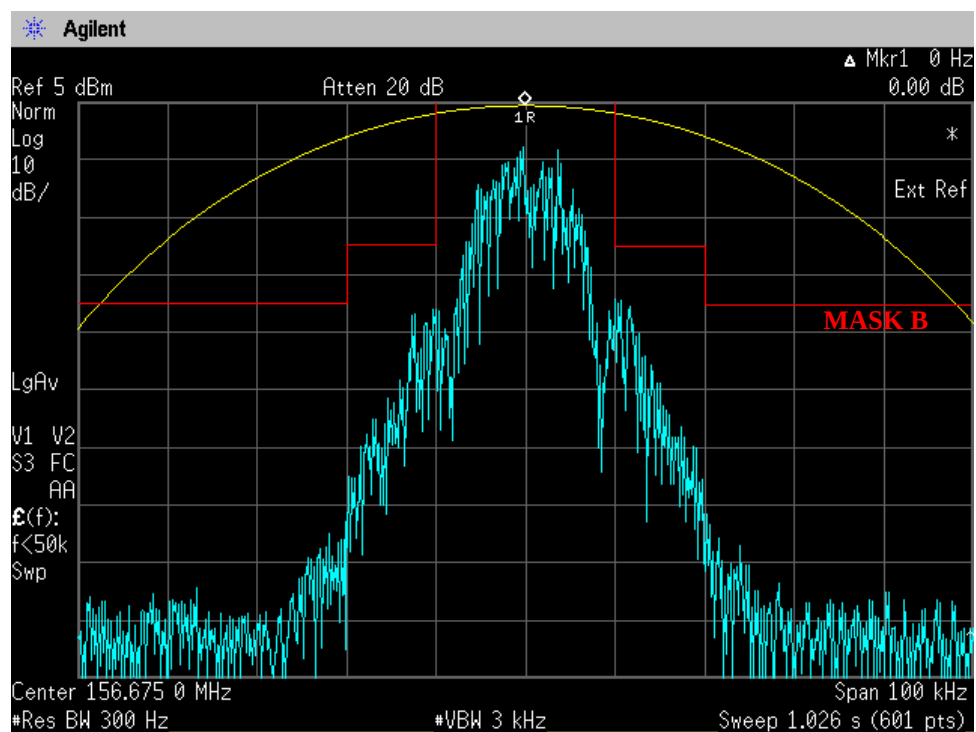
Figure 6E-10: 25.0 kHz Channel Spacing, 156.675 MHz, I Voice Encryption, 20K0F1E ,
