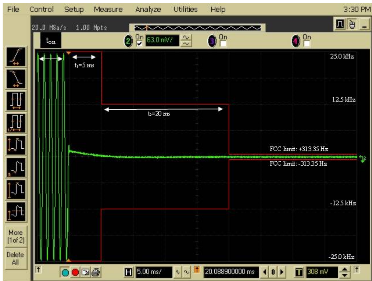
Figure 6I-7: 1.6 Watt, 25 kHz Key-Up Attack Time
