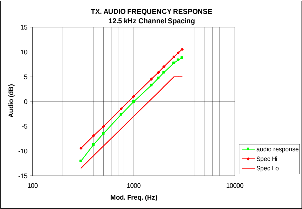
Figure 6B-1: 12.5 kHz Channel Spacing, 156.675 MHz, Transmit Audio Frequency Response
