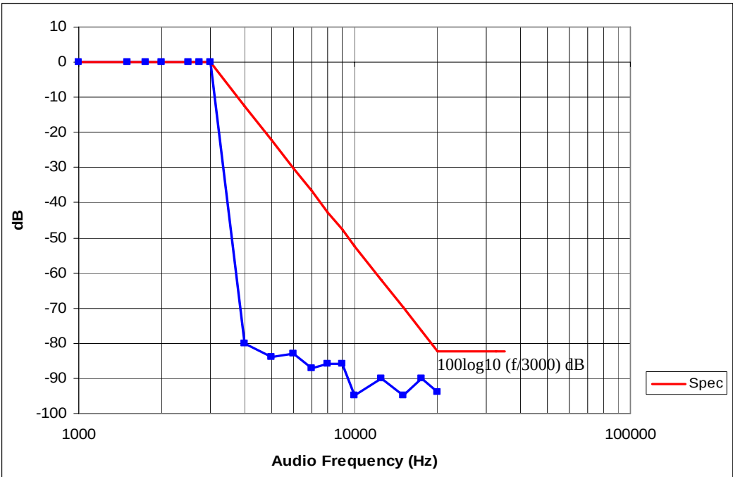
Figure 6C-1: 12.5 kHz Channel Spacing, 156.675 MHz, Transmit Audio Low Pass Filter Response
