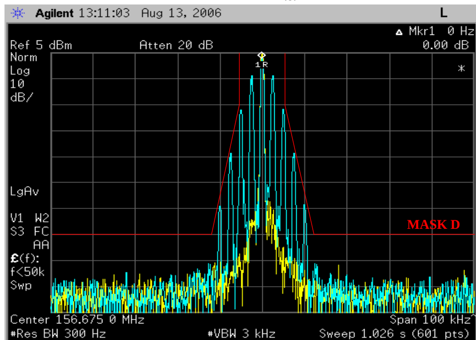
Figure 6E-1: 12.5 kHz Channel Spacing, 156.675 MHz, 2500 Hz Audio Modulation Only, 11K0F3E
