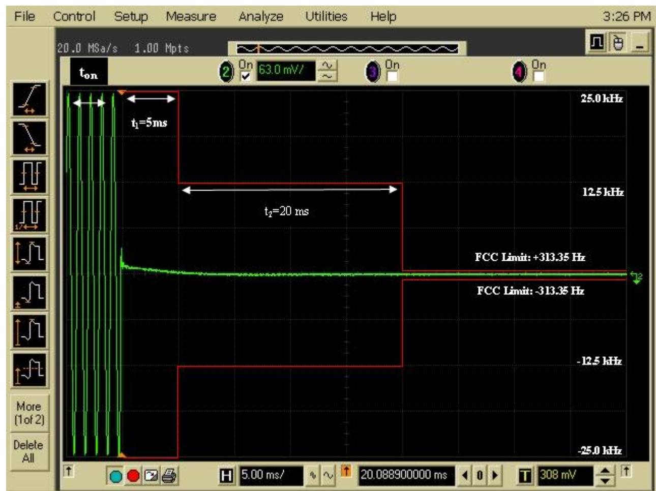
Figure 6I-1: 2.8 Watts, 12.5 kHz Key-Up Attack Time
