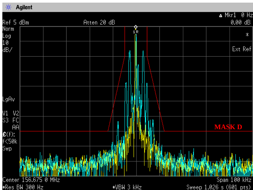
Figure 6E-3: 12.5 kHz Channel Spacing, 156.675 MHz, 2500 Hz Audio and DPL Tone Modulation, 11K0F3E
