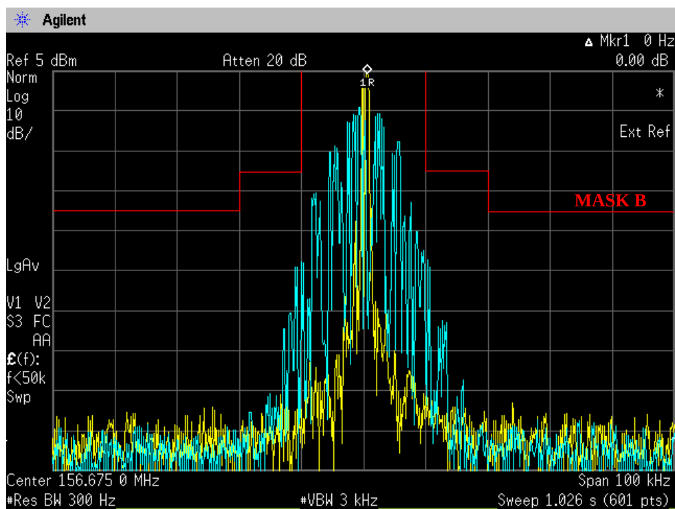
Figure 6E-4: 25 kHz Channel Spacing, 156.675 MHz, 2500 Hz Audio Modulation Only, 16K0F3E
