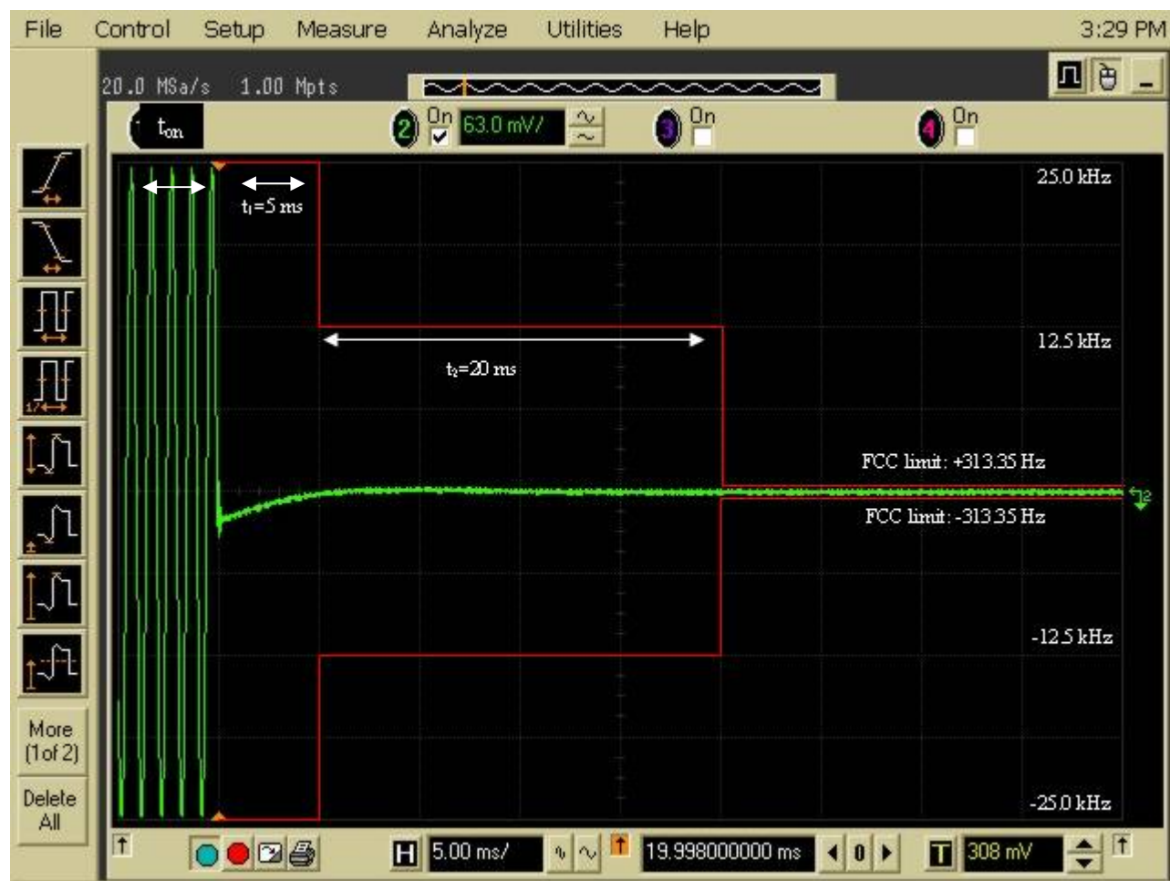
Figure 6I-5: 1.6 Watt, 12.5 kHz Key-Up Attack Time
