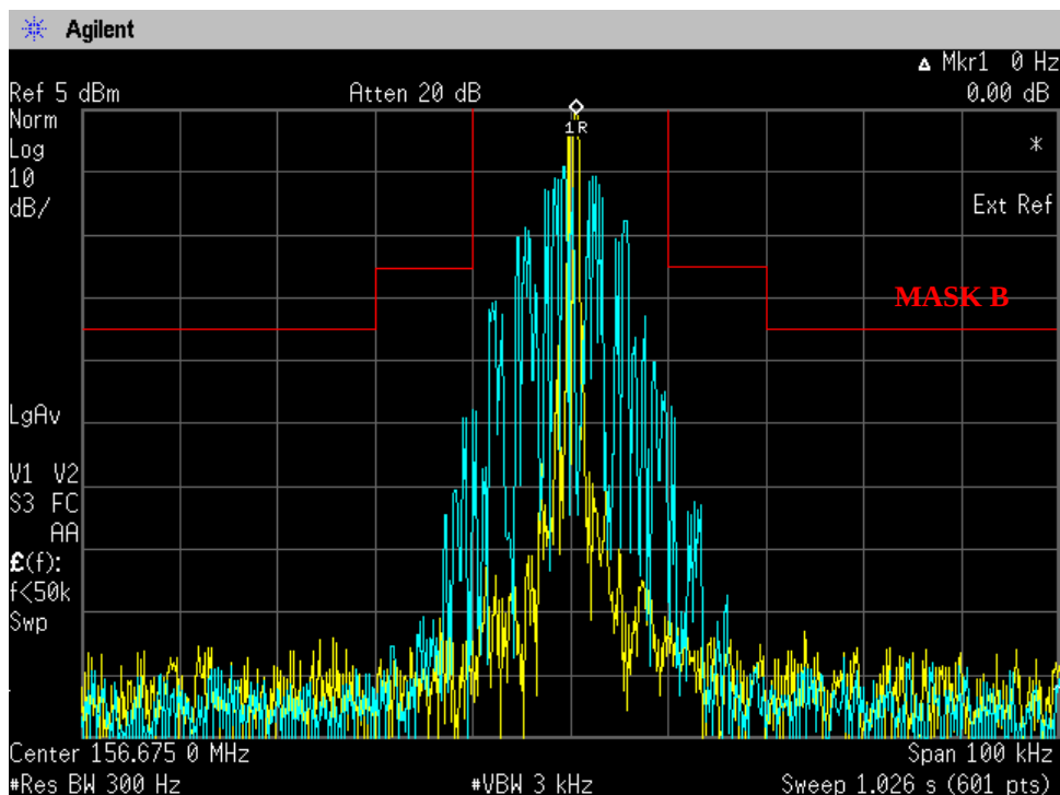
Figure 6E-5: 25 kHz Channel Spacing, 156.675 MHz, 2500 Hz Audio and PL Tone Modulation, 16K0F3E
