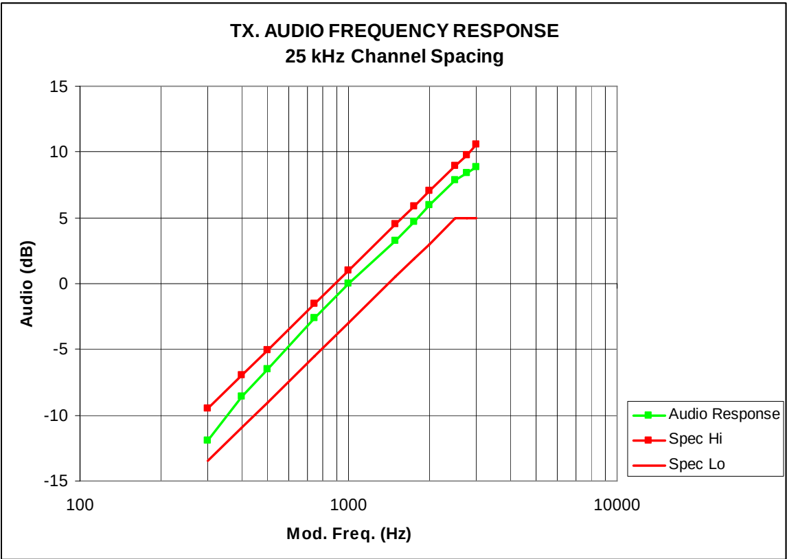
Figure 6B-2: 25 kHz Channel Spacing, 156.675 MHz, Transmit Audio Frequency Response
