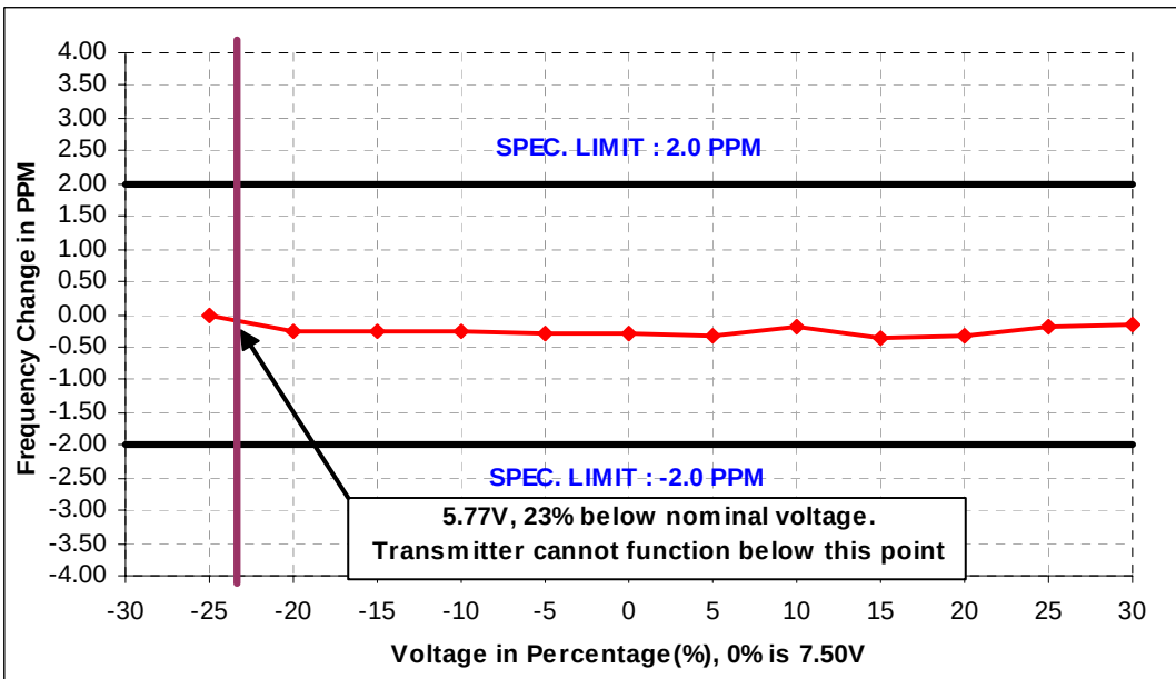
Figure 6H-2: Frequency Stability vs. Voltage
