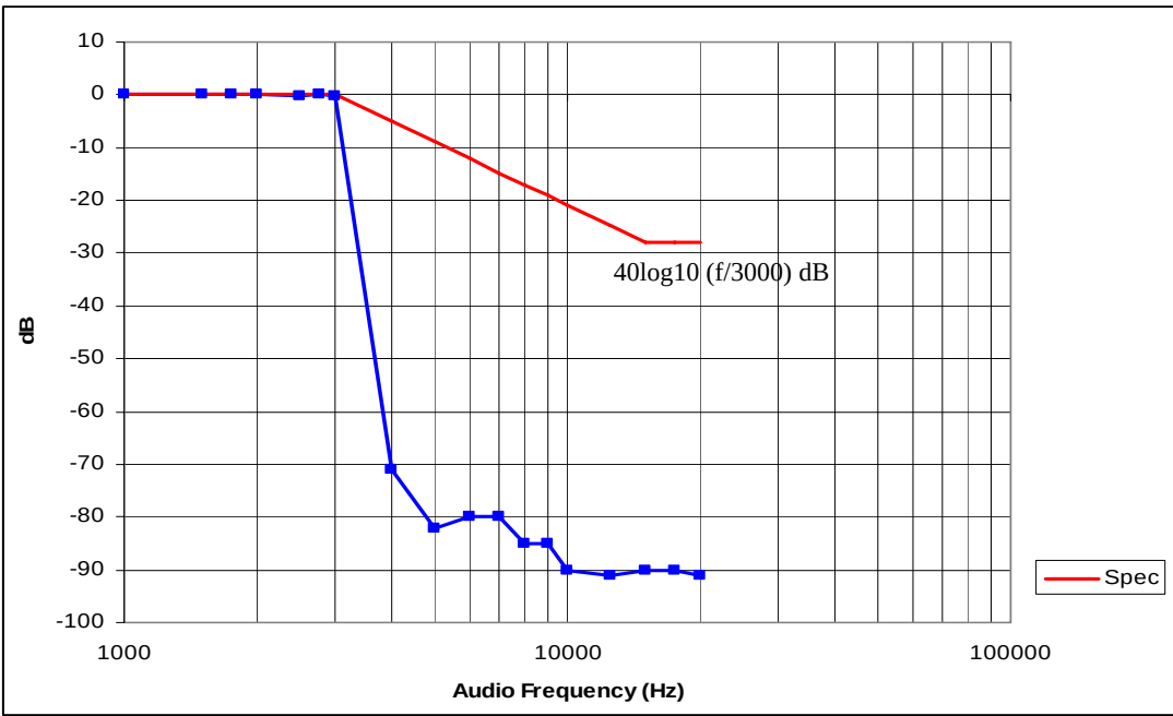
Figure 6C-2: 25 kHz Channel Spacing, 156.675 MHz, Transmit Audio Low Pass Filter Response
