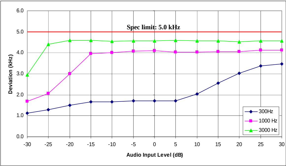
Figure 6D-5: 25 kHz Channel Spacing, 156.675 MHz, Tone Private Line (TPL) Mode
