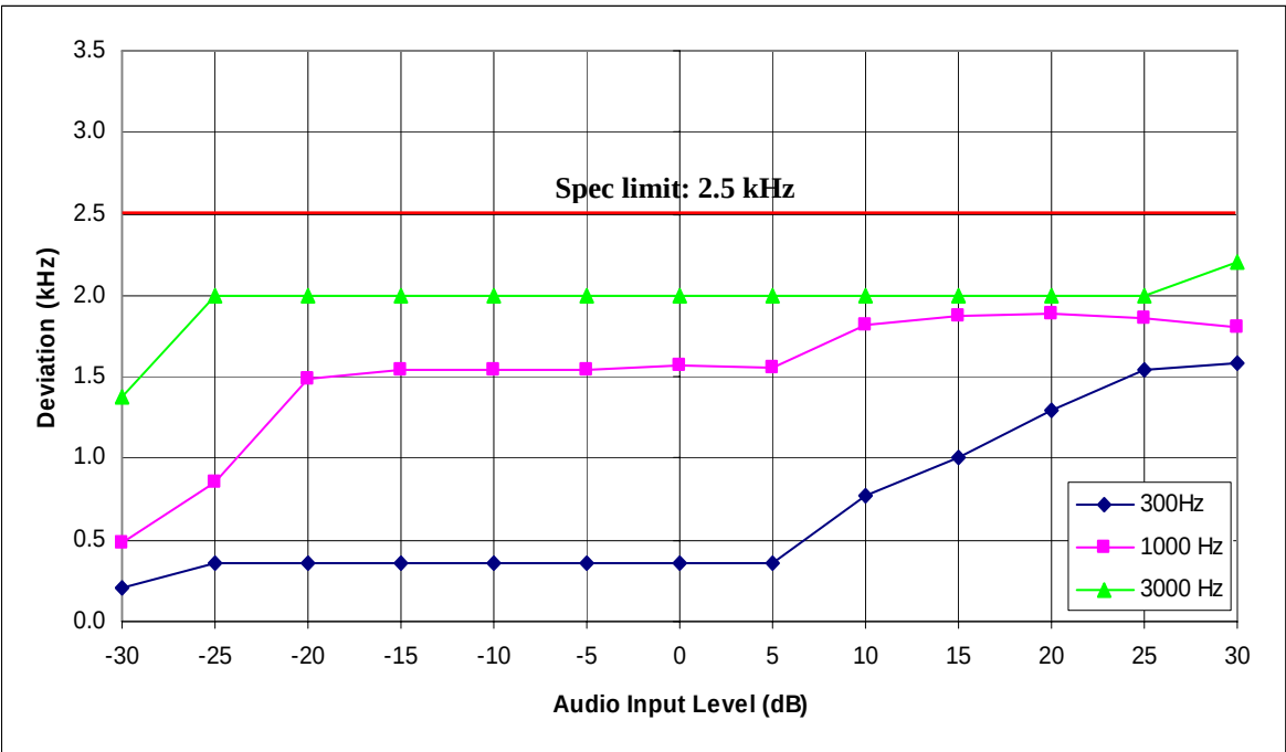
Figure 6D-1: 12.5 kHz Channel Spacing, 156.675 MHz, Carrier Squelch (CSQ) Mode
