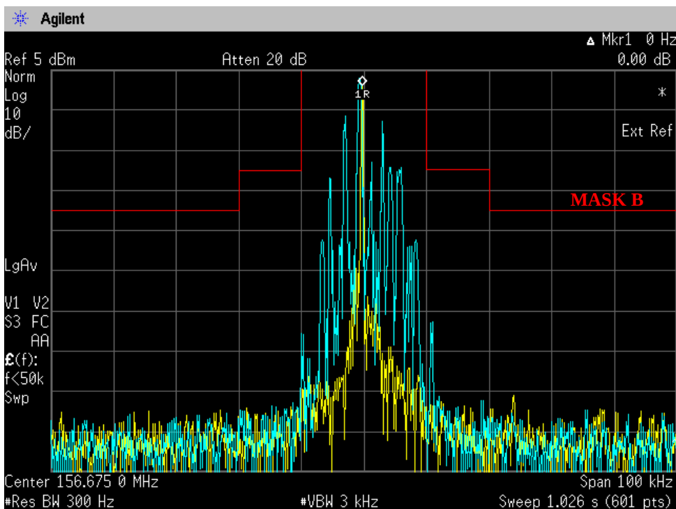
Figure 6E-6: 25 kHz Channel Spacing, 156.675 MHz, 2500 Hz Audio and DPL Tone Modulation, 16K0F3E
