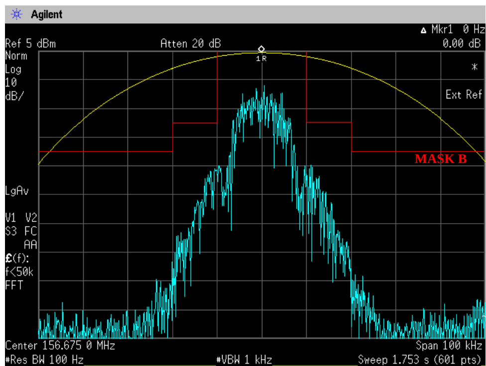
Figure 6E-9: 25.0 kHz Channel Spacing, 156.675 MHz, Voice Encryption, 20K0F1E
