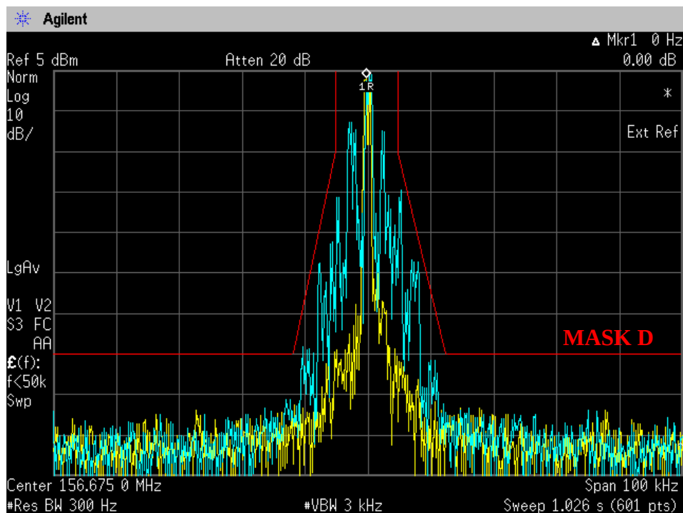
Figure 6E-2: 12.5 kHz Channel Spacing, 156.675 MHz, 2500 Hz Audio and PL Tone Modulation, 11K0F3E
