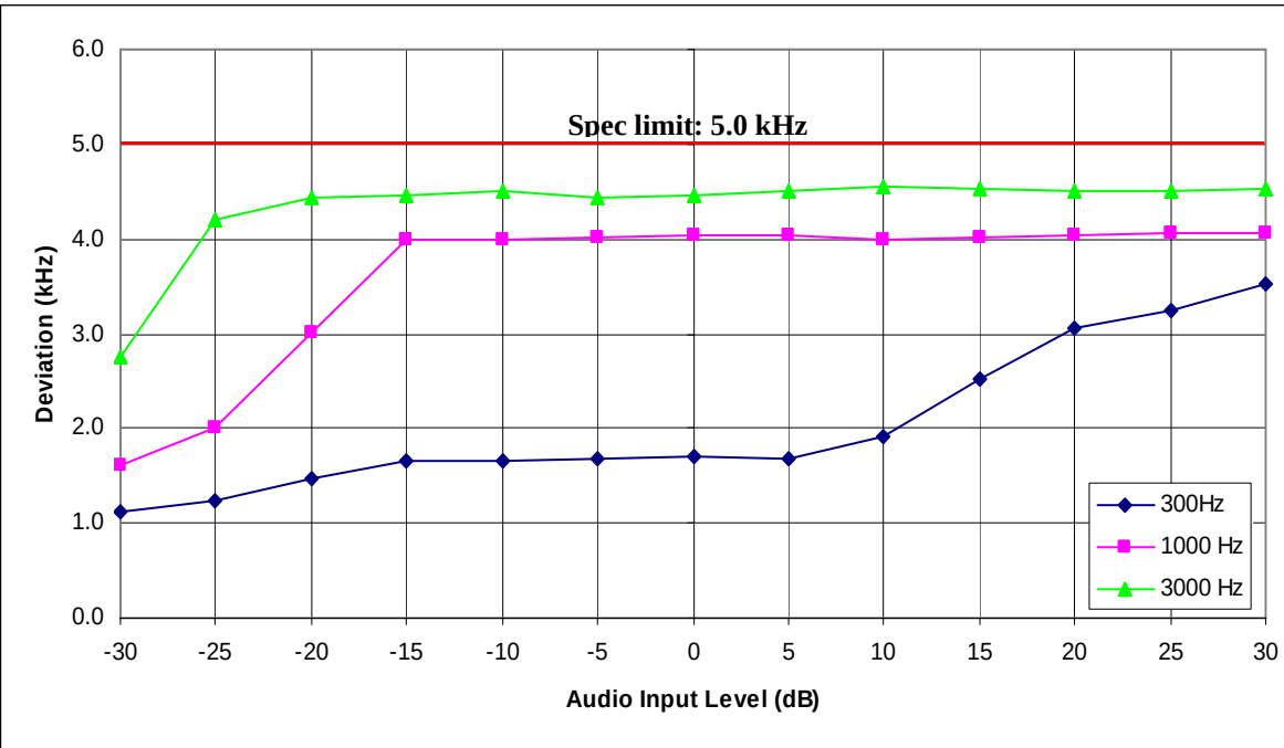
Figure 6D-6: 25 kHz Channel Spacing, 156.675 MHz, Digital Private Line (DPL) Mode
