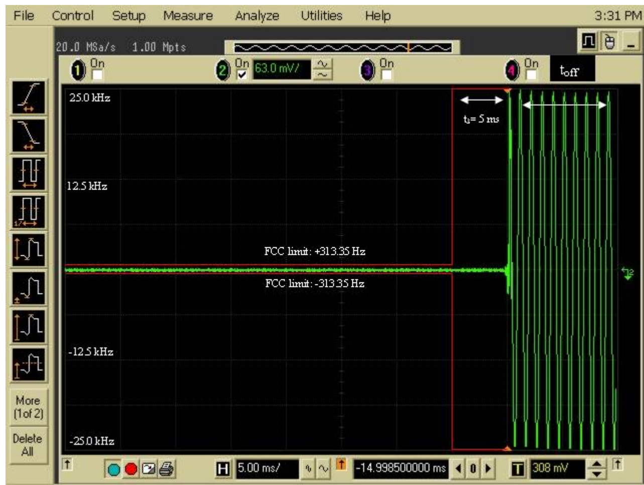
Figure 6I-8: 1.6 Watt, 25 kHz De-Key Decay Time
