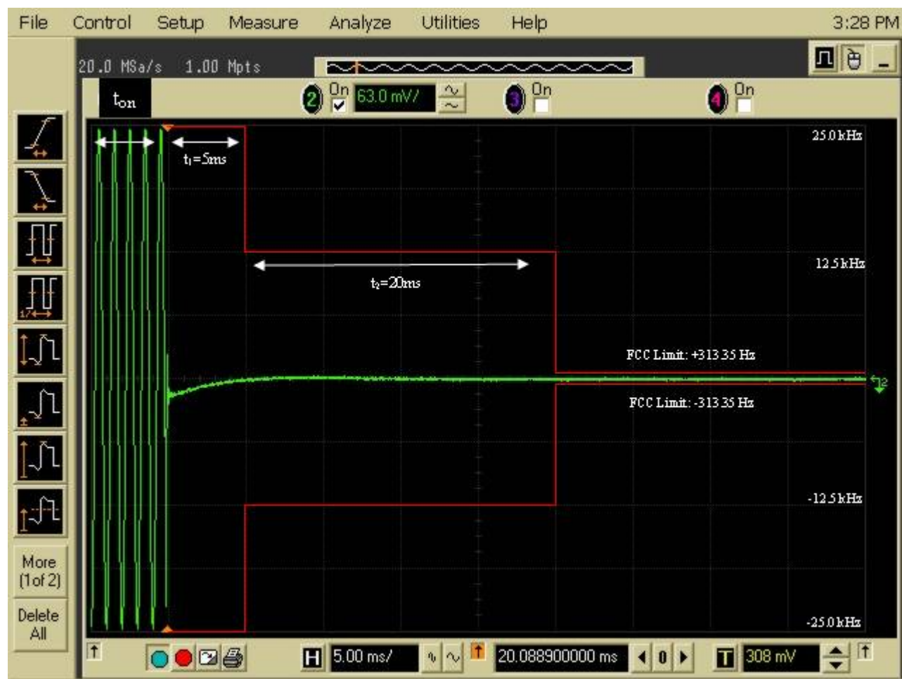
Figure 6I-3: 2.8 Watts, 25 kHz Key-Up Attack Time
