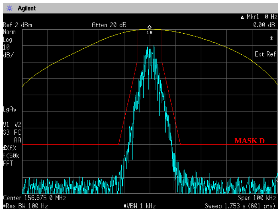
Figure 6E-7: 12.5 kHz Channel Spacing, 156.675 MHz, APCO25 Digital Data (8K10F1D), 8K10F1D
