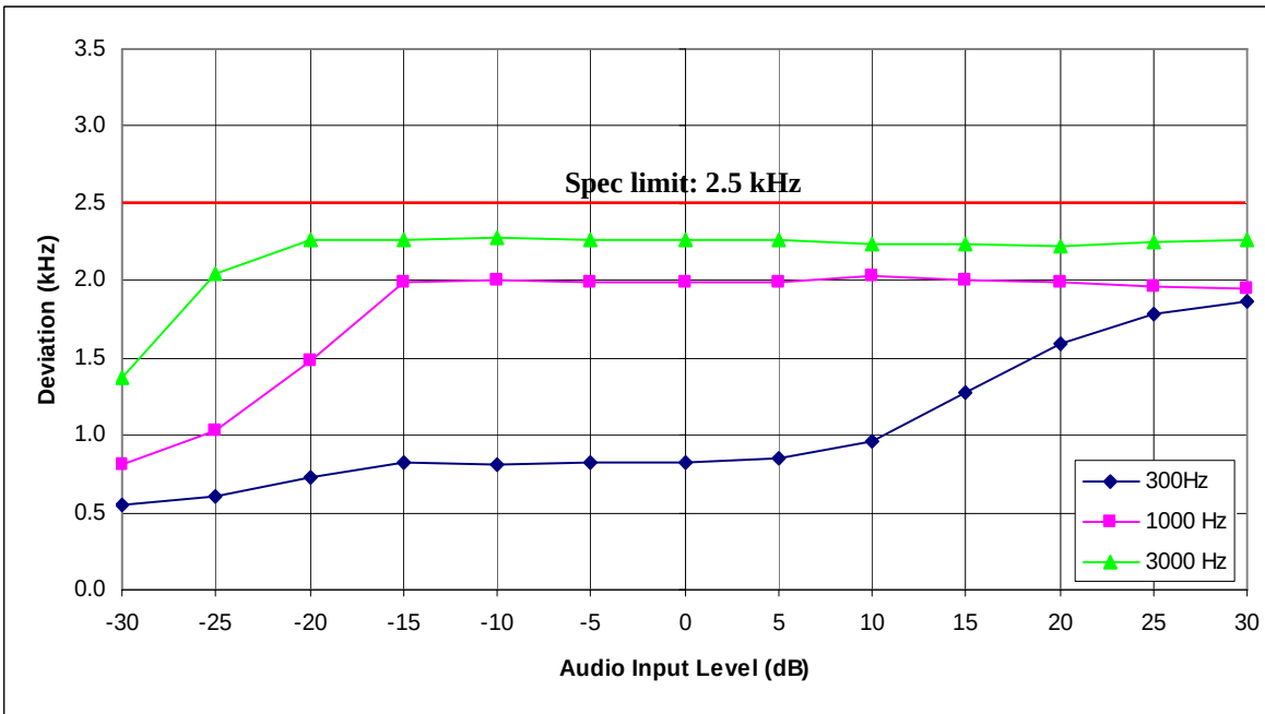
Figure 6D-2: 12.5 kHz Channel Spacing, 156.675 MHz, Tone Private Line (TPL) Mode
