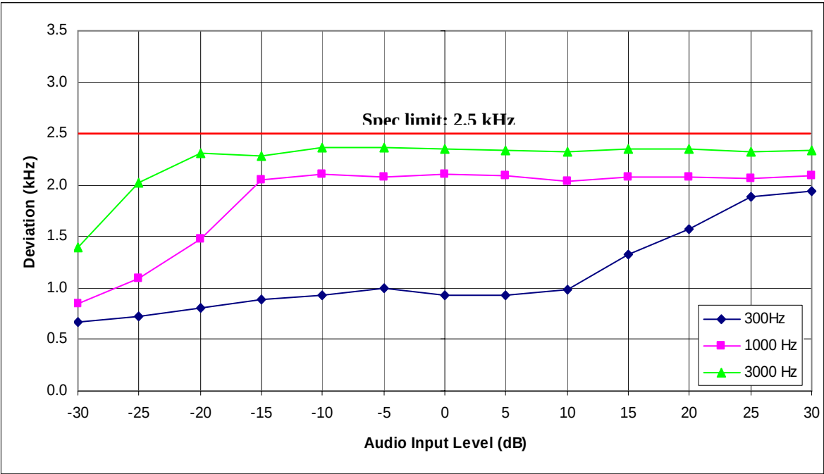
Figure 6D-3: 12.5 kHz Channel Spacing, 156.675 MHz, Digital Private Line (DPL) Mode
