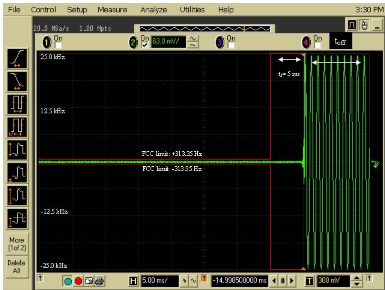
Figure 6I-6: 1.6 Watt, 12.5 kHz De-Key Decay Time
