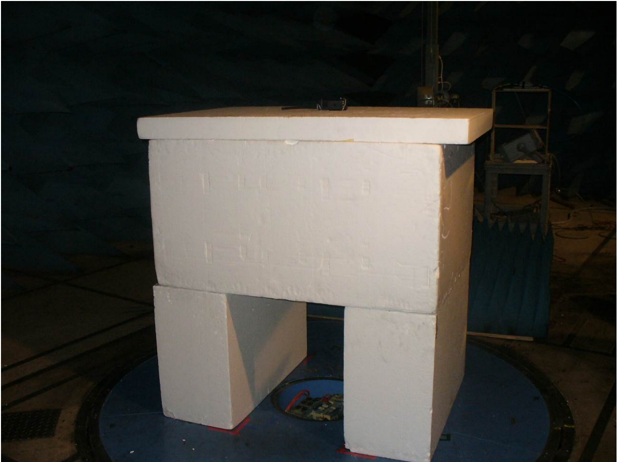
Figure 4: Radiated Emissions – Back View – EUT on Side
