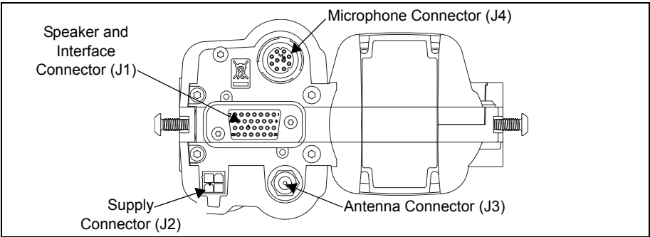
Figure 5: Console Connections
