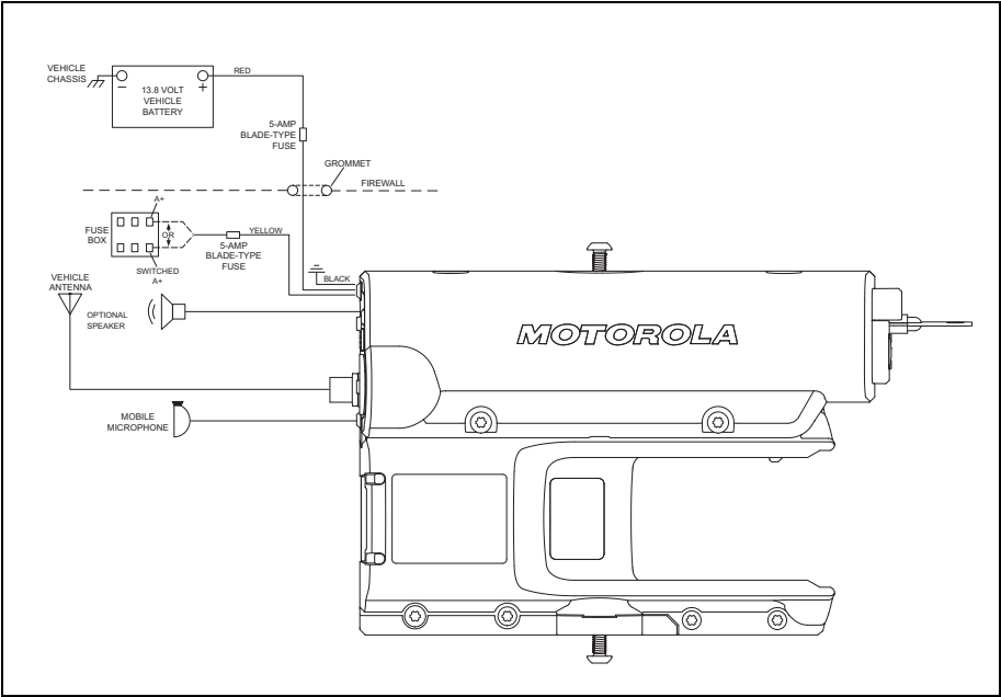
Figure 6: Console Cabling
