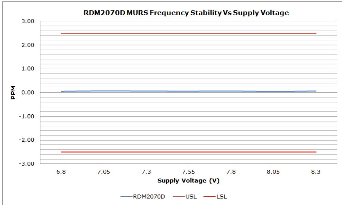
Figure 6E-2: Frequency Stability over Supply Voltage
