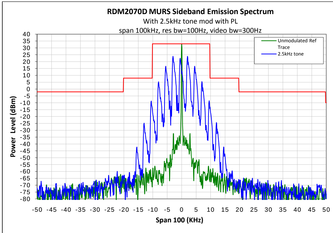
Figure 6C-6: Emission Mask Spectrum 25 KHz with PL
