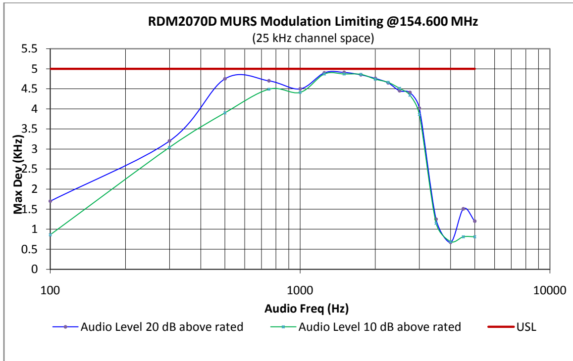
Figure 6B-2: Modulation limiting for 25 KHz band.
