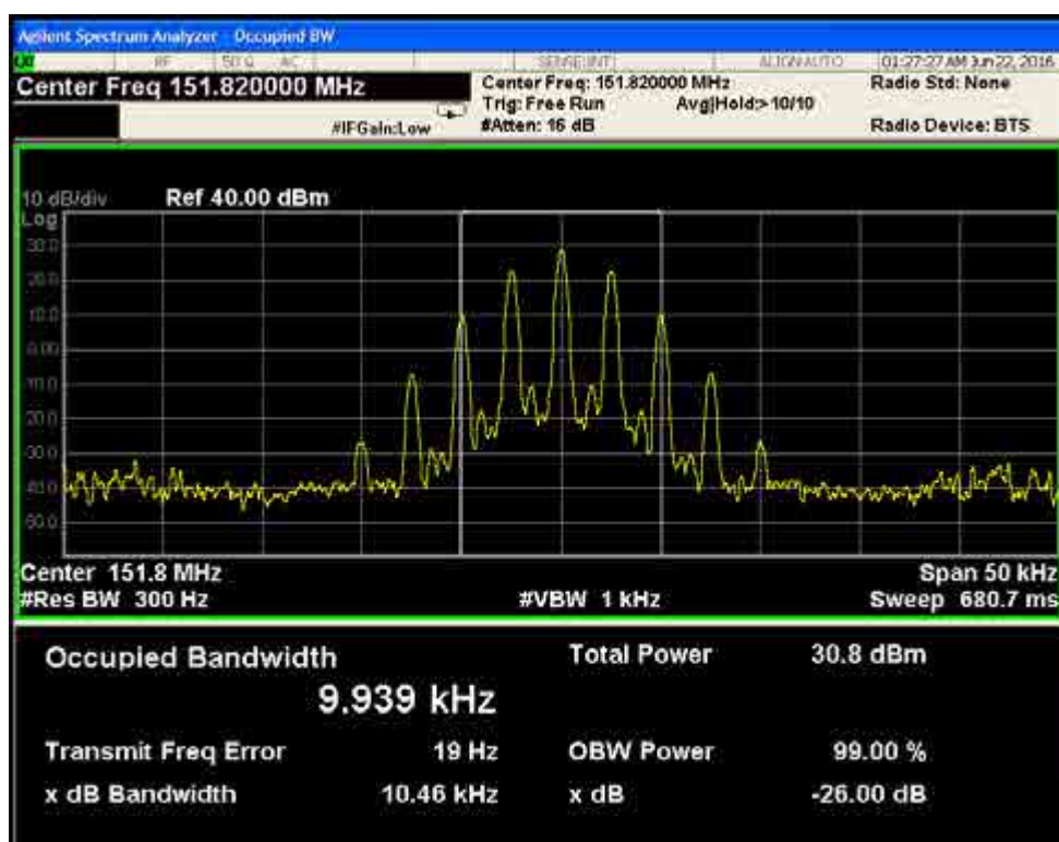
Figure 6C-1: 151.820 MHz, 12.5 KHz Band, 99% Occupied BW
