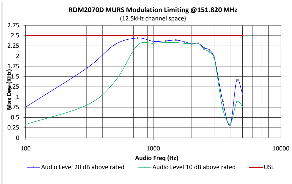
Figure 6B-1: Modulation limiting for 12.5 KHz band.
