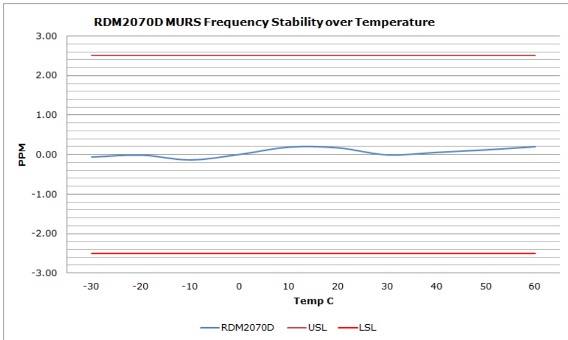
Figure 6E-1: Frequency Stability over Temperature
