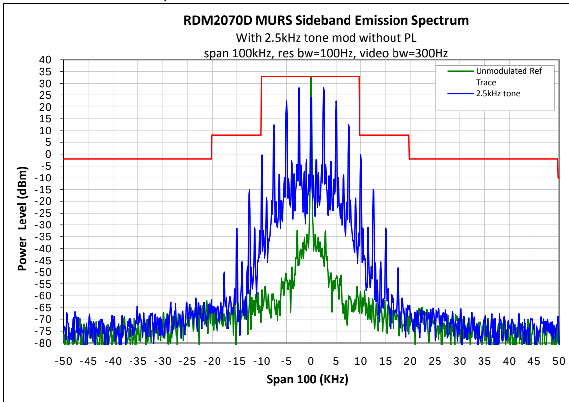
Figure 6C-5: Emission Mask Spectrum 25 KHz without PL
