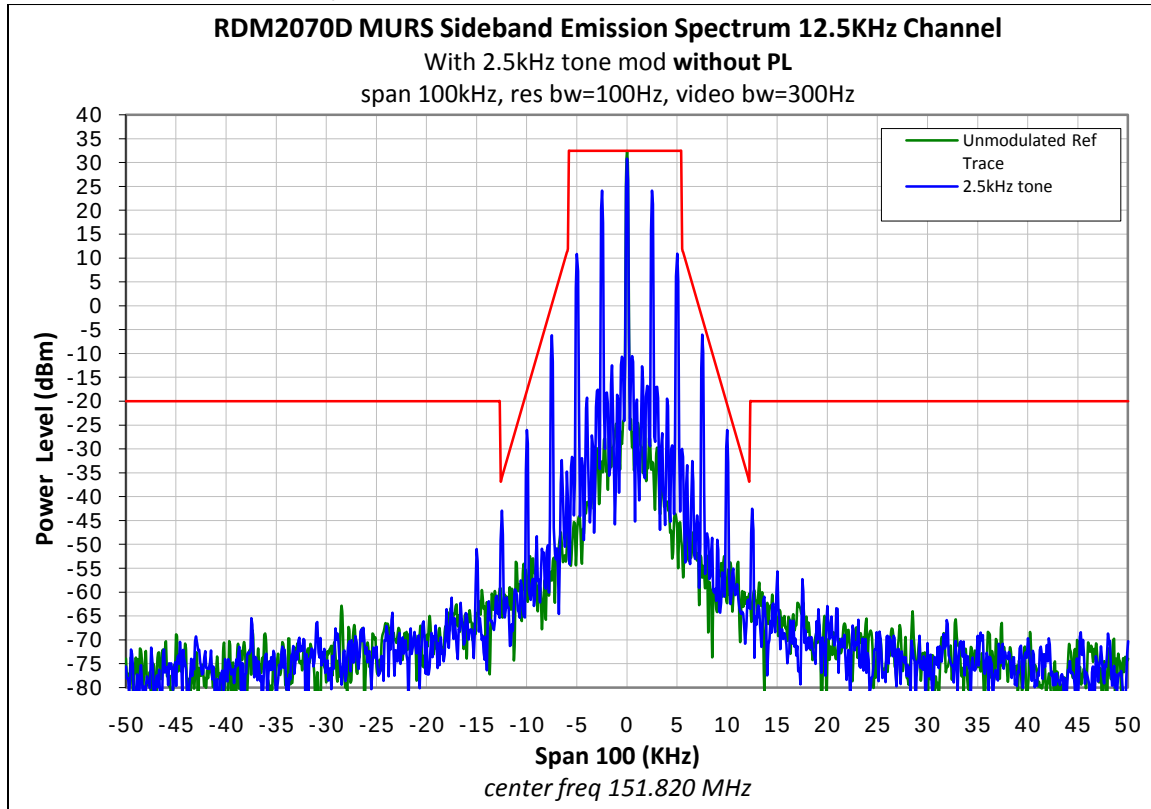
Figure 6C-3: Emission Mask Spectrum 12.5 KHz without PL
