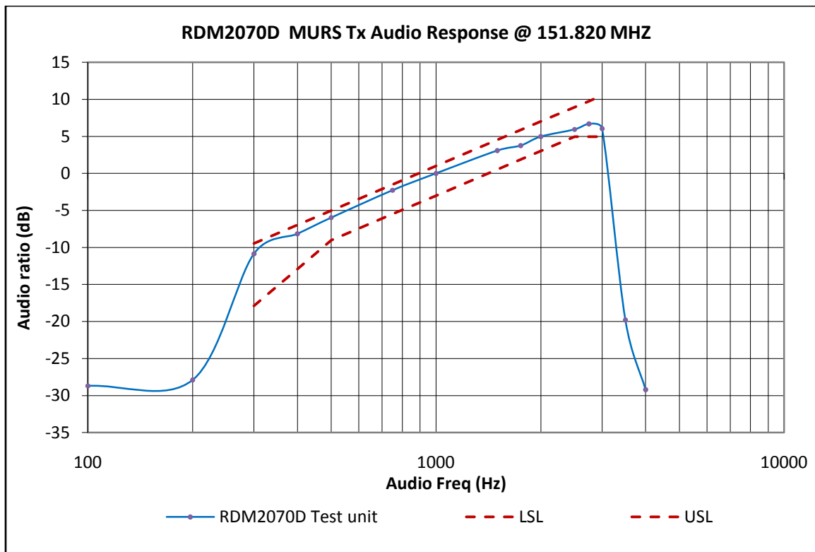
Figure 6B-3: Audio Response.
