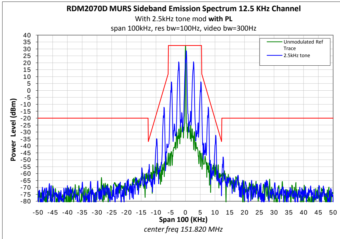
Figure 6C-4: Emission Mask Spectrum 12.5 KHz with PL
