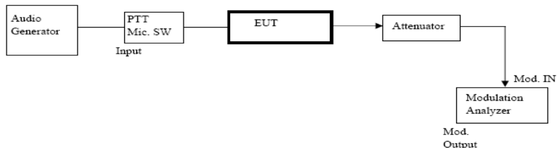
Figure 1. Modulation limiting setup
