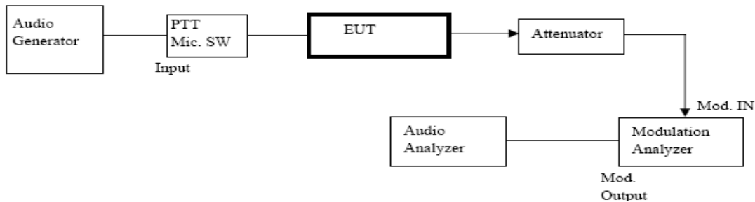
Figure 2. Audio Response setup
