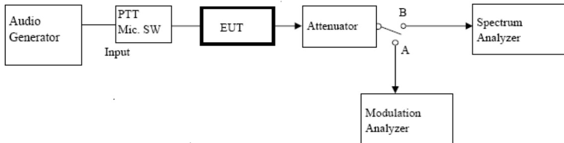
Figure 3. Occupied Bandwidth and Emission Mask Setup
