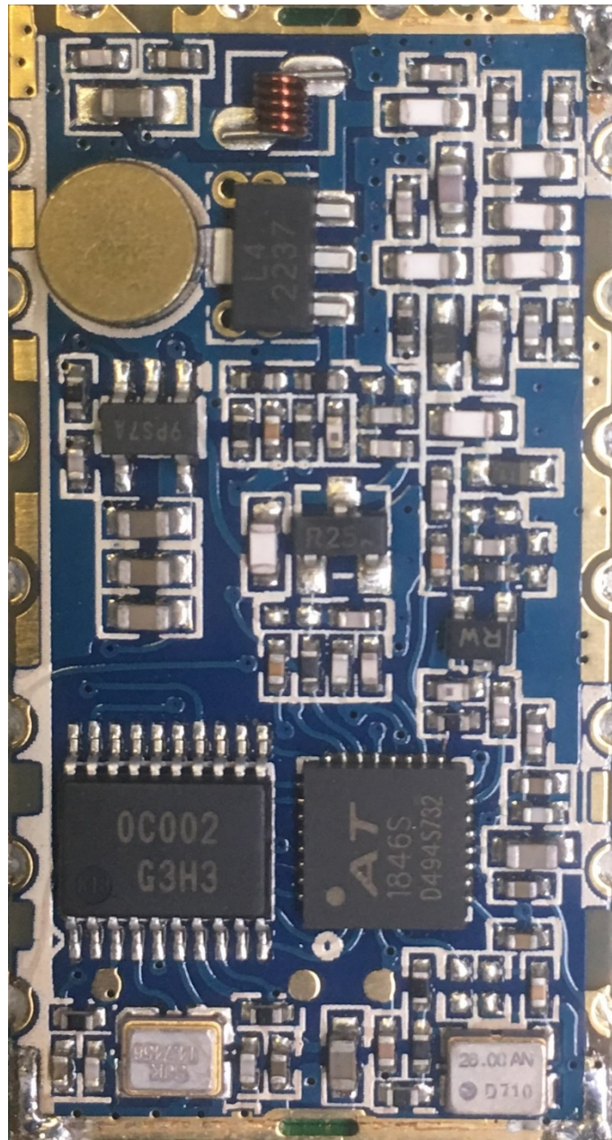
RF Module Shield Removed
