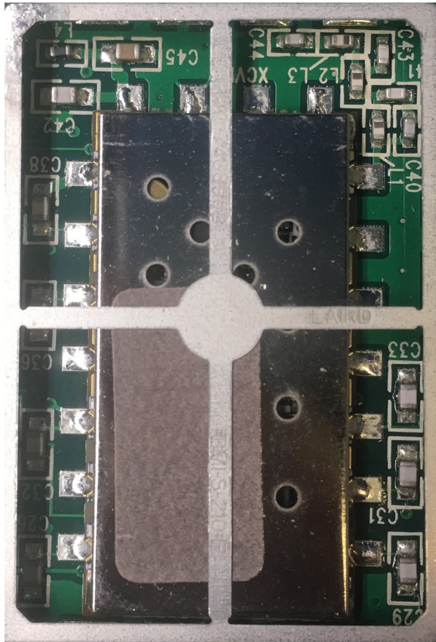
Outer Shield Removed (Close Up)
