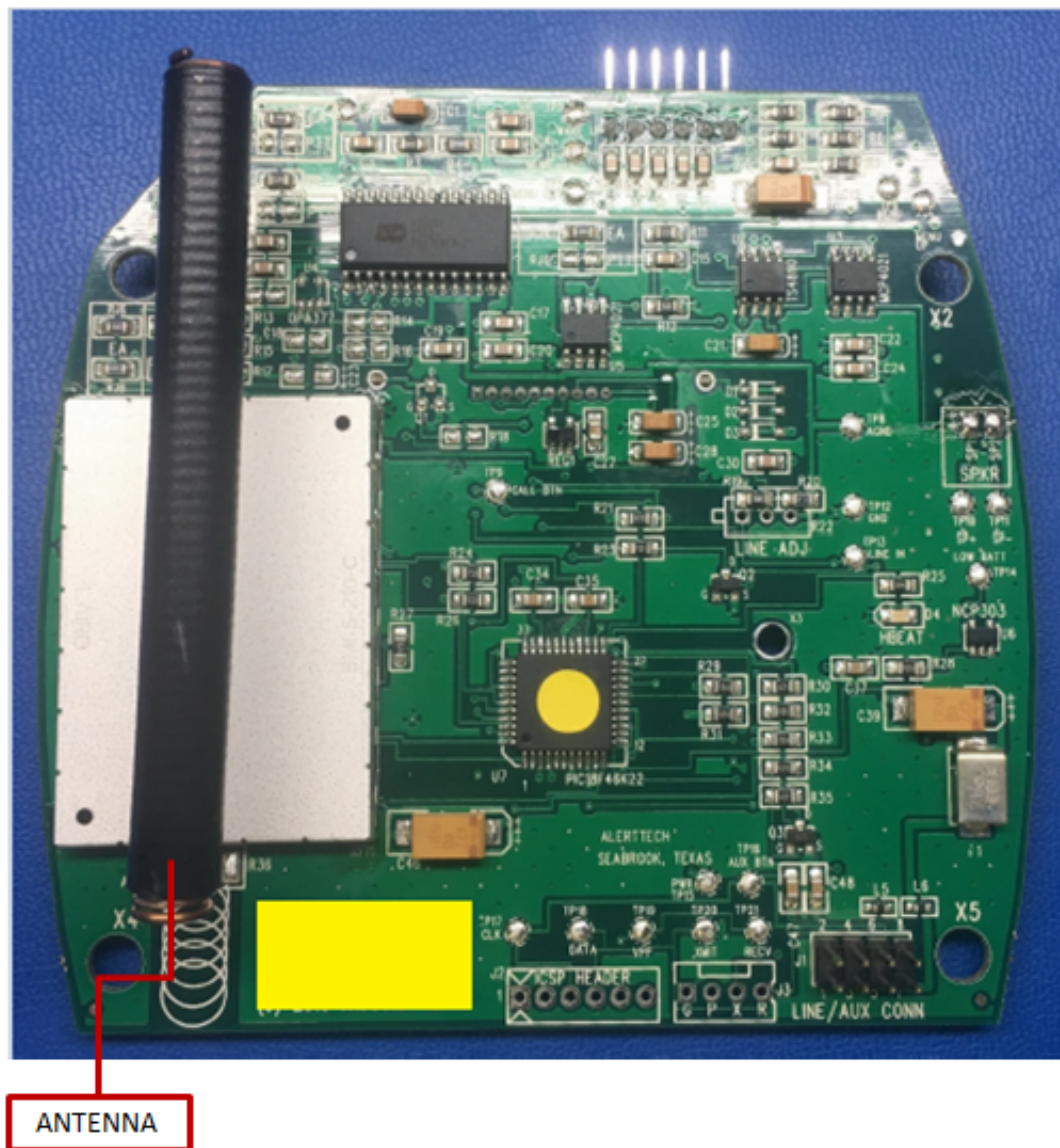
Board Side 1 (With antenna)
