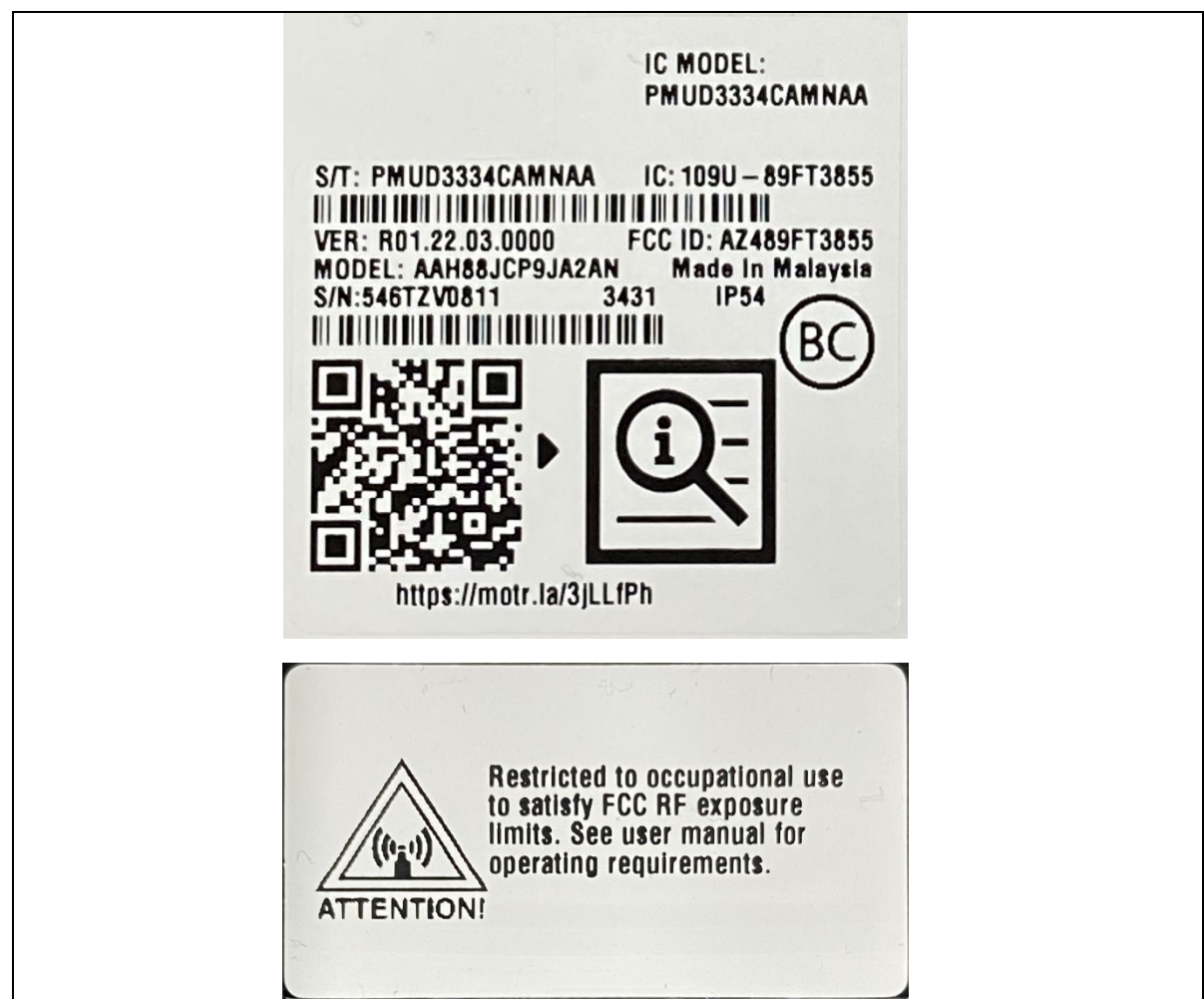
Figure 1: FCC/IC Label for SL300 136-174MHz 2-3W DISPLAY
