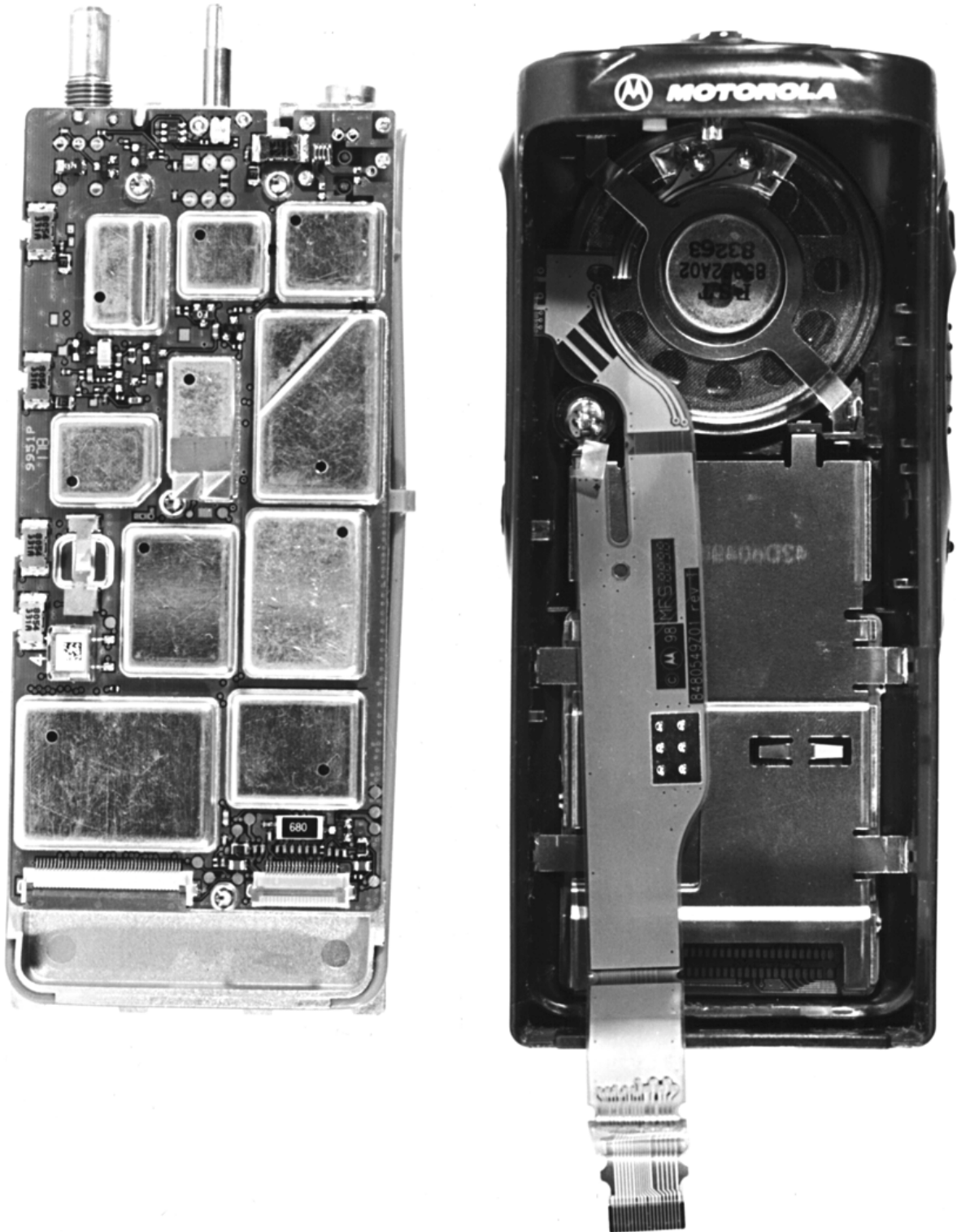
View With Front Housing Open up (GP328)
