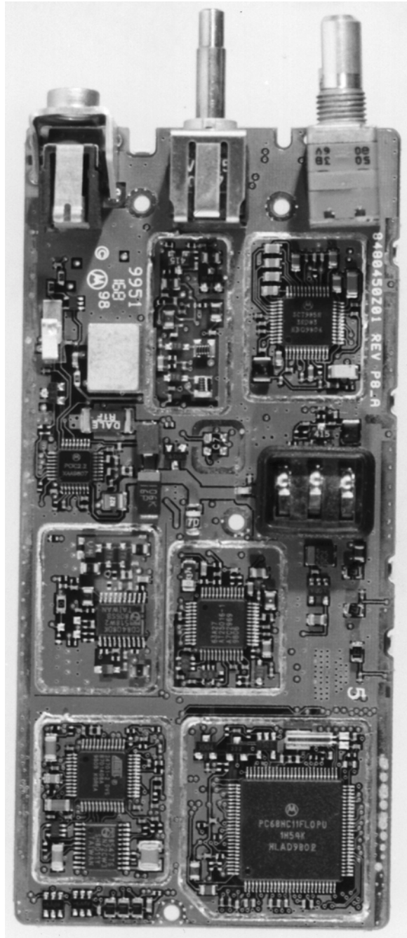
Bottom (Casting) Side Of RF/Controller Board With Shields Removed. (GP328 & GP338)
