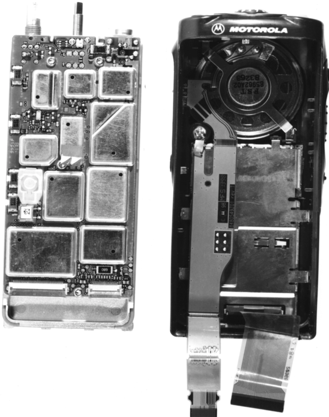
View With Front Housing Open up (GP338)
