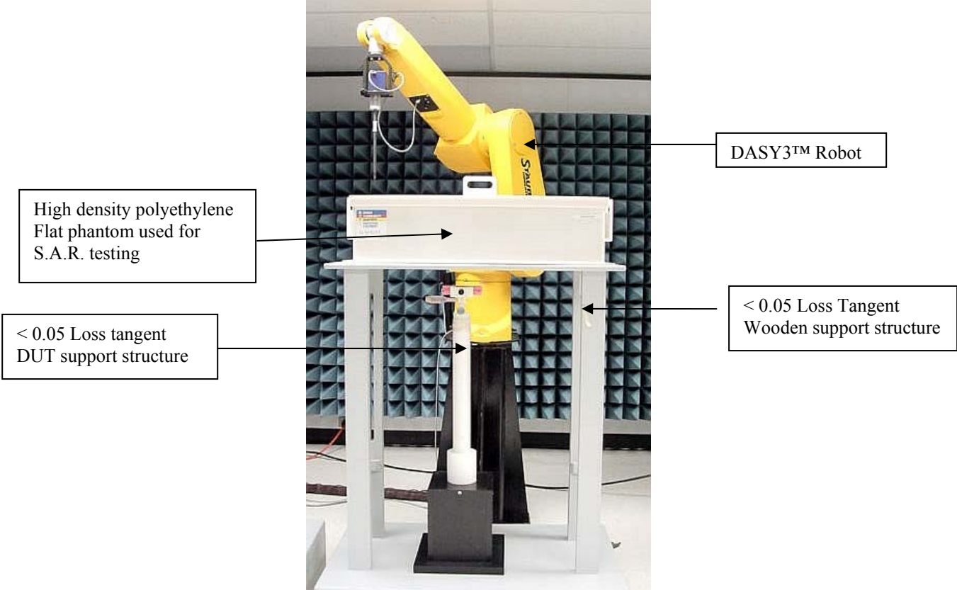
Figure 3: Robot Test System (Flat Phantom)
