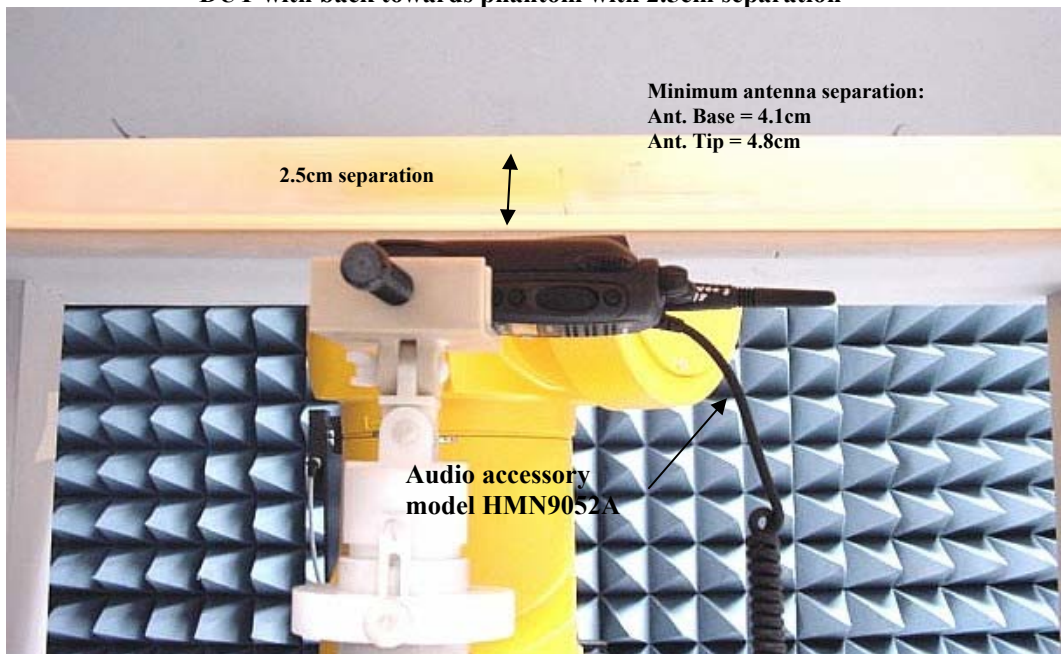
Figure 2. Assessment @ the Body DUT with back towards phantom with 2.5cm separation
