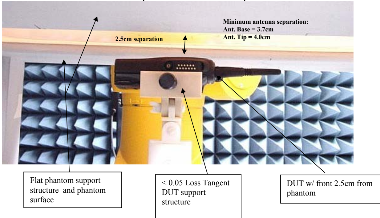
Figure 1: Highest S.A.R. Test Position (@ Face) DUT with front separated 2.5 cm from the flat phantom.
