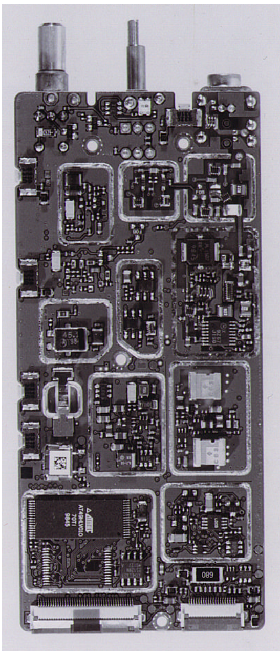
Top (Front Housing) Side Of RF/Controller Board With Shields Removed. (GP328 & GP338)
