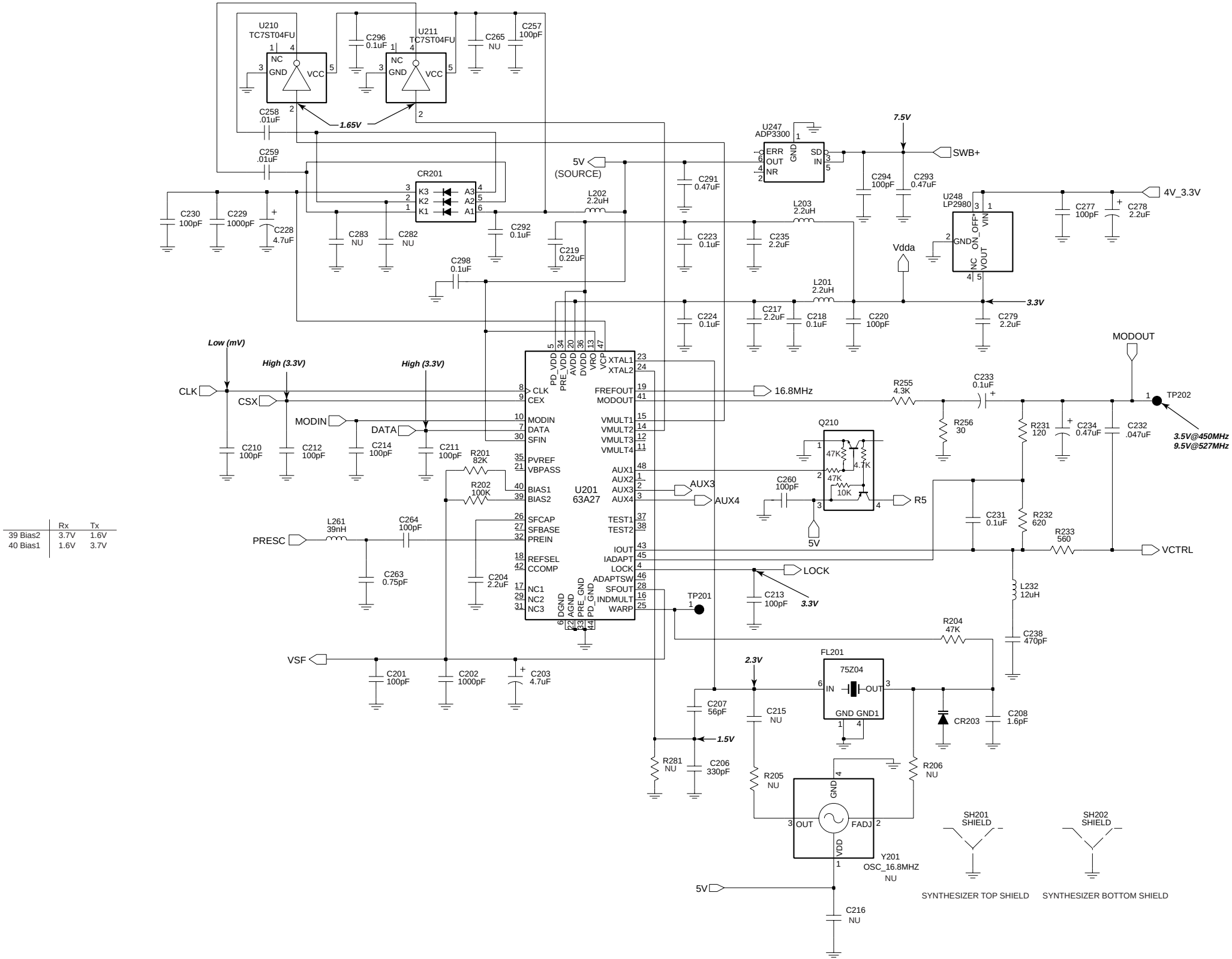
Figure 4-38: UHF Band 2 Synthesizer Schematic Diagram
