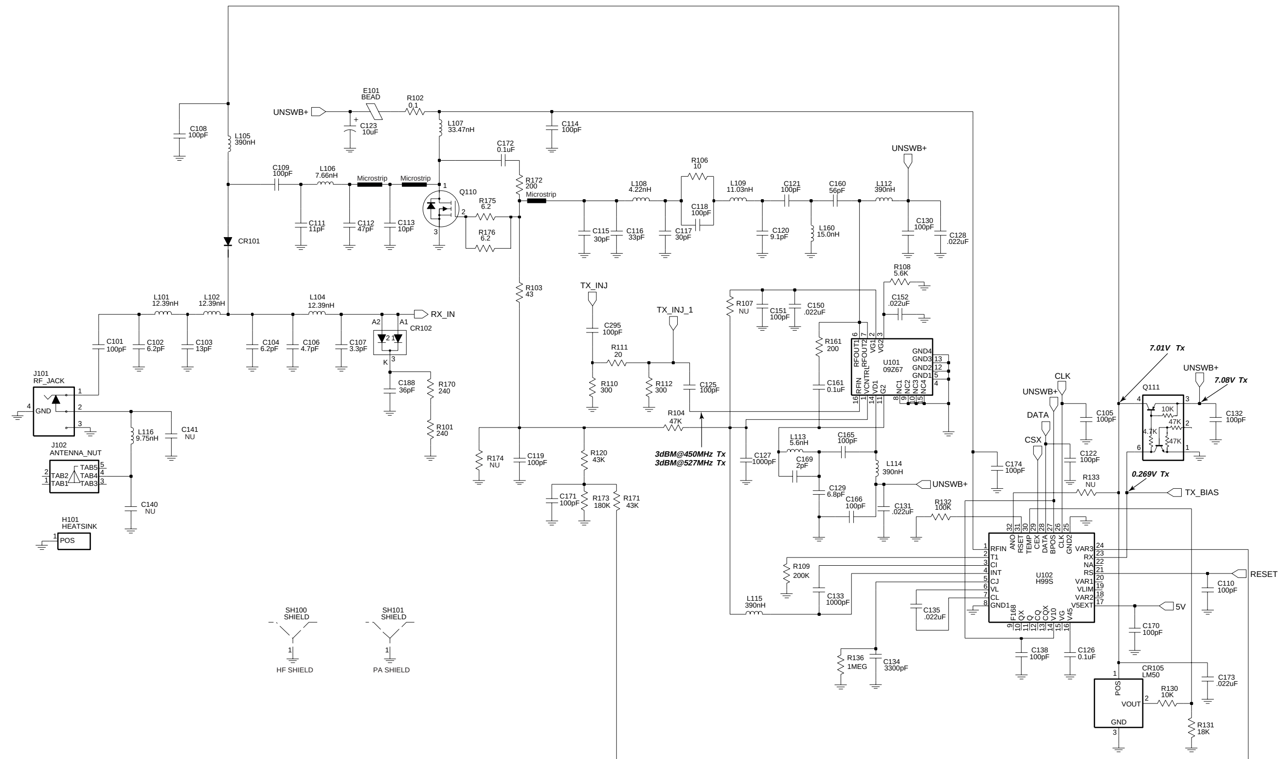
Figure 4-40: UHF Band 2 Transmitter Schematic Diagram
