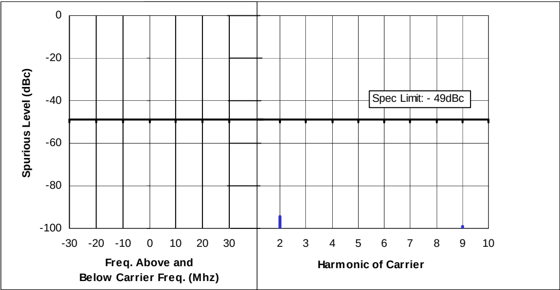
Figure 6F-3: Hi-Power, 511.975 MHz, 25 kHz Channel Spacing
