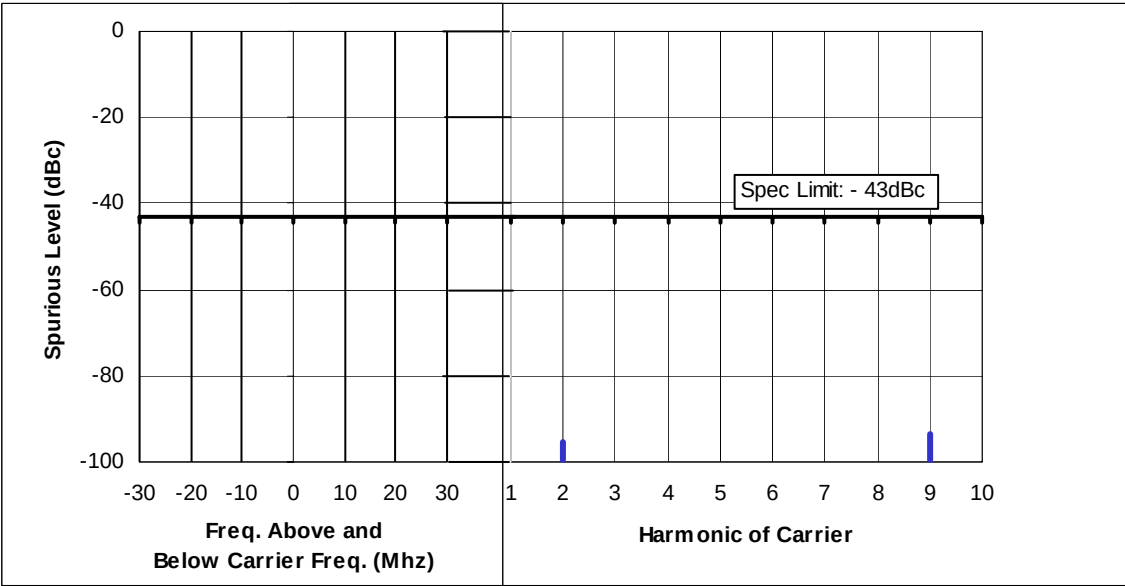
Figure 6F-6: Lo-Power, 511.975 MHz, 25 kHz Channel Spacing
