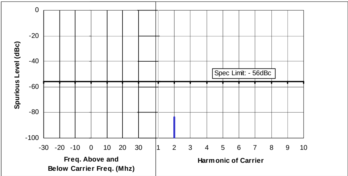
Figure 6F-8: Hi-Power, 481.050 MHz, 12.5 kHz Channel Spacing
