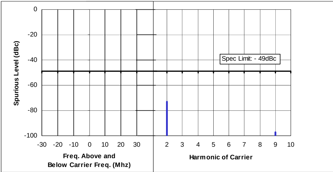
Figure 6F-1: Hi-Power, 450.025 MHz, 25 kHz Channel Spacing
