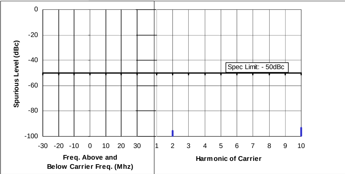
Figure 6F-12: Lo-Power, 511.975 MHz, 12.5 kHz Channel Spacing
