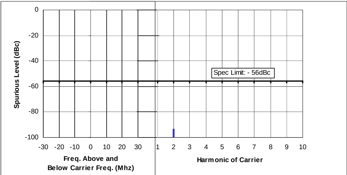
Figure 6F-9: Hi-Power, 511.975 MHz, 12.5 kHz Channel Spacing
