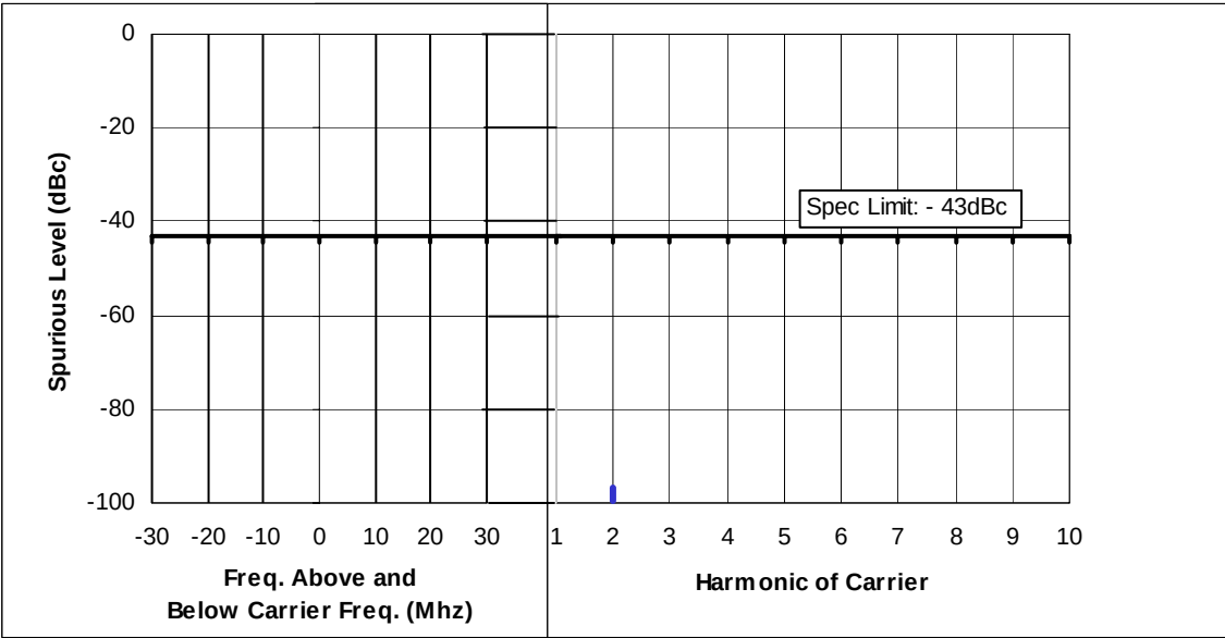
Figure 6F-5: Lo-Power, 481.050 MHz, 25 kHz Channel Spacing
