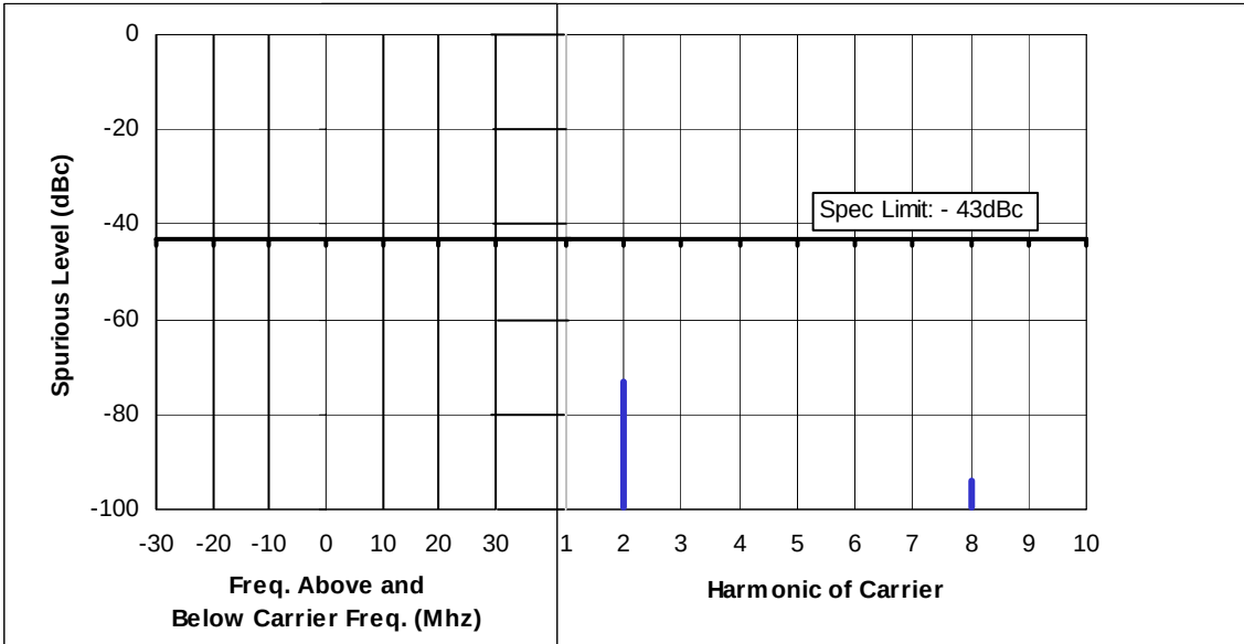
Figure 6F-4: Lo-Power, 450.025 MHz, 25 kHz Channel Spacing
