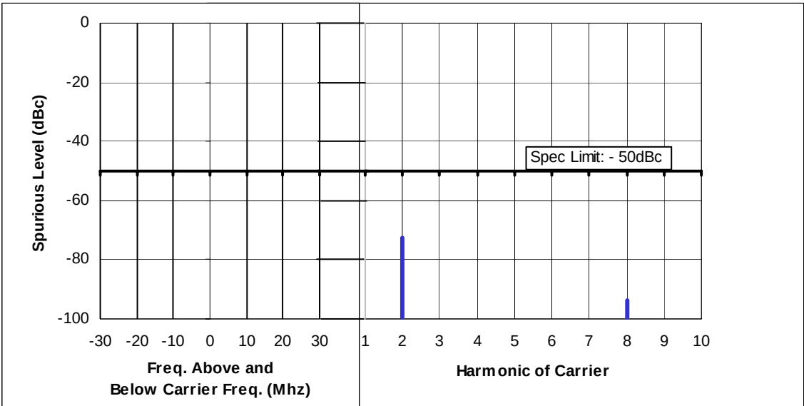
Figure 6F-10: Lo-Power, 450.025 MHz, 12.5 kHz Channel Spacing
