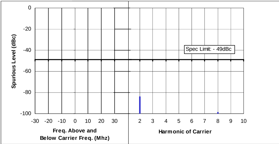
Figure 6F-2: Hi-Power, 481.050 MHz, 25 kHz Channel Spacing
