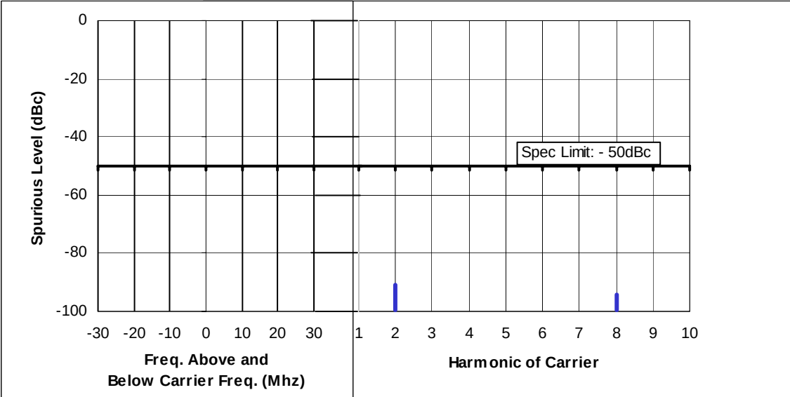
Figure 6F-11: Lo-Power, 481.050 MHz, 12.5 kHz Channel Spacing
