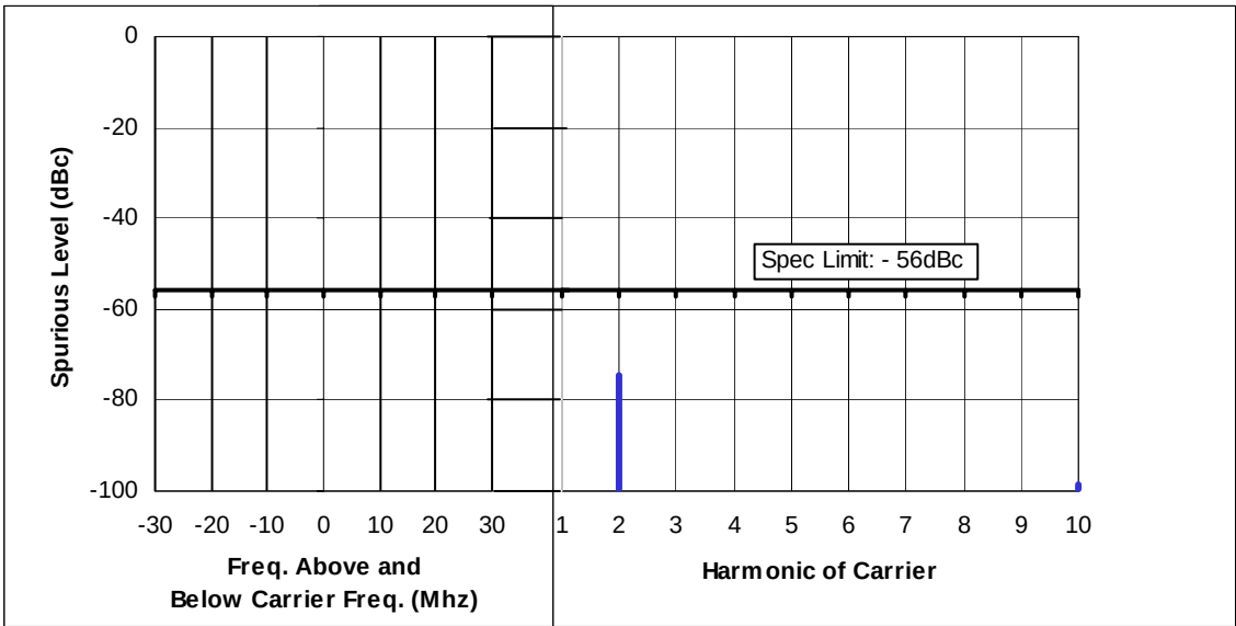
Figure 6F-7: Hi-Power, 450.025 MHz, 12.5 kHz Channel Spacing
