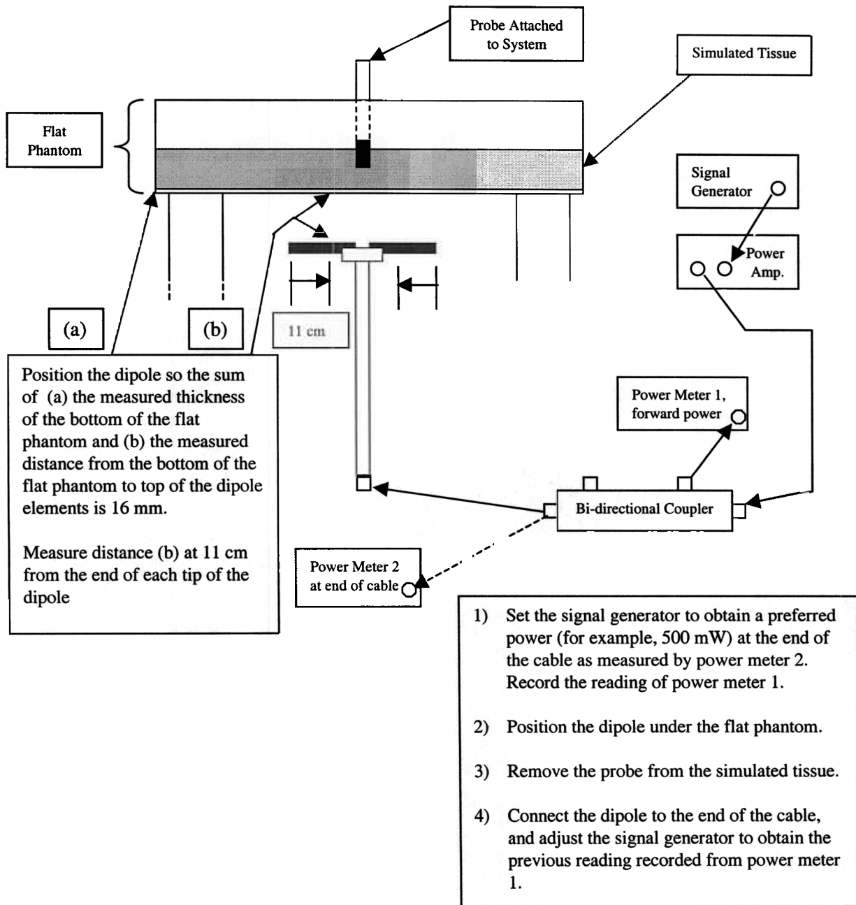
Figure 1. Flat Phantom System Validation Setup
