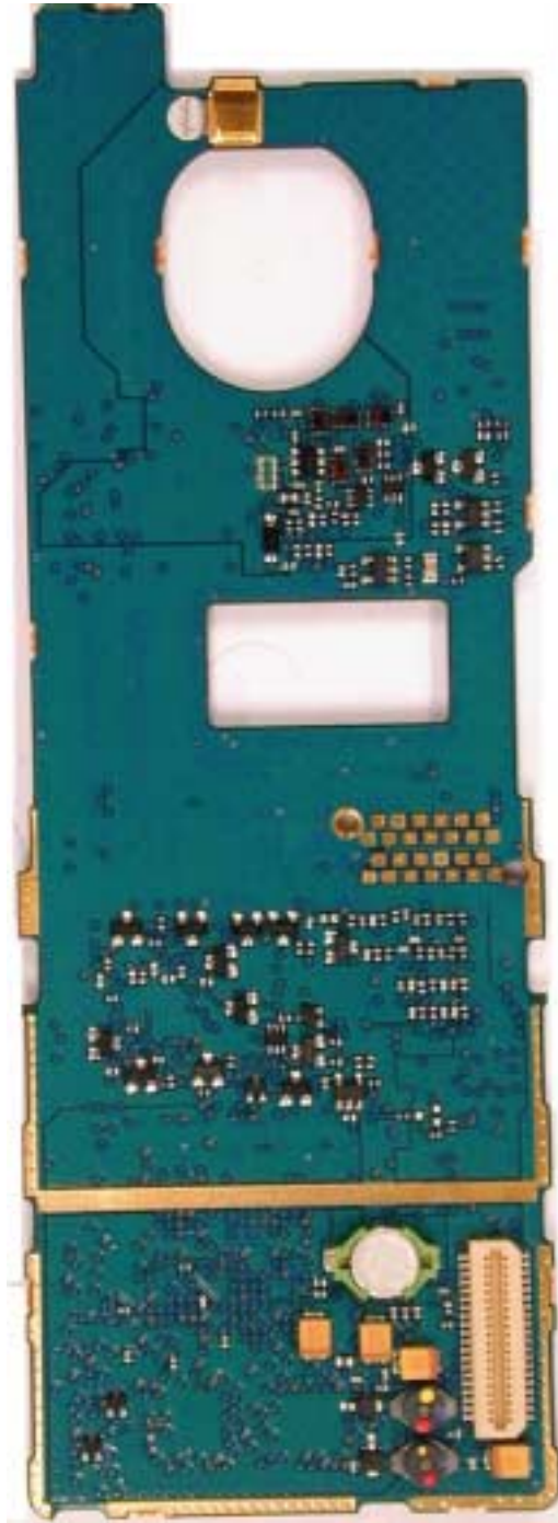
Vocon board (Bottom))
