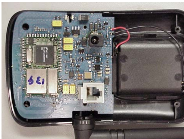
Component side Base
