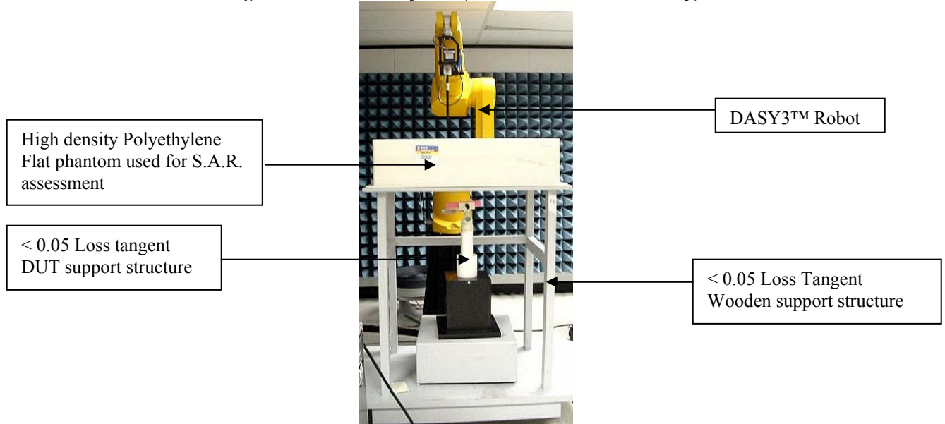
Figure 9: Robot Test System (Flat Phantom used for body)
