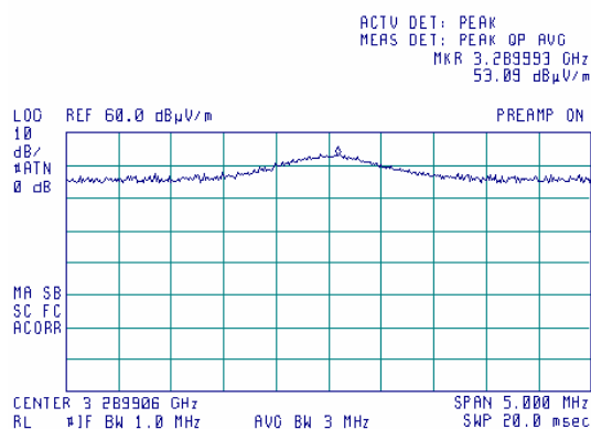
Plot 7.6.46 Radiated emission measurements at the 7 th harmonic
