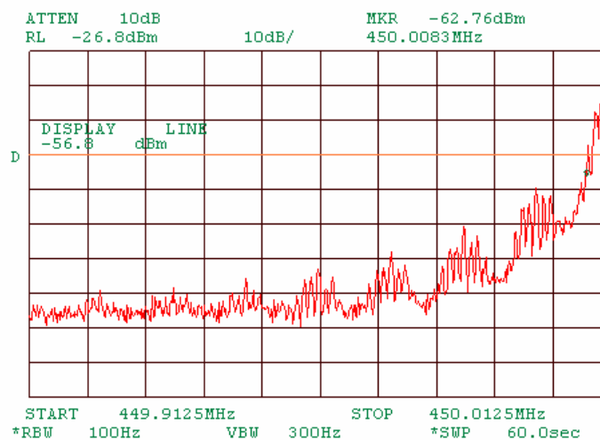
Plot 7.5.1 Band edge emission test results at low carrier frequency low side
