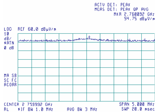
Plot 7.6.42 Radiated emission measurements at the 6 th harmonic
