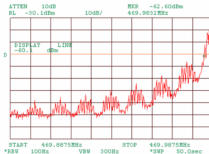
Plot 7.5.6 Band edge emission test results at high carrier frequency high side
