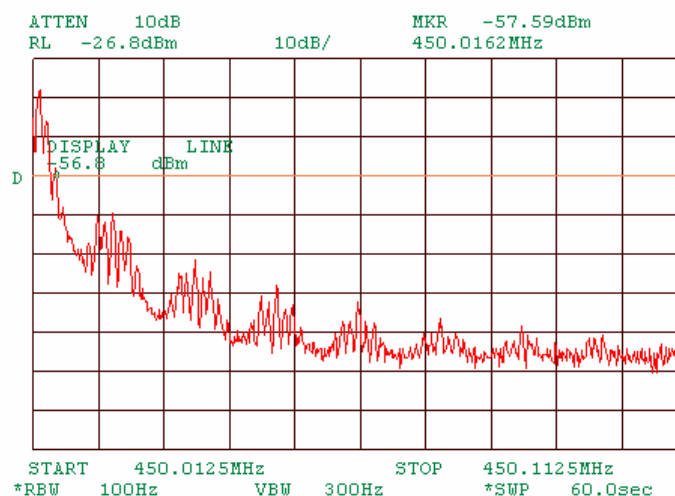
Plot 7.5.2 Band edge emission test results at low carrier frequency high side
