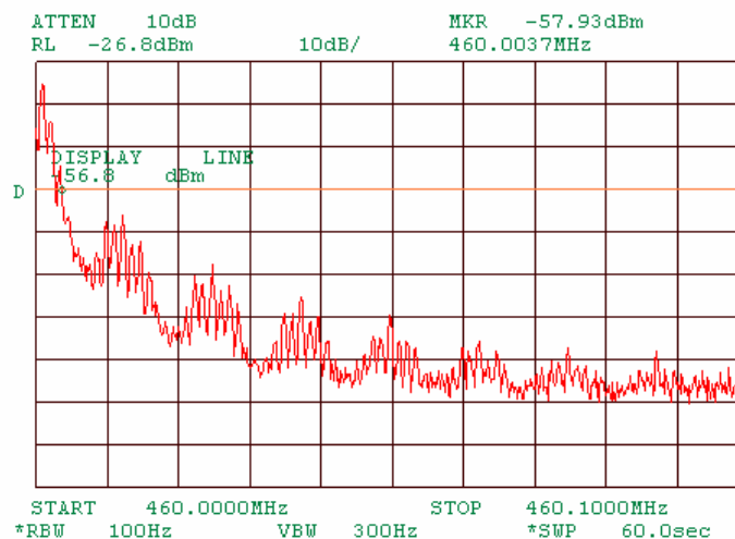
Plot 7.5.4 Band edge emission test results at mid carrier frequency high side
