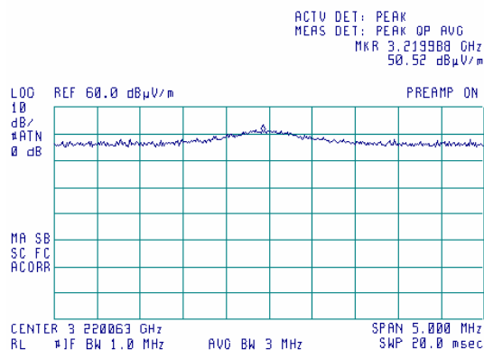
Plot 7.6.48 Radiated emission measurements at the 7 th harmonic
