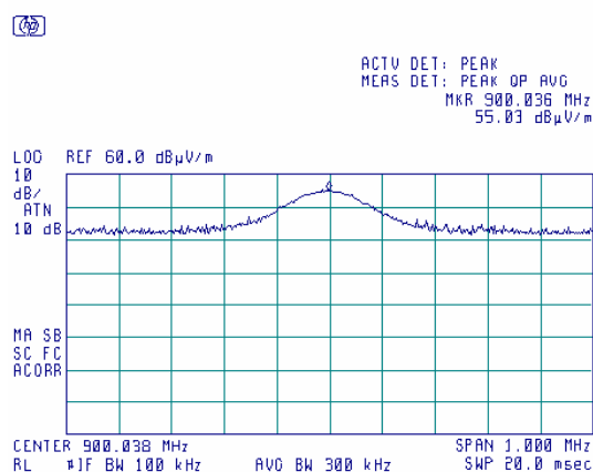
Plot 7.6.14 Radiated emission measurements at the 2 nd harmonic
