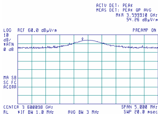
Plot 7.6.50 Radiated emission measurements at the 8 th harmonic
