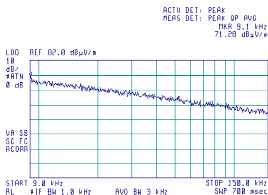
Plot 7.6.2 Radiated emission measurements in 9 - 150 kHz range
