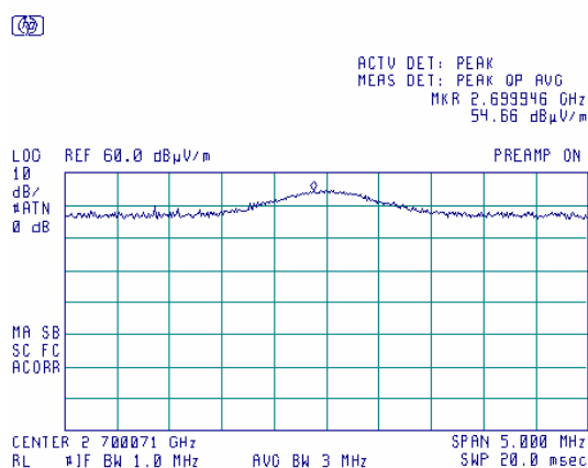
Plot 7.6.38 Radiated emission measurements at the 6 th harmonic
