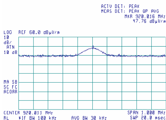
Plot 7.6.18 Radiated emission measurements at the 2 nd harmonic
