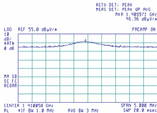
Plot 7.6.22 Radiated emission measurements at the 3 rd harmonic
