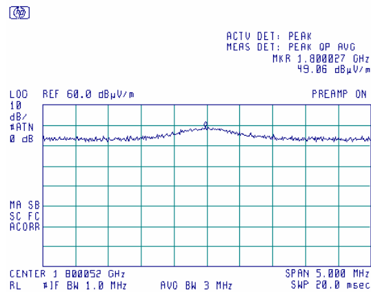
Plot 7.6.26 Radiated emission measurements at the 4 th harmonic
