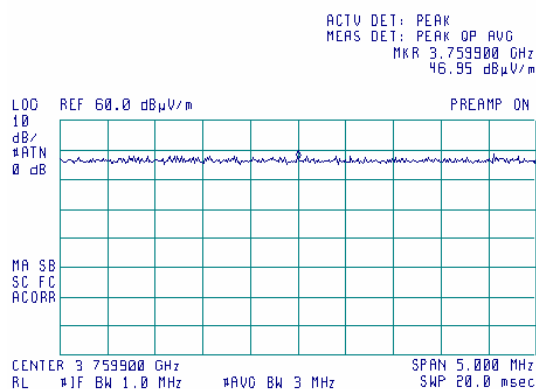
Plot 7.6.52 Radiated emission measurements at the 8 th harmonic
