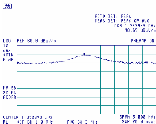
Plot 7.6.20 Radiated emission measurements at the 3 rd harmonic
