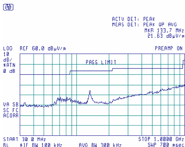
Plot 7.7.2 Radiated emission measurements in 30- 1000 MHz range, horizontal antenna polarization
