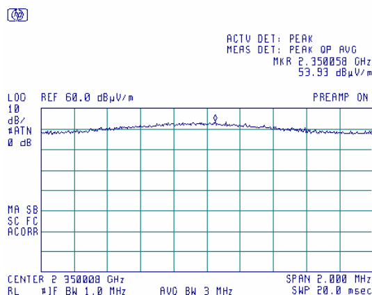
Plot 7.6.34 Radiated emission measurements at the 5 th harmonic
