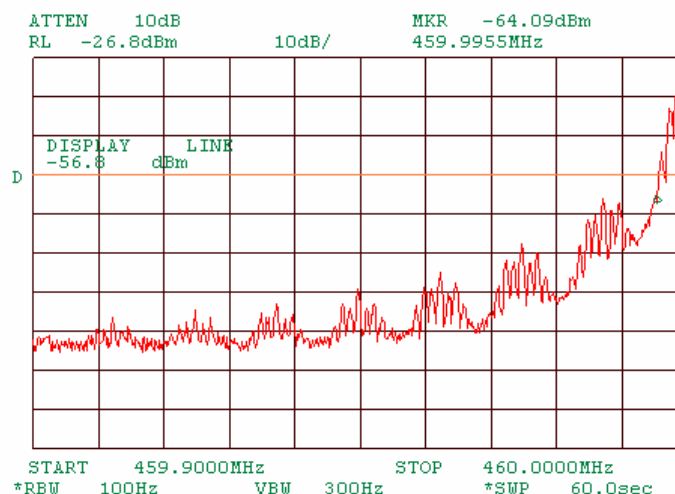
Plot 7.5.3 Band edge emission test results at mid carrier frequency low side
