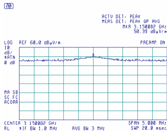
Plot 7.6.44 Radiated emission measurements at the 7 th harmonic
