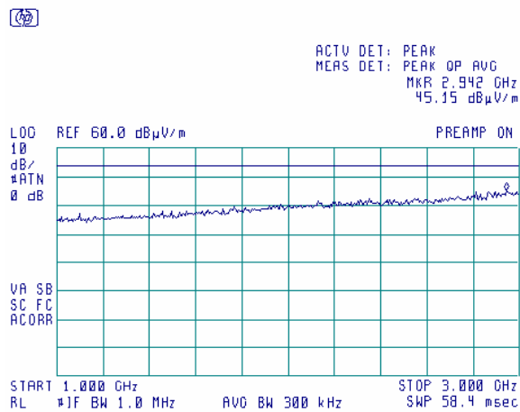
Plot 7.7.4 Radiated emission measurements in 1000 - 3000 MHz range, horizontal antenna polarization
