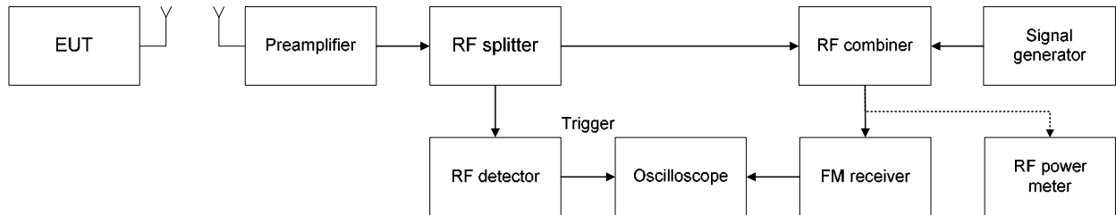
Figure 7.4.1 Transient frequency test setup
