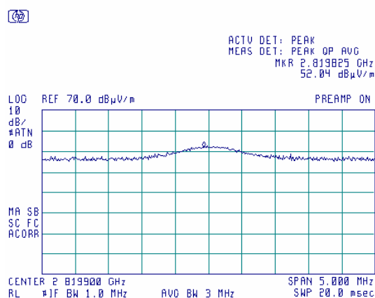
Plot 7.6.40 Radiated emission measurements at the 6 th harmonic
