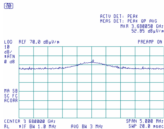
Plot 7.6.54 Radiated emission measurements at the 8 th harmonic
