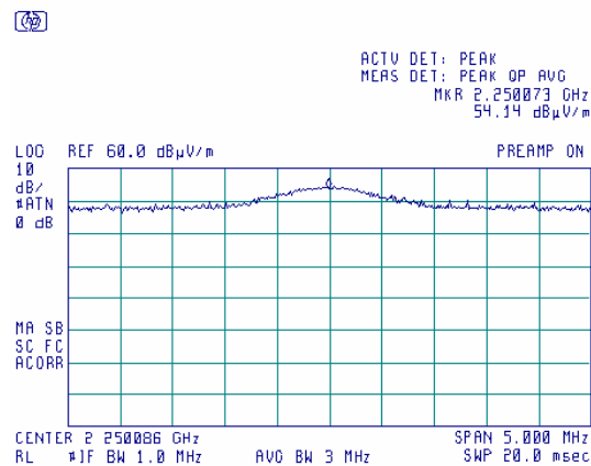
Plot 7.6.32 Radiated emission measurements at the 5 th harmonic
