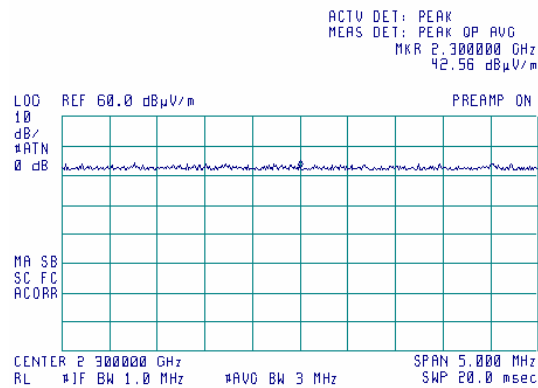
Plot 7.6.36 Radiated emission measurements at the 5 th harmonic
