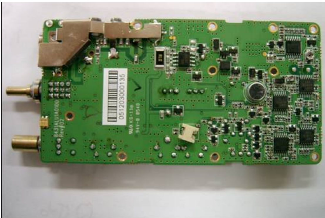
Figure 9-1: Top Side of PCB.
