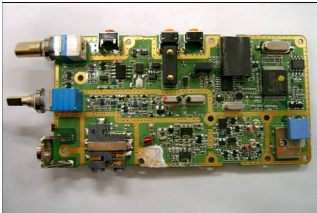
Figure 9-2: Bottom Side of PCB.
