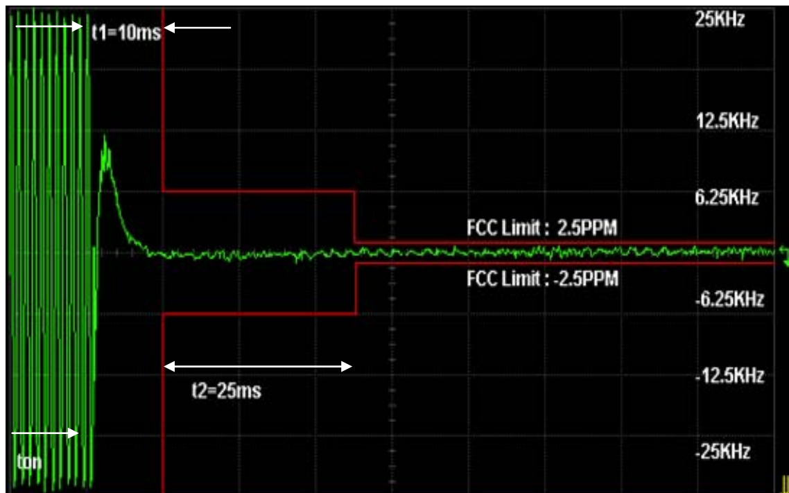
Figure 6I-5: 1 Watt, 12.5 kHz, 414.025 MHz, Key-Up Attack Time
