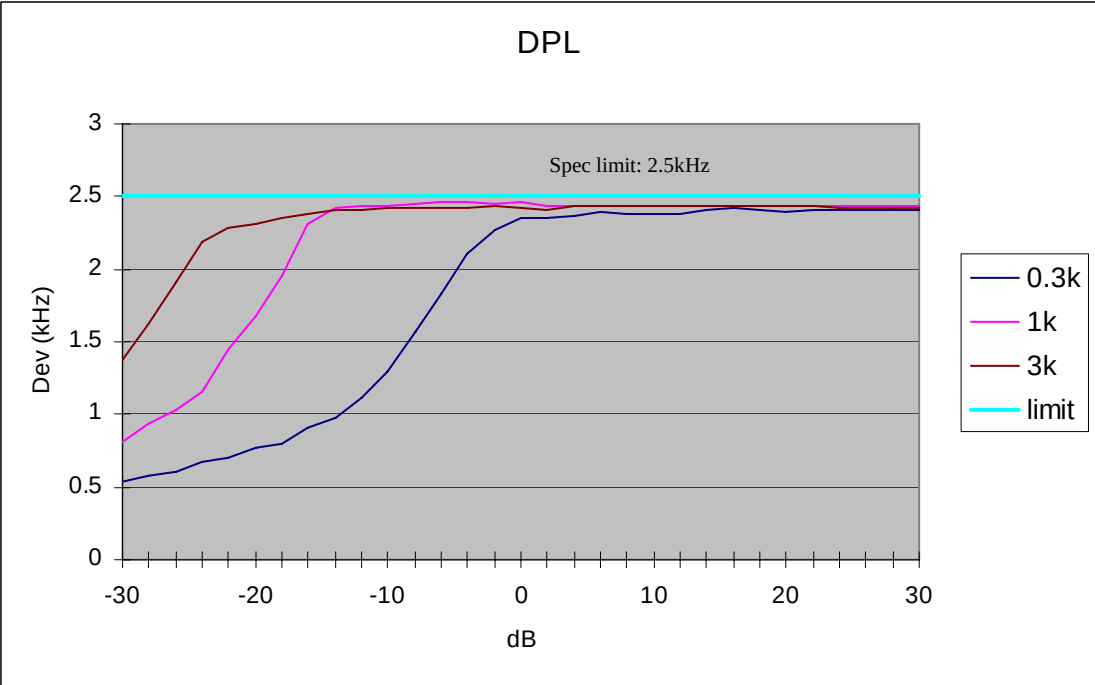
Figure 6D-3: 12.5 kHz Channel Spacing, 414.025 MHz, Digital Private Line (DPL) Mode
