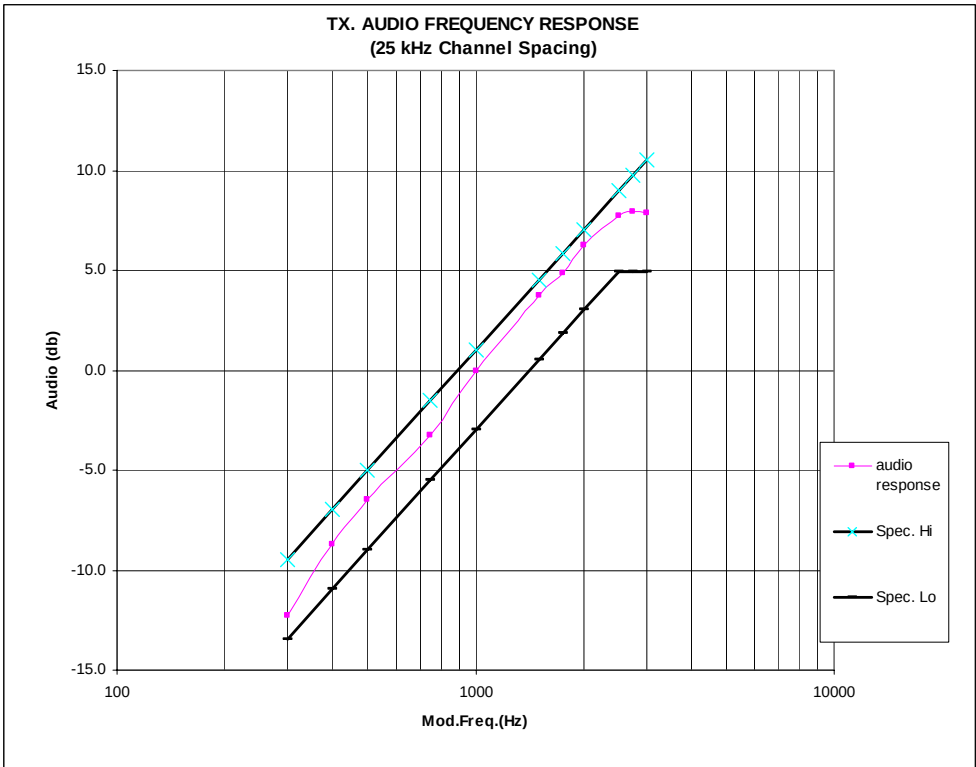
Figure 6B-2: 25 kHz Channel Spacing, 414.025 MHz, Transmit Audio Frequency Response
