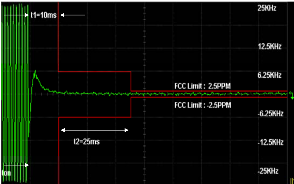
Figure 6I-1: 4 Watts, 12.5 kHz, 414.025 MHz, Key-Up Attack Time
