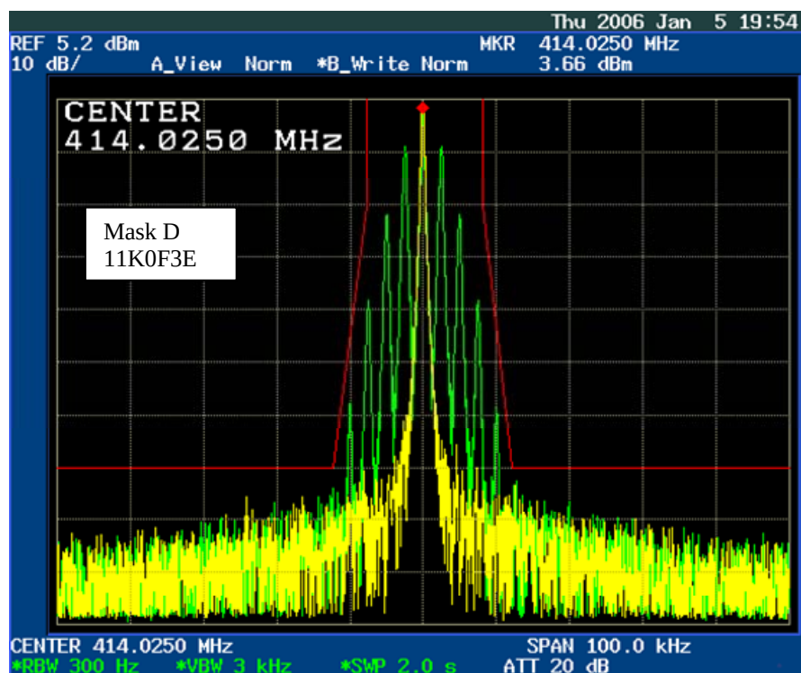
Figure 6E-1: 12.5 kHz Channel Spacing, 414.025 MHz, 2500 Hz Audio Modulation Only, Mask D 11K0F3E
