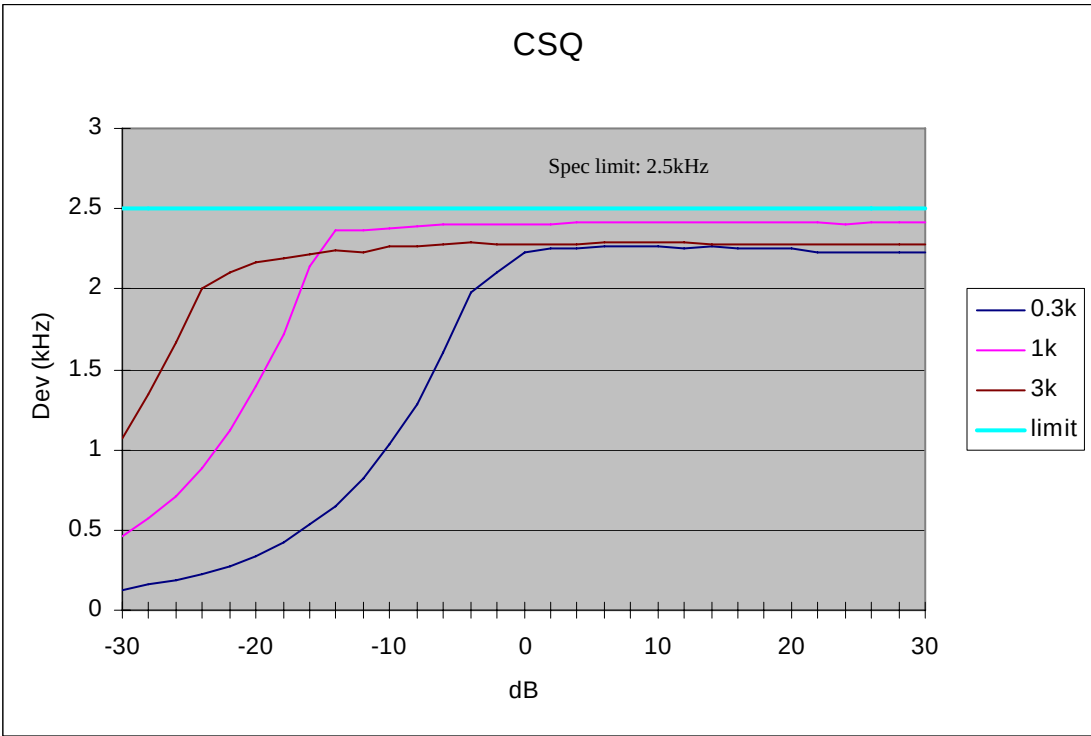
Figure 6D-1: 12.5 kHz Channel Spacing, 414.025 MHz, Carrier Squelch (CSQ) Mode
