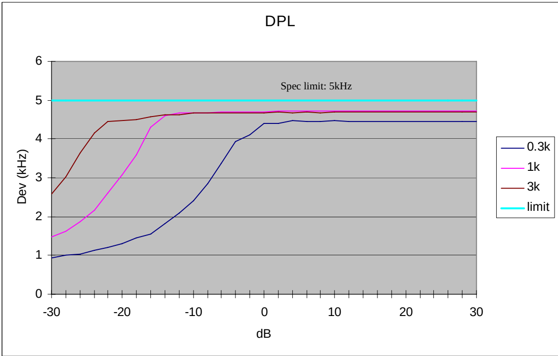
Figure 6D-6: 25 kHz Channel Spacing, 414.025 MHz, Digital Private Line (DPL) Mode
