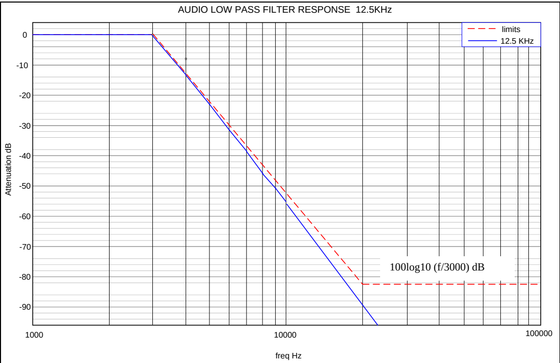
Figure 6C-1: 12.5 kHz Channel Spacing, 414.025 MHz, Transmit Audio Lowpass Filter Response
