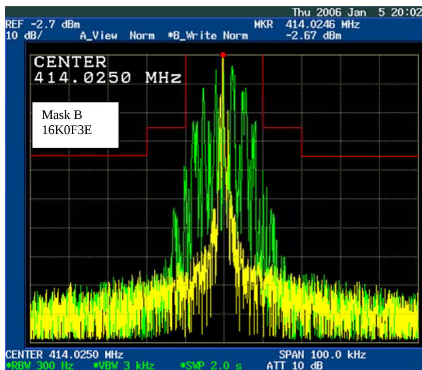
Figure 6E-6: 25 kHz Channel Spacing, 414.025 MHz, 2500 Hz Audio and DPL Tone Modulation, Mask B 16K0F3E
