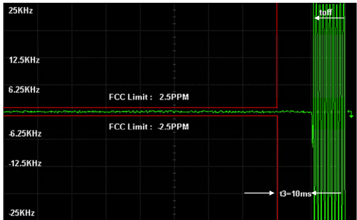
Figure 6I-4: 4 Watts, 25 kHz, 414.025 MHz, De-Key Decay Time
