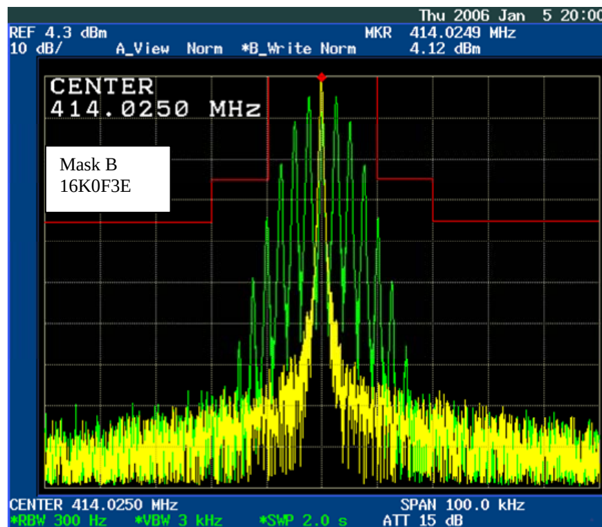
Figure 6E-4: 25 kHz Channel Spacing, 414.025 MHz, 2500 Hz Audio Modulation Only, Mask B 16K0F3E
