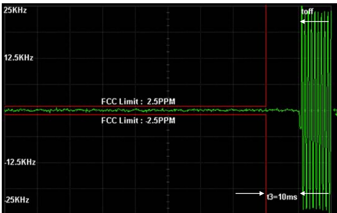
Figure 6I-6: 1 Watt, 12.5 kHz, 414.025 MHz, De-Key Decay Time
