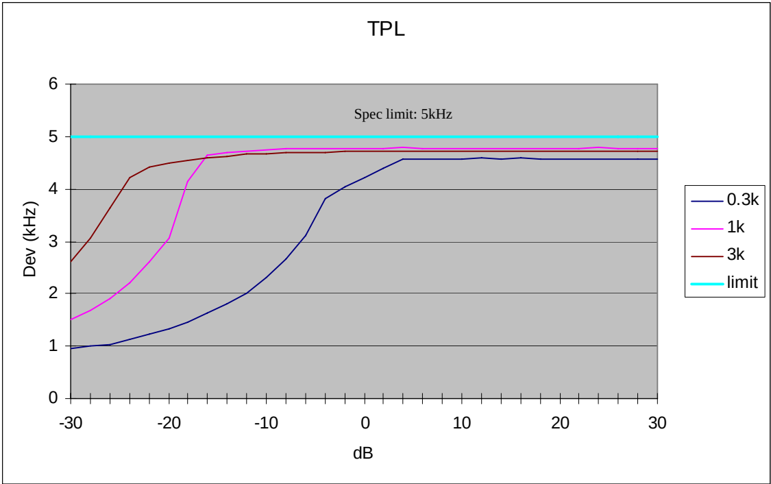
Figure 6D-5: 25 kHz Channel Spacing, 414.025 MHz, Tone Private Line (TPL) Mode
