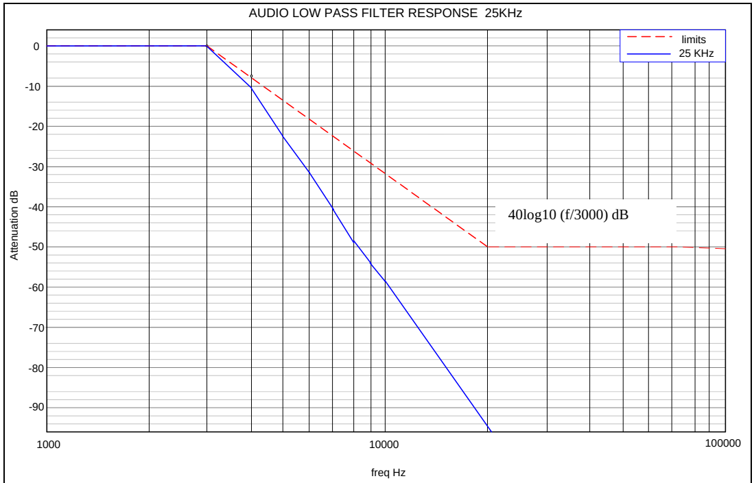
Figure 6C-2: 25 kHz Channel Spacing, 414.025 MHz, Transmit Audio Lowpass Filter Response
