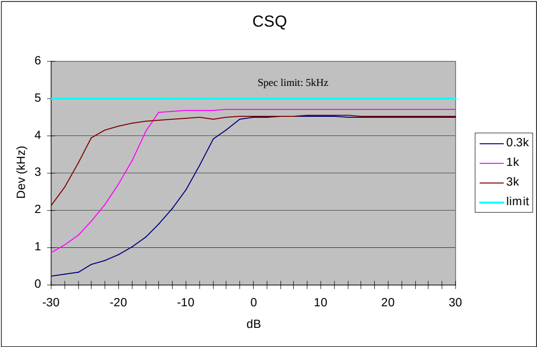
Figure 6D-4: 25 kHz Channel Spacing, 414.025 MHz, Carrier Squelch (CSQ) Mode
