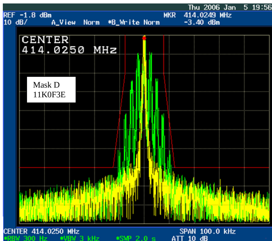
Figure 6E-1: 12.5 kHz Channel Spacing, 414.025 MHz, 2500 Hz Audio Modulation Only, Mask D 11K0F3E
