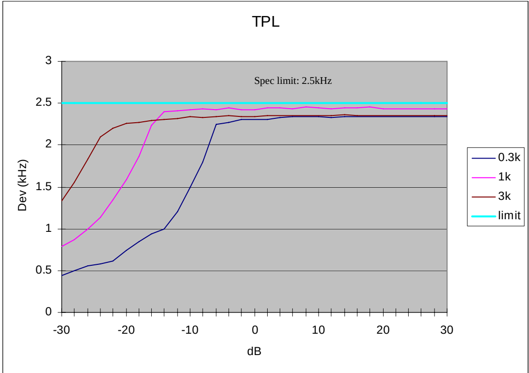
Figure 6D-2: 12.5 kHz Channel Spacing, 414.025 MHz, Tone Private Line (TPL) Mode
