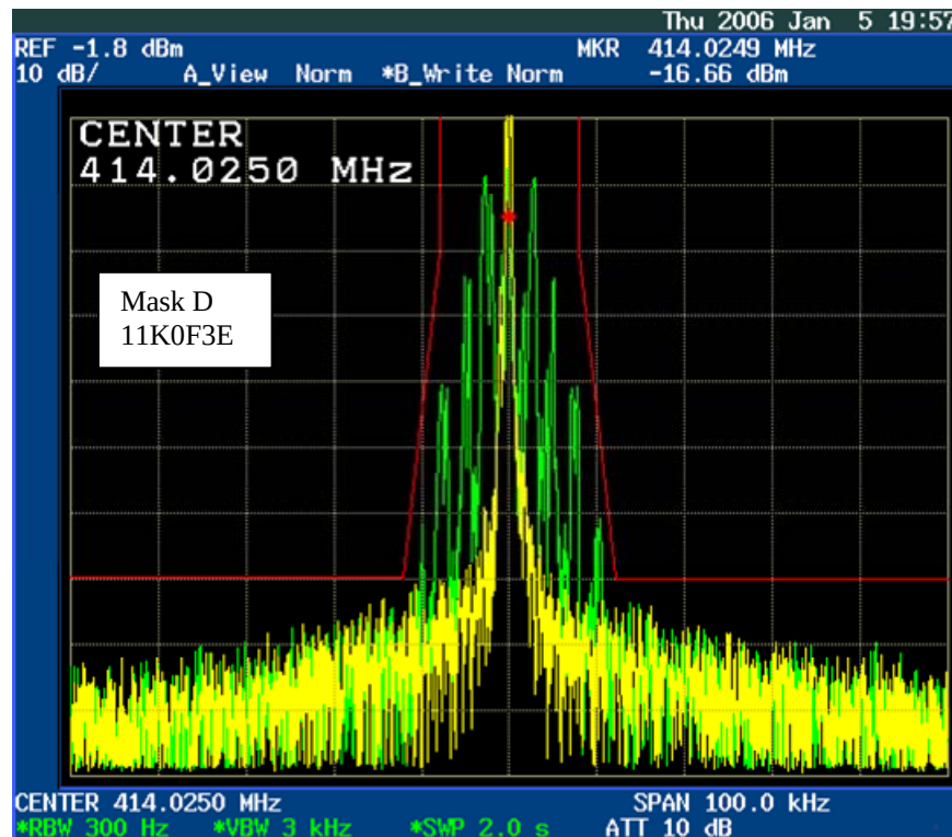
Figure 6E-3: 12.5 kHz Channel Spacing, 414.025 MHz, 2500 Hz Audio and DPL Tone Modulation, Mask D 11K0F3E
