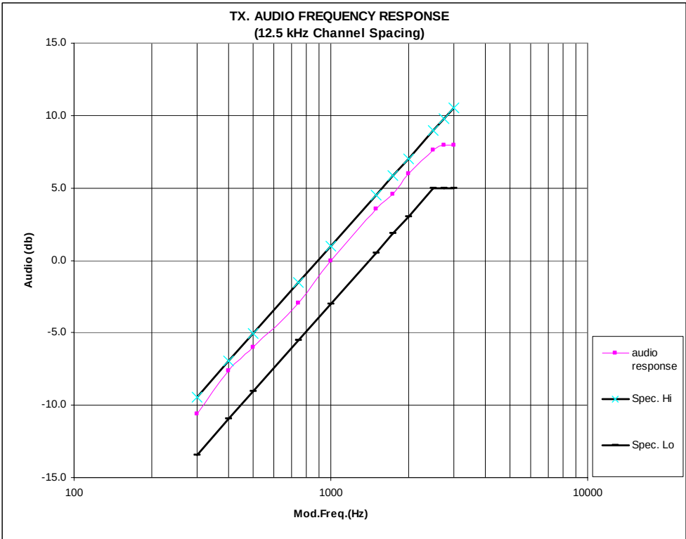
Figure 6B-1: 12.5 kHz Channel Spacing, 414.025 MHz, Transmit Audio Frequency Response
