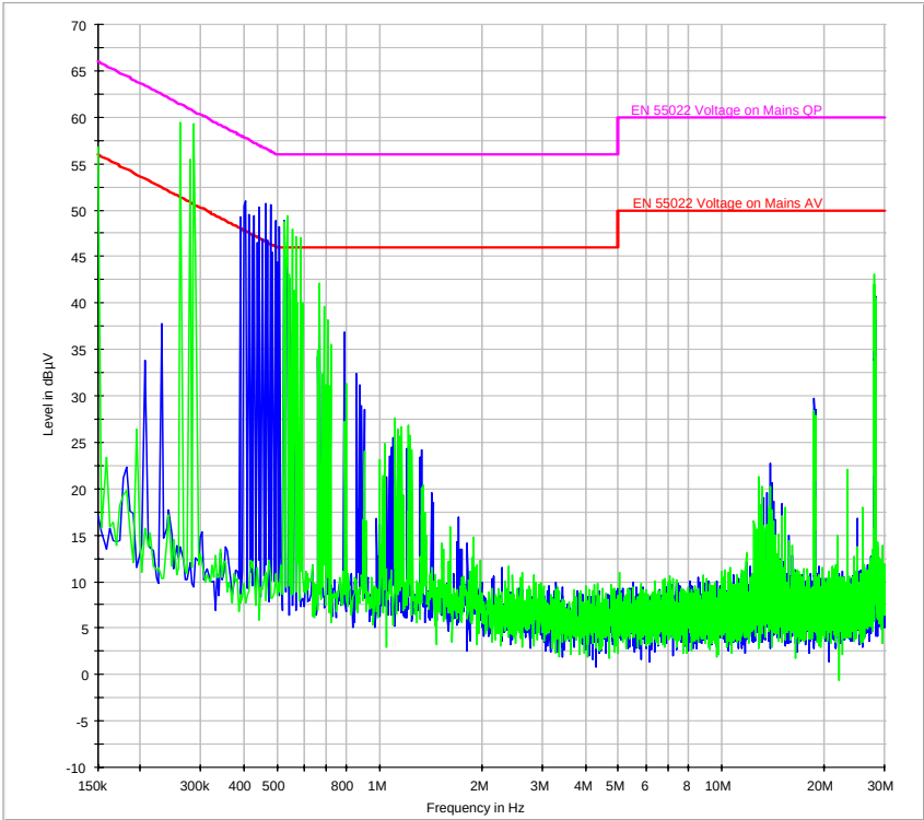
EMI Conducted Scan latest FCC Peak det - 3810 LISN Tx Freq 403.025 MHz Auto Merge Results N (Green) L1 (Blue)
