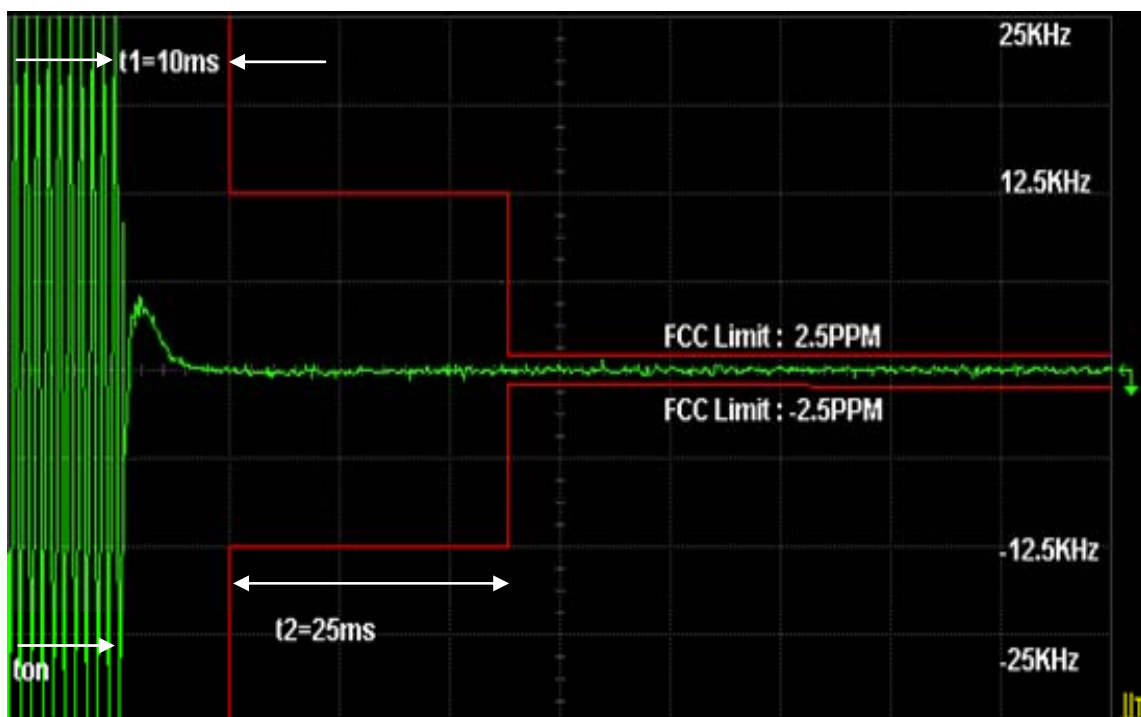
Figure 6I-7: 1 Watt, 25 kHz, 414.025 MHz, Key-Up Attack Time
