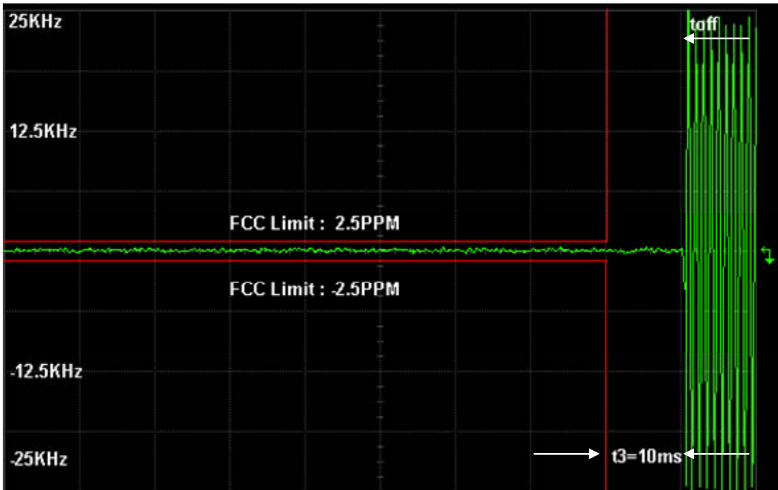
Figure 6I-2: 4 Watts, 12.5 kHz, 414.025 MHz, De-Key Decay Time
