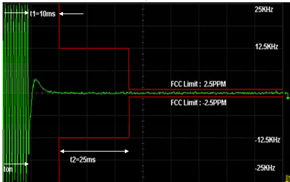
Figure 6I-3: 4 Watts, 25 kHz, 414.025 MHz, Key-Up Attack Time
