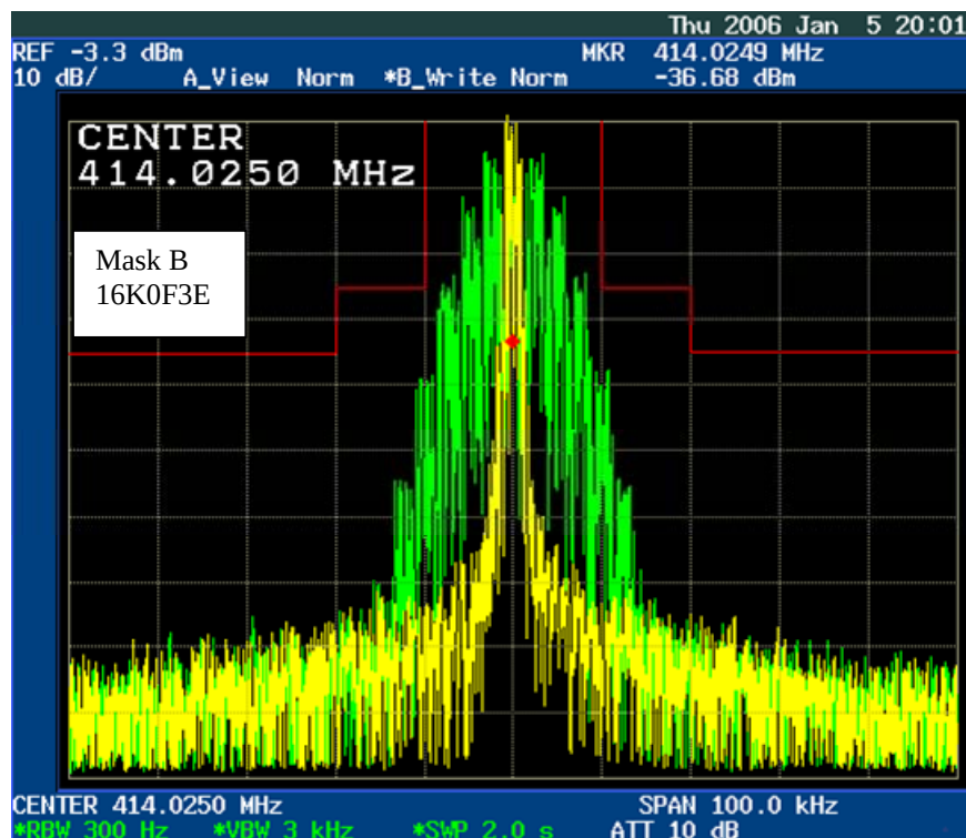
Figure 6E-5: 25 kHz Channel Spacing, 414.025 MHz, 2500 Hz Audio and PL Tone Modulation, Mask B 16K0F3E
