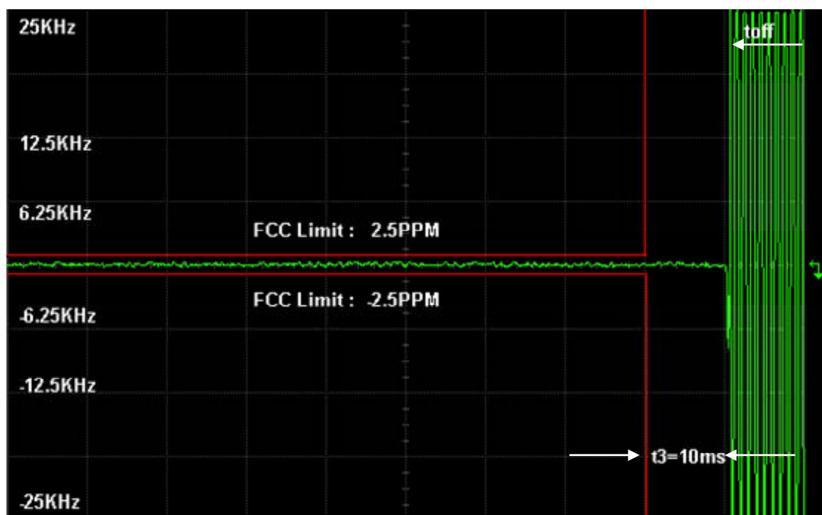
Figure 6I-8: 1 Watt, 25 kHz, 414.025 MHz, De-Key Decay Time
