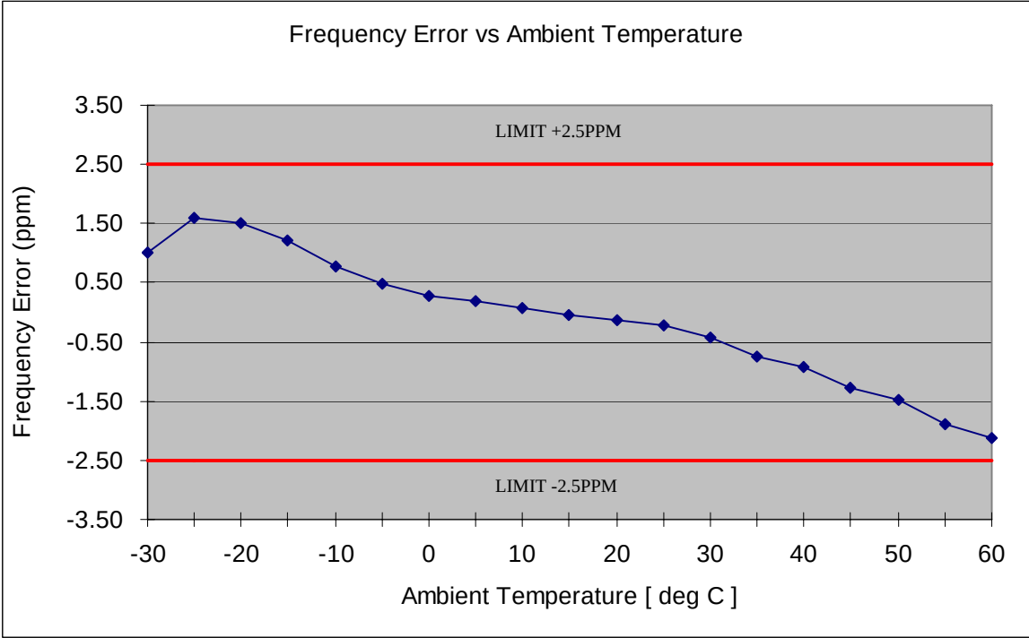
Figure 6H-1: Frequency Stability vs. Temperature
