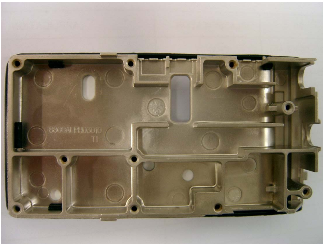
Figure 9-4: Bottom View of chassis.
