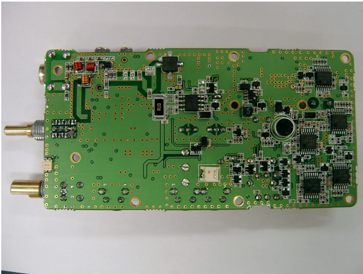
Figure 9-1: Top Side of PCB.
