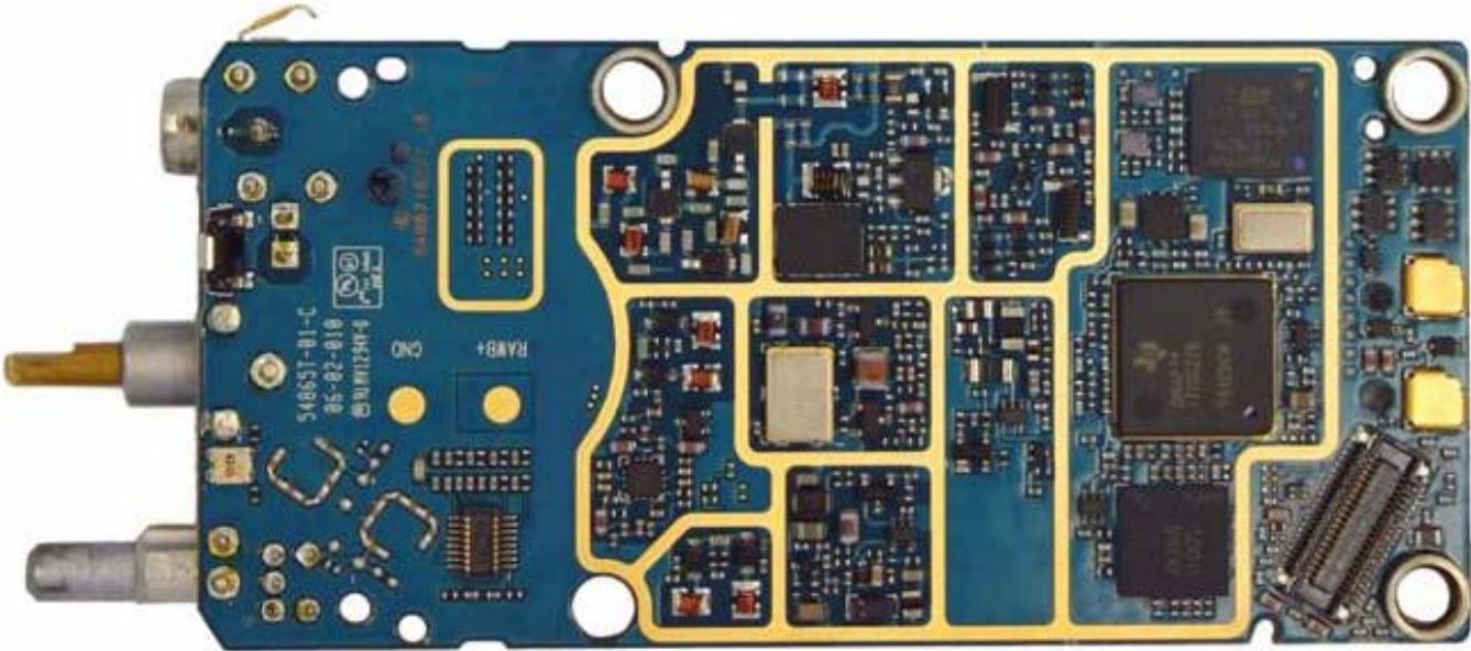
FIGURE 3-8: MOTOTRBO BOARD TOP VIEW.
