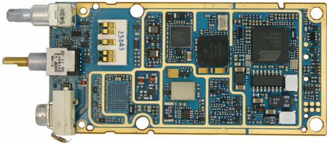
FIGURE 3-6: MOTOTRBO BOTTOM VIEW BOARD WITHOUT GPS.
