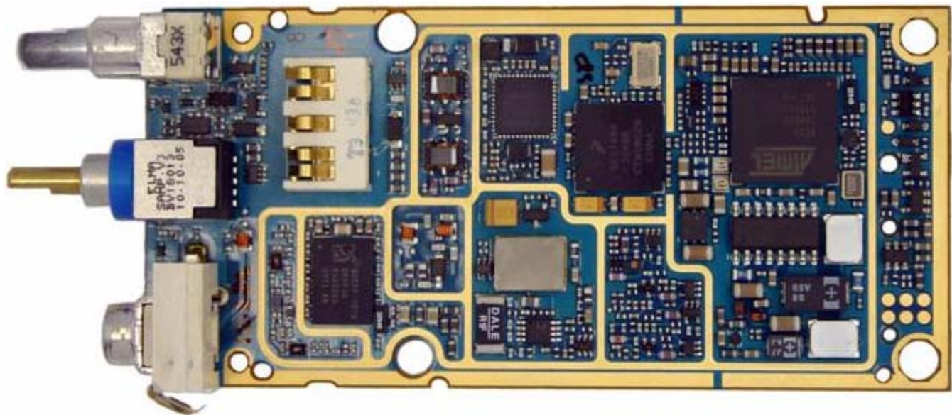
FIGURE 3-7: MOTOTRBO BOTTOM VIEW BOARD WITH GPS.
