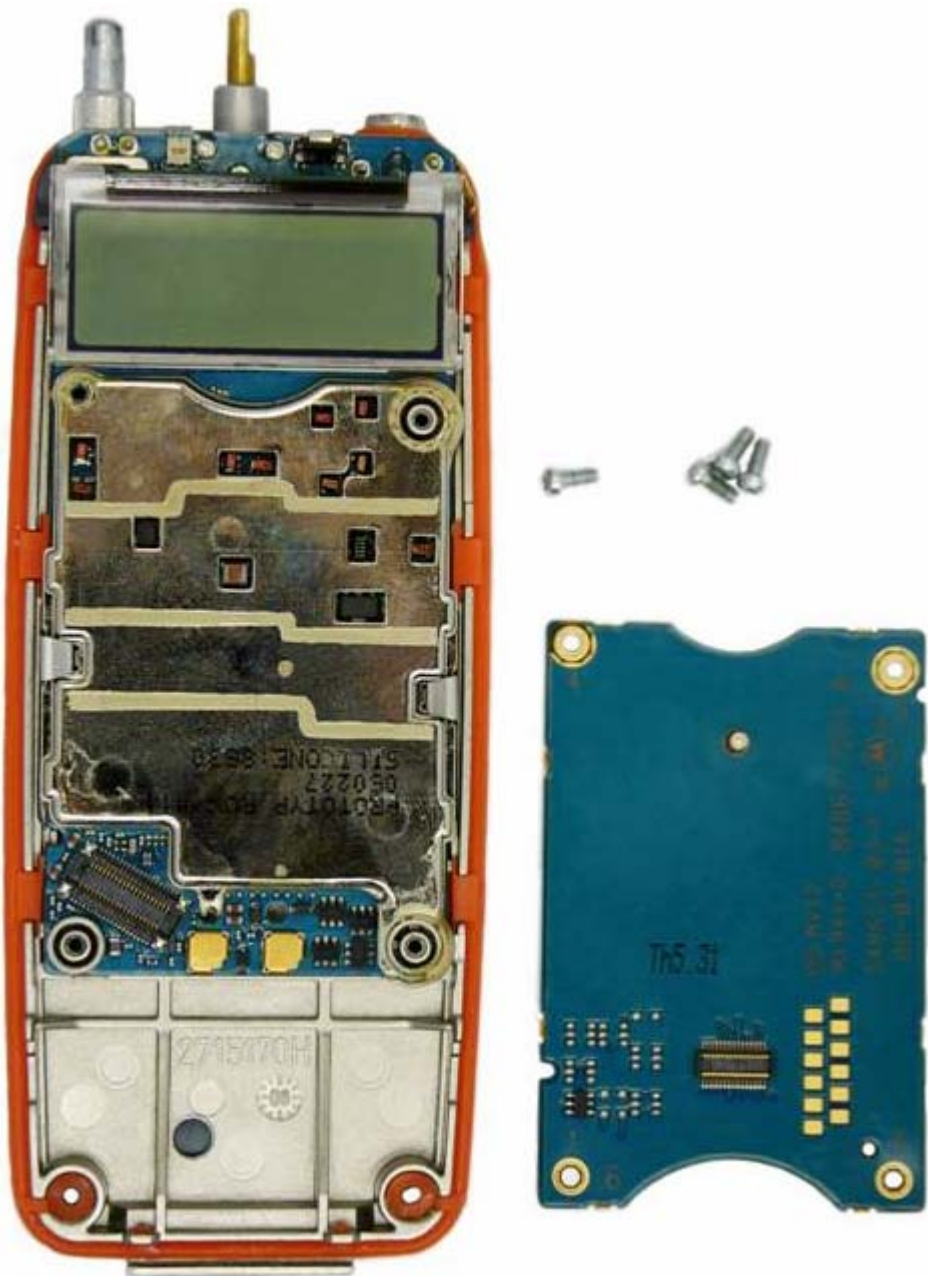
FIGURE 3- 2: MOTOTRBO WITH OPTION BOARD.
