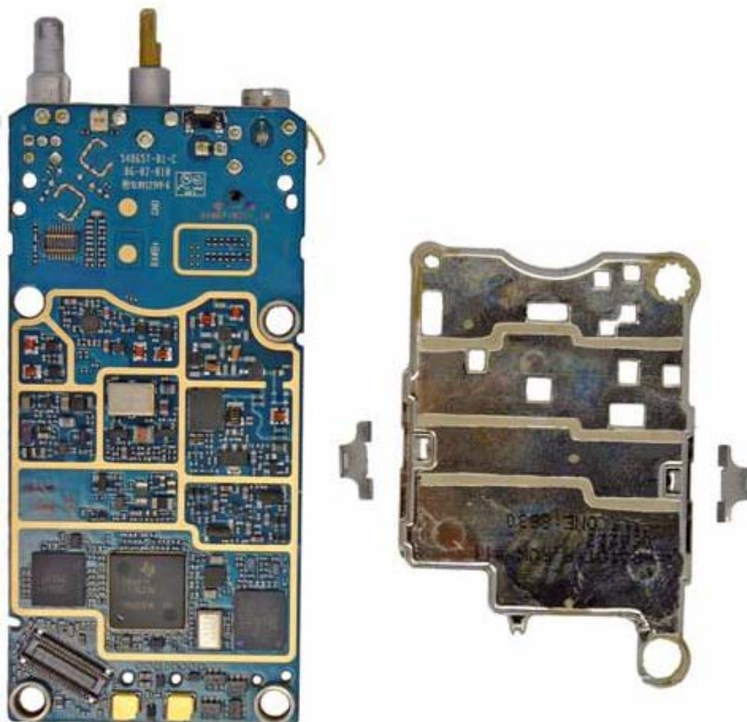
FIGURE 3-5: MOTOTRBO BOARD WITH CLIP-SHIELD DETACHED.
