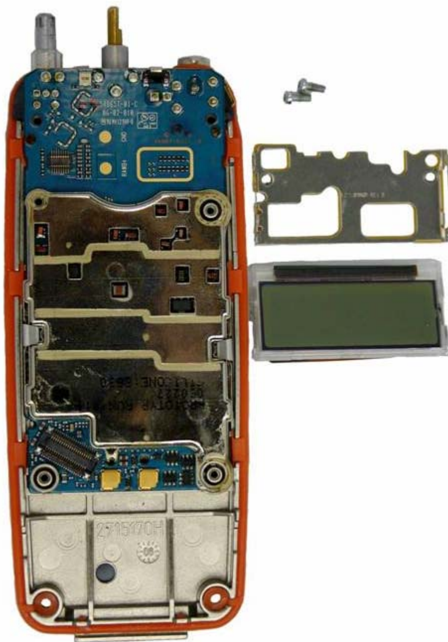
FIGURE 3-3: MOTOTRBO WITH LCD AND METAL BRACKET DETACHED.
