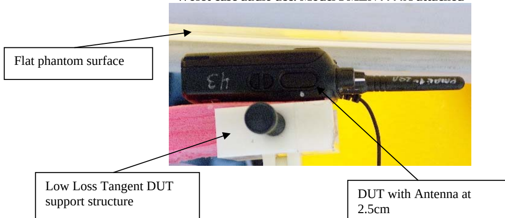
Figure 1: Highest S.A.R. Test Position (Body) DUT Back w/ antenna separated 2.5cm from the phantom. Worst case audio acc. Model PMLN4444A attached
